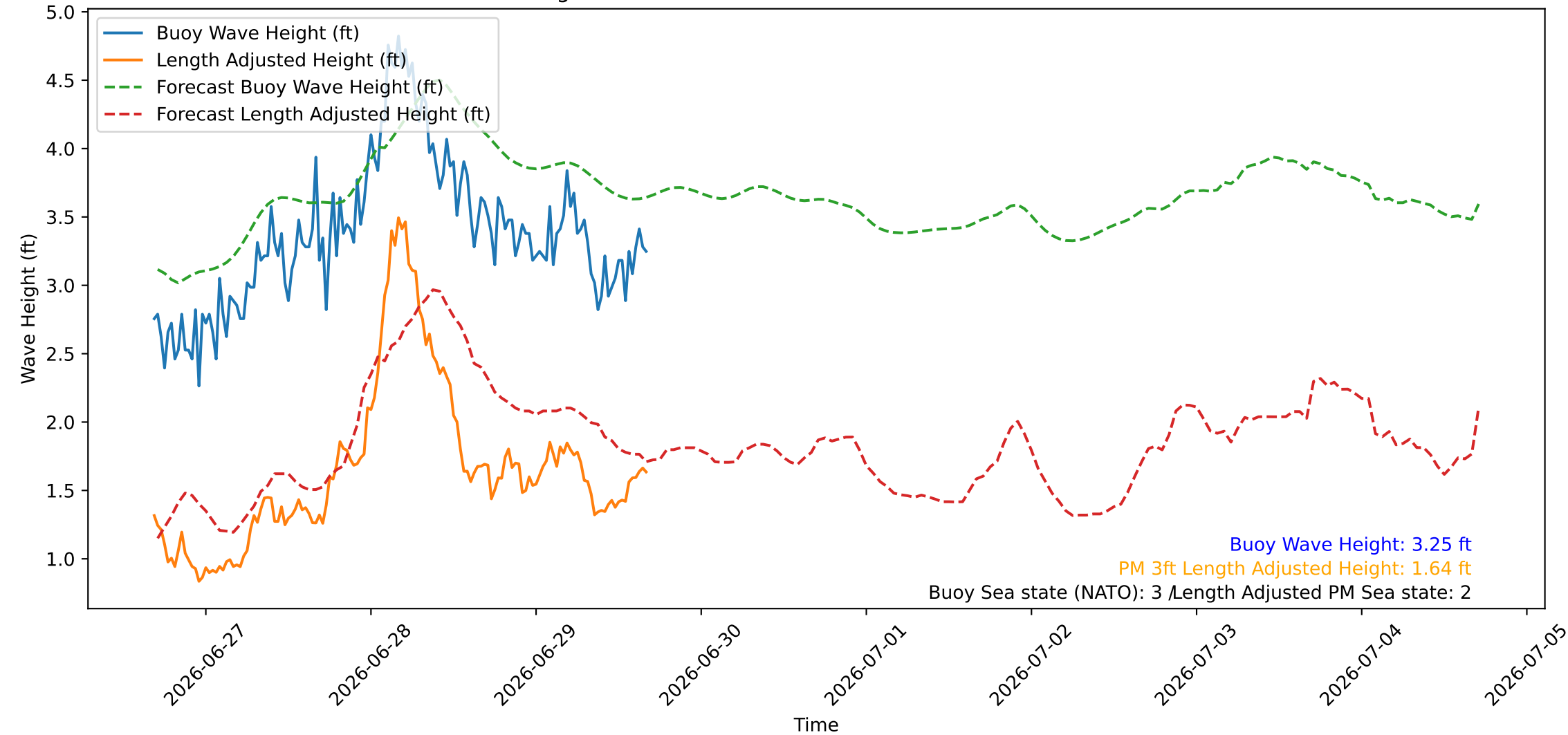
Wave Heights over Time for Green Beach at 2026-06-29 16:41:08
