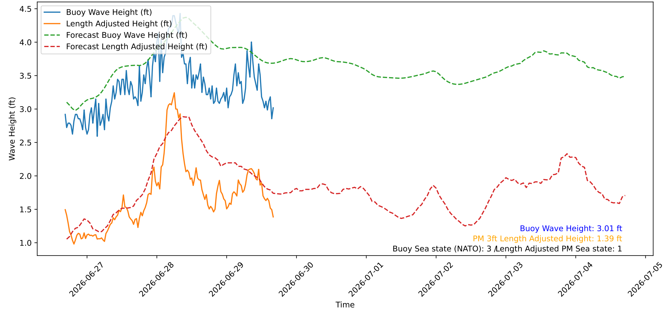
Wave Heights over Time for Oceanside Harbor at 2026-06-29 16:40:26
