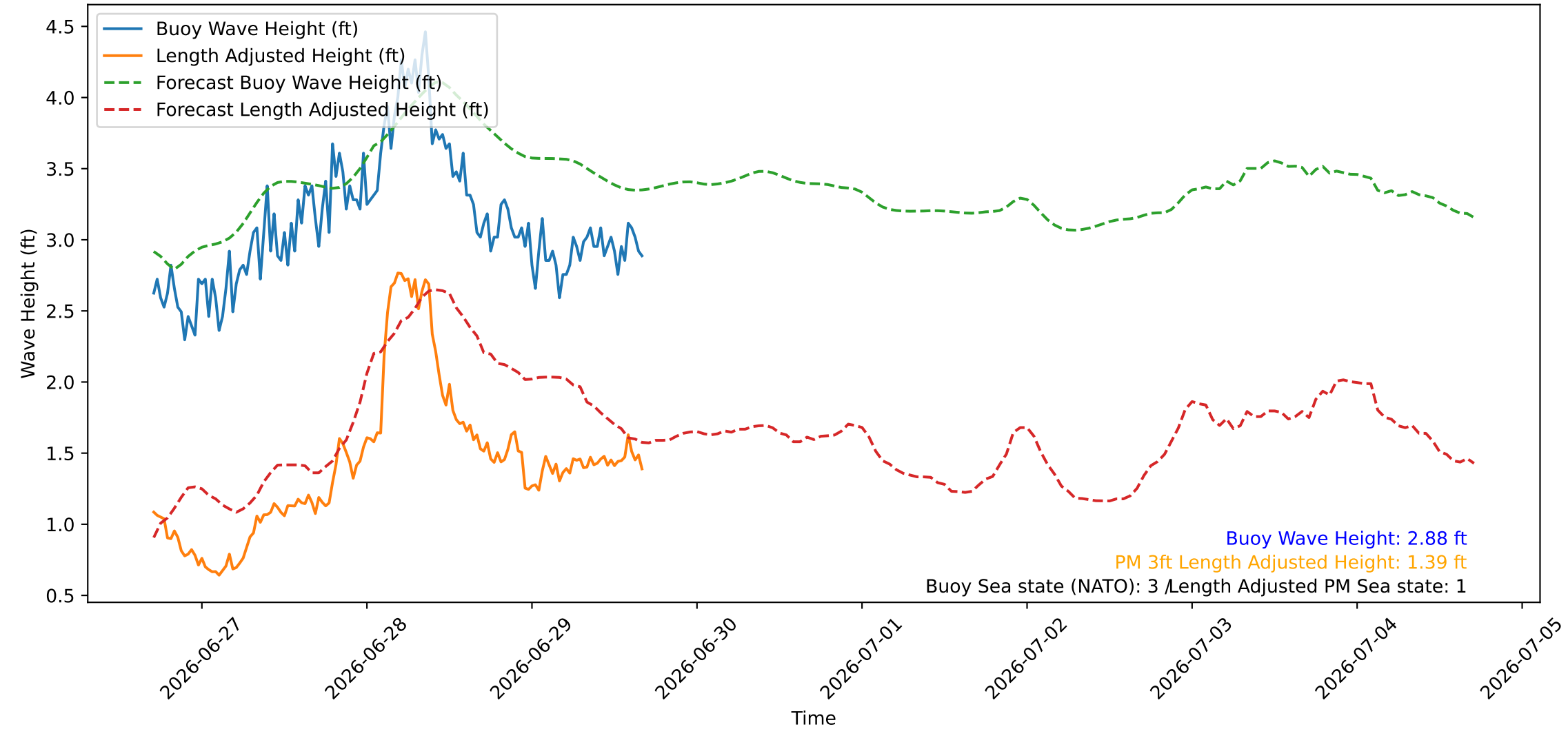
Wave Heights over Time for Red Beach at 2026-06-29 16:40:45
