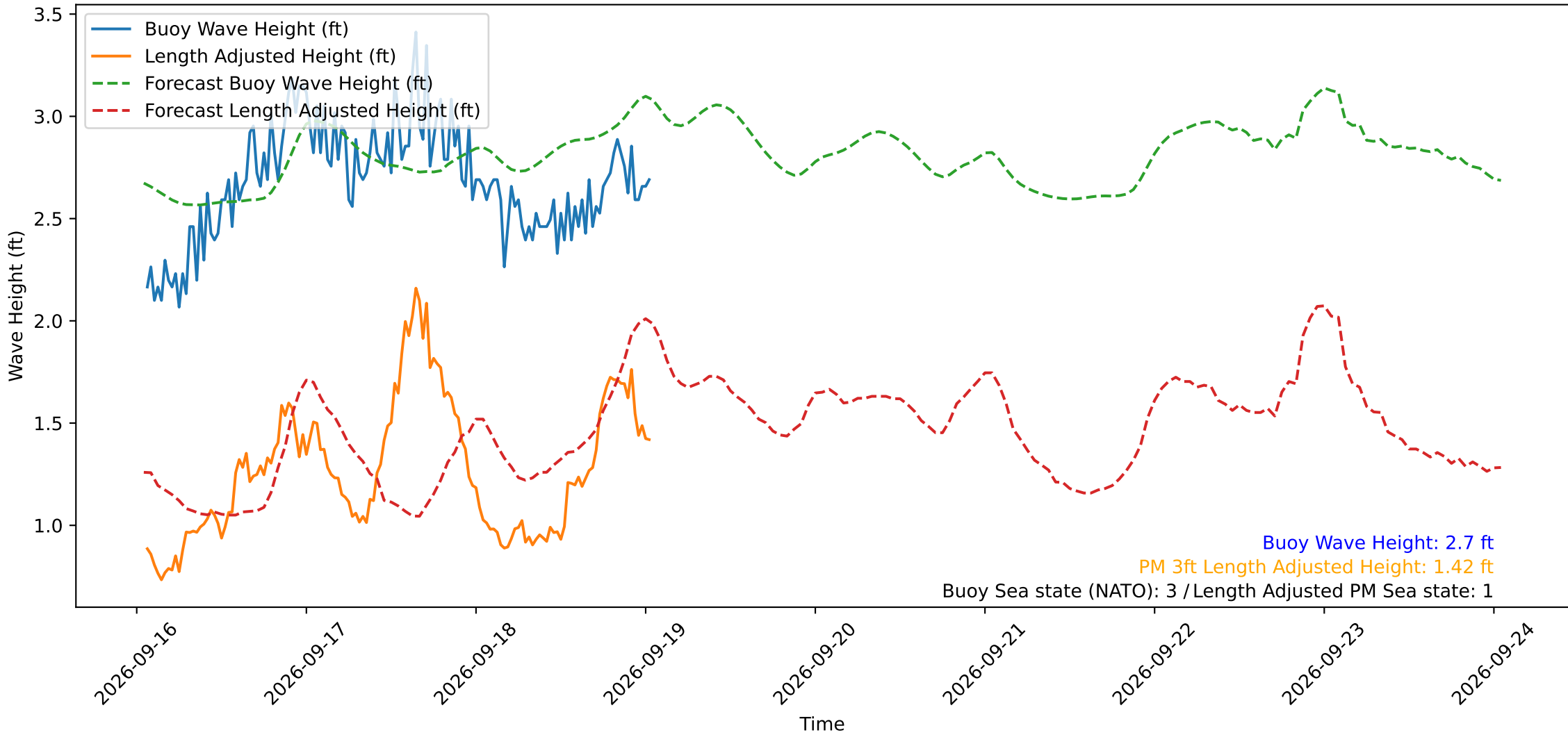
Wave Heights over Time for Red Beach at 2026-09-19 01:20:50
