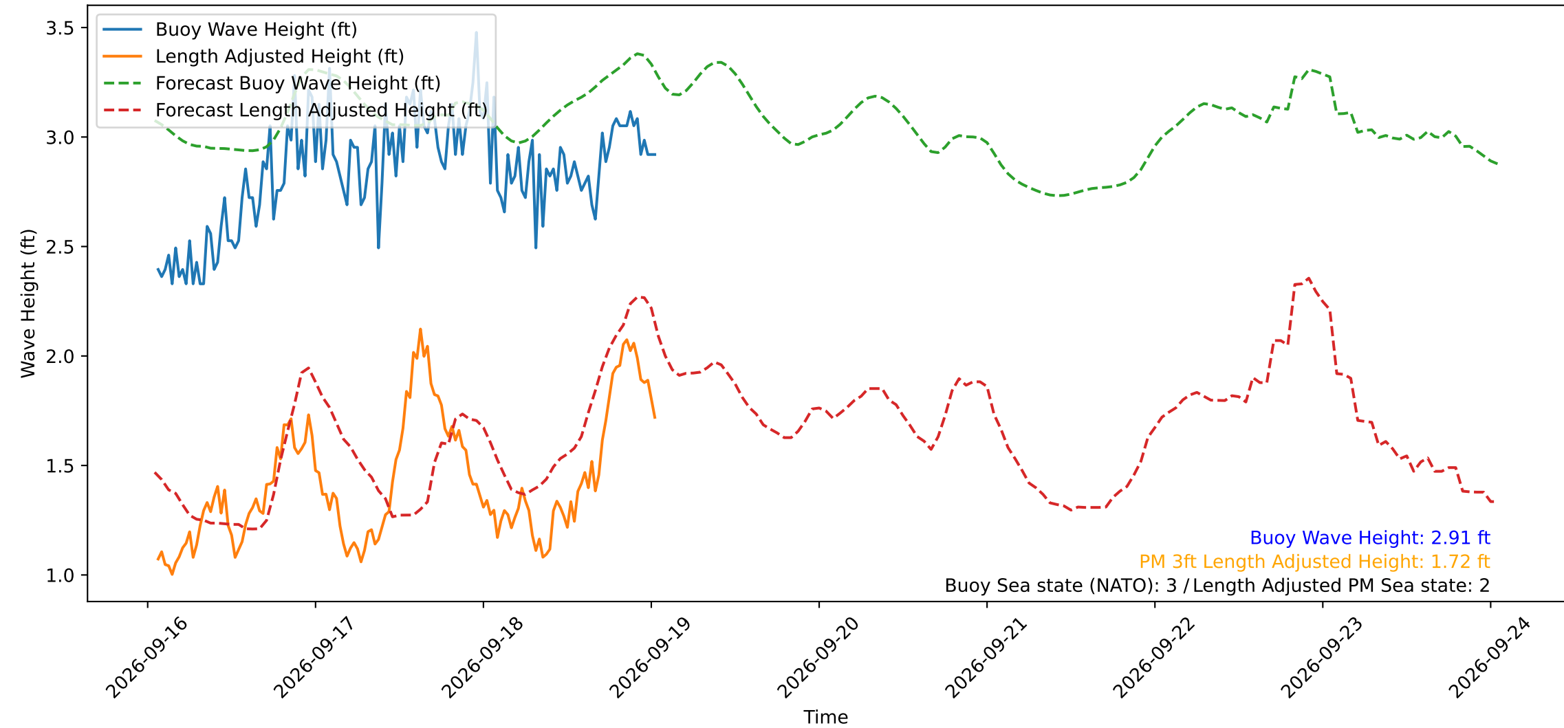
Wave Heights over Time for Green Beach at 2026-09-19 01:21:14
