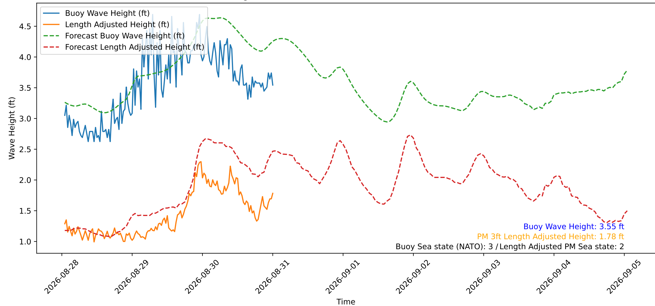
Wave Heights over Time for Red Beach at 2026-08-31 00:40:49
