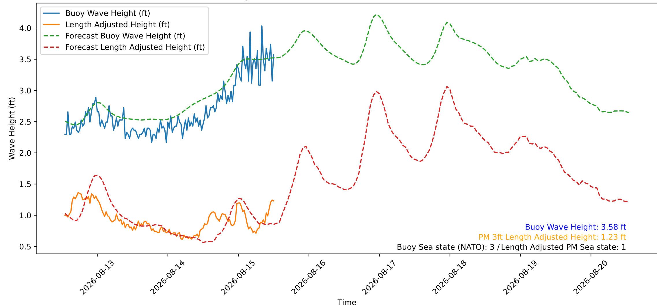
Wave Heights over Time for Red Beach at 2026-08-15 12:40:45
