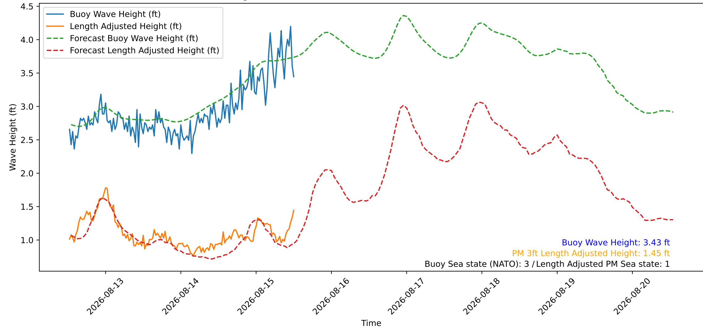
Wave Heights over Time for Oceanside Harbor at 2026-08-15 12:40:26
