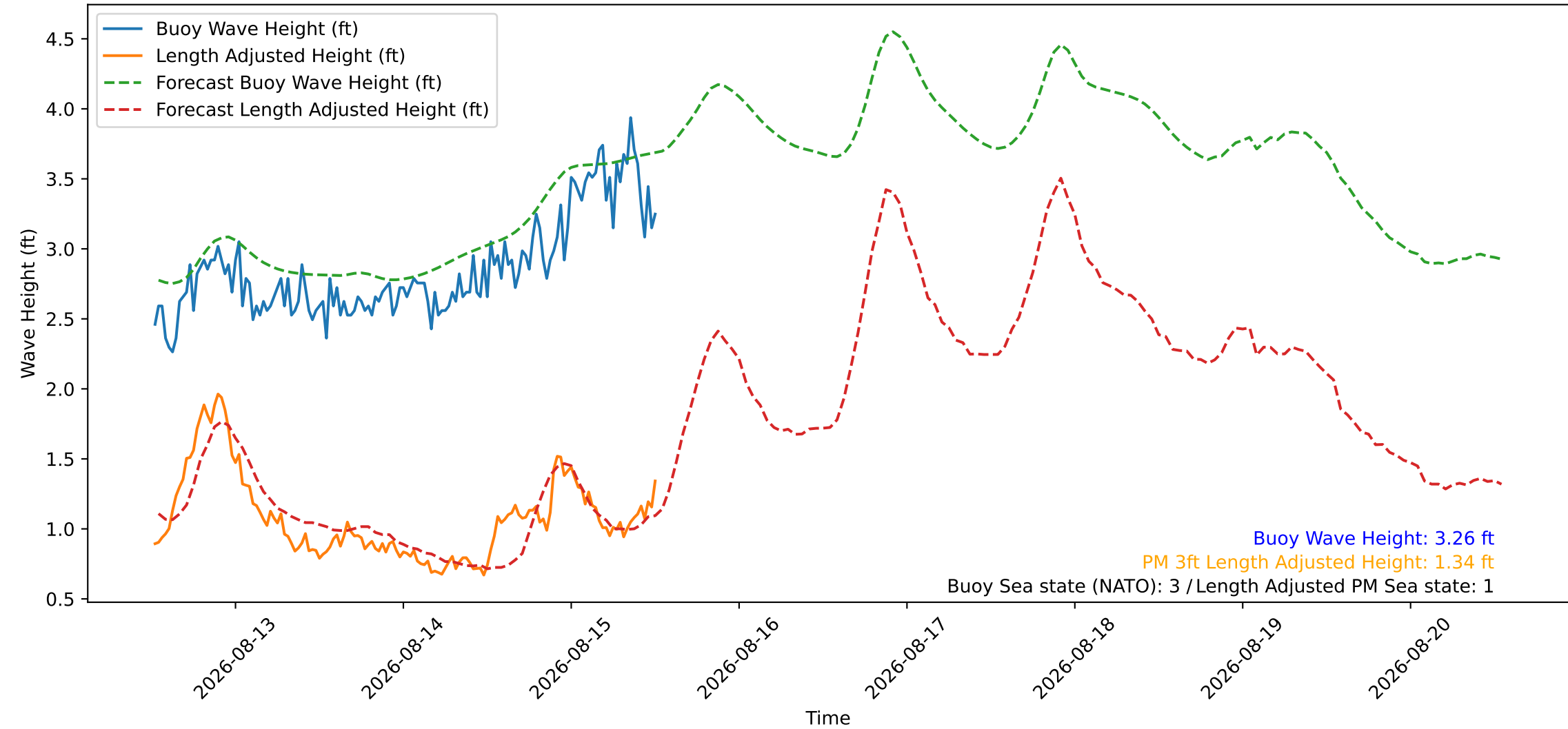
Wave Heights over Time for Green Beach at 2026-08-15 12:41:08
