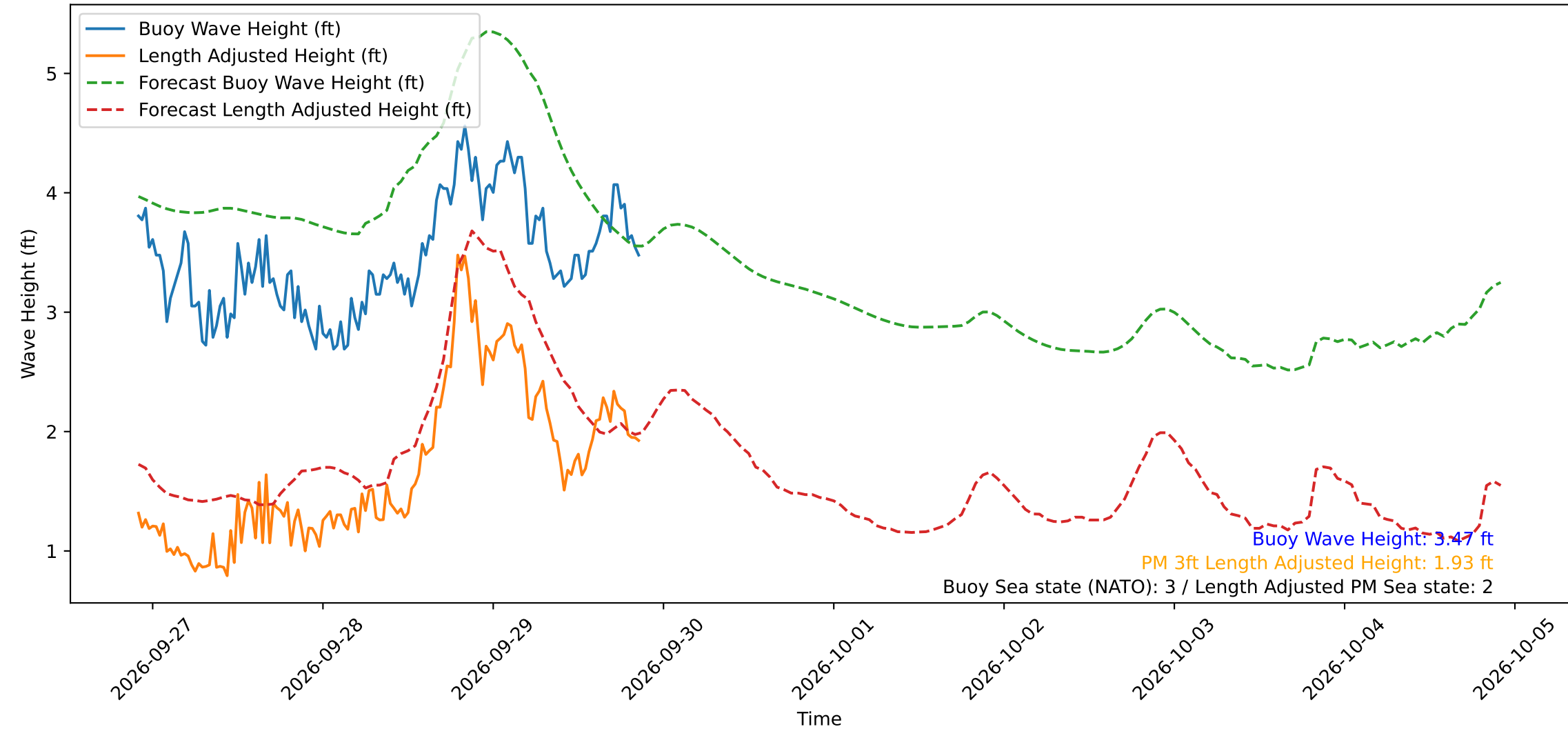
Wave Heights over Time for Green Beach at 2026-09-29 21:31:13
