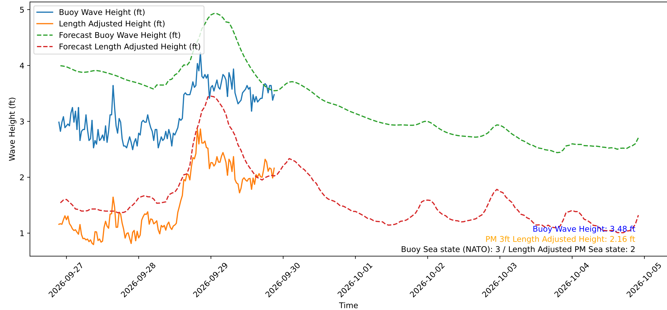
Wave Heights over Time for Oceanside Harbor at 2026-09-29 21:30:30
