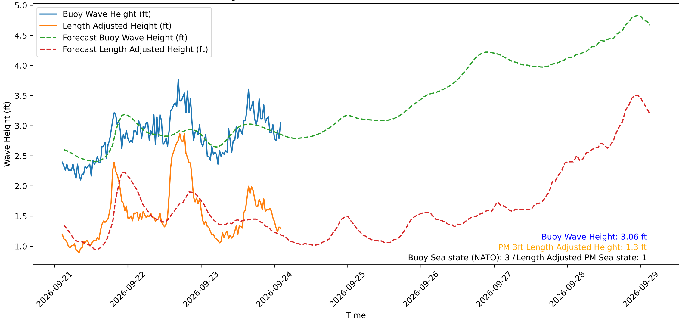
Wave Heights over Time for Oceanside Harbor at 2026-09-24 02:40:29
