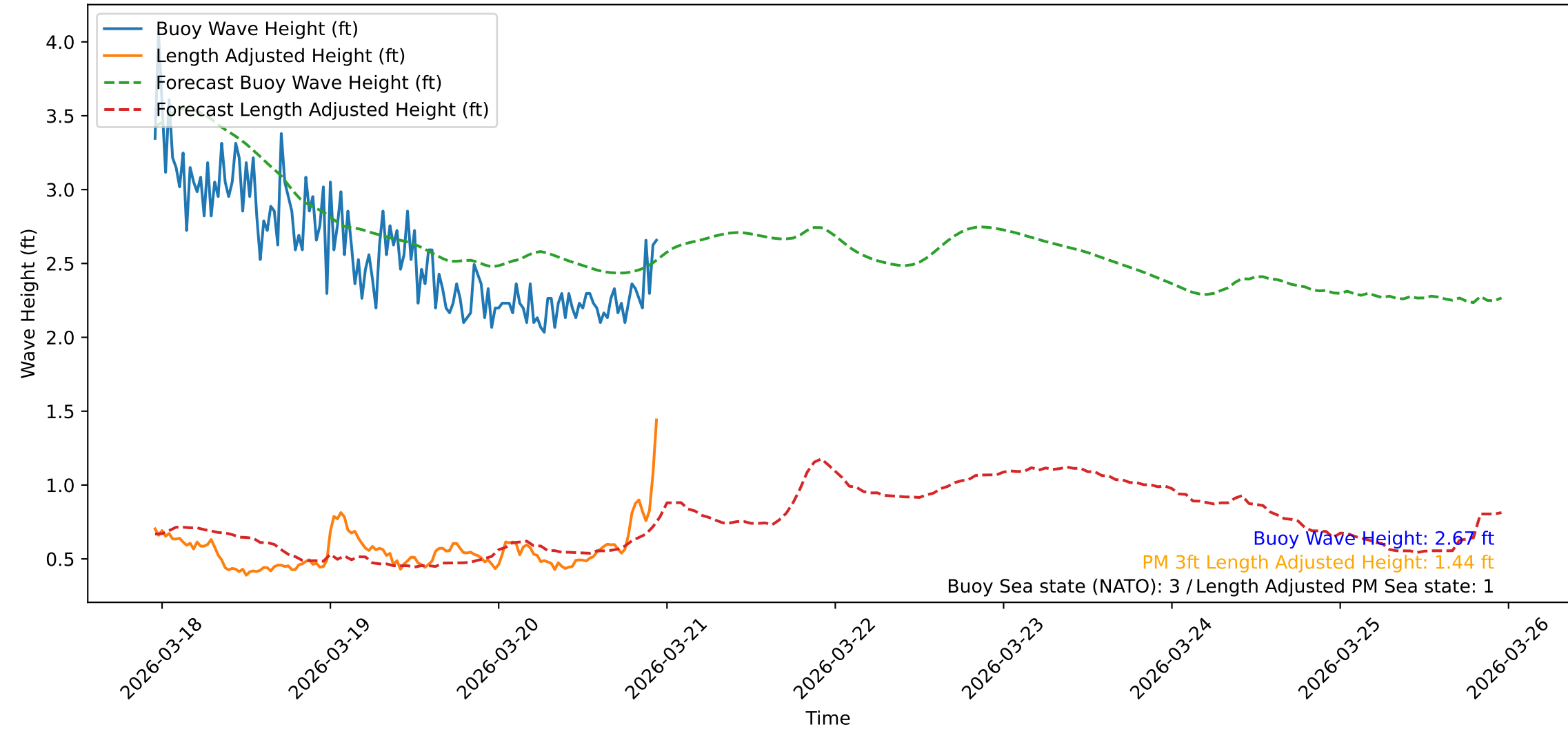
Wave Heights over Time for Green Beach at 2026-03-20 23:11:11
