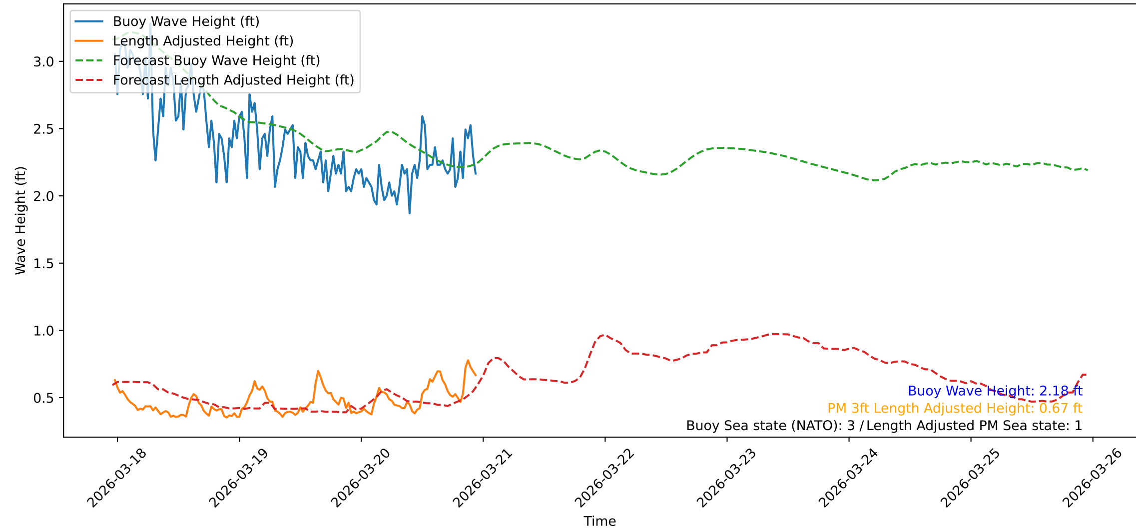
Wave Heights over Time for Red Beach at 2026-03-20 23:10:49
