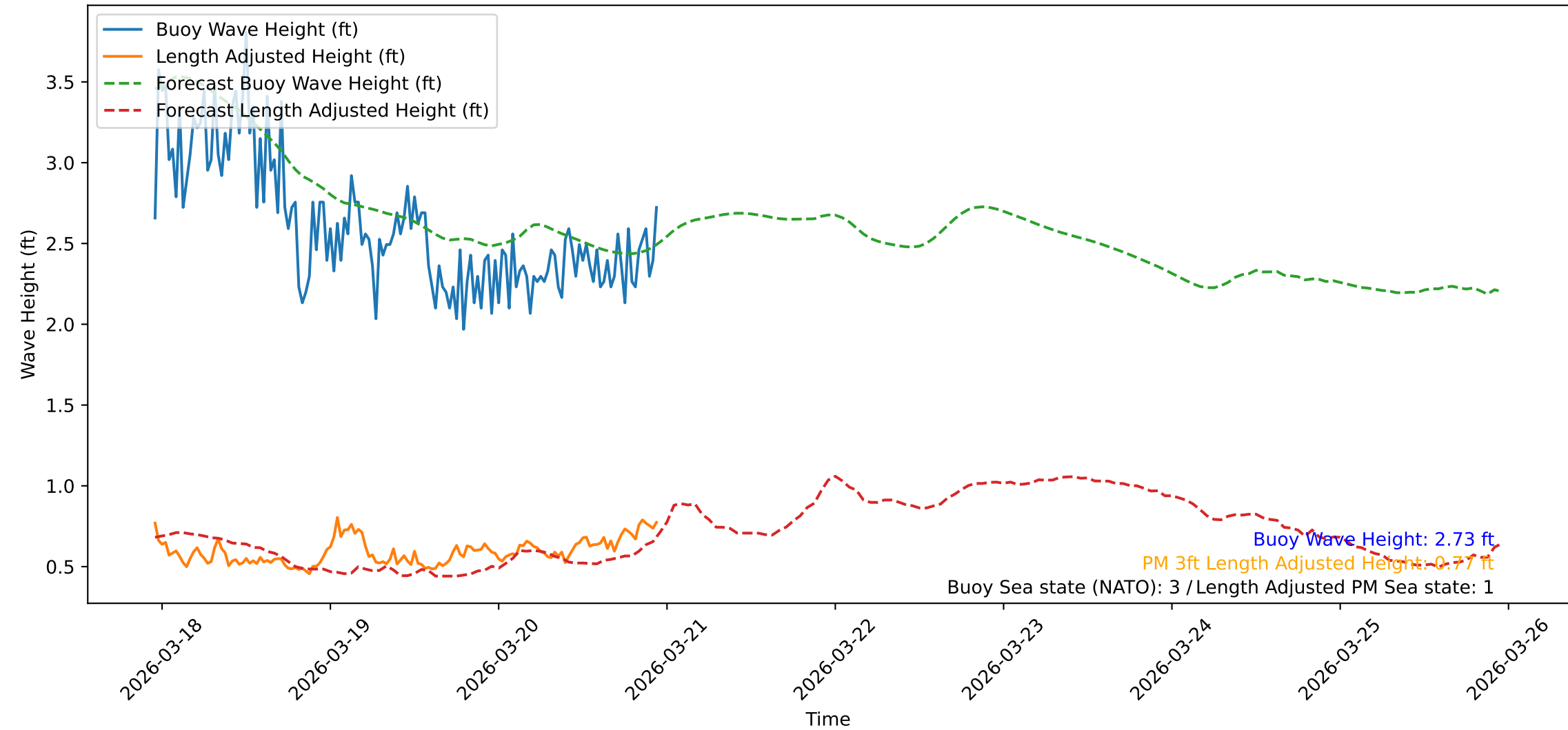
Wave Heights over Time for Oceanside Harbor at 2026-03-20 23:10:32
