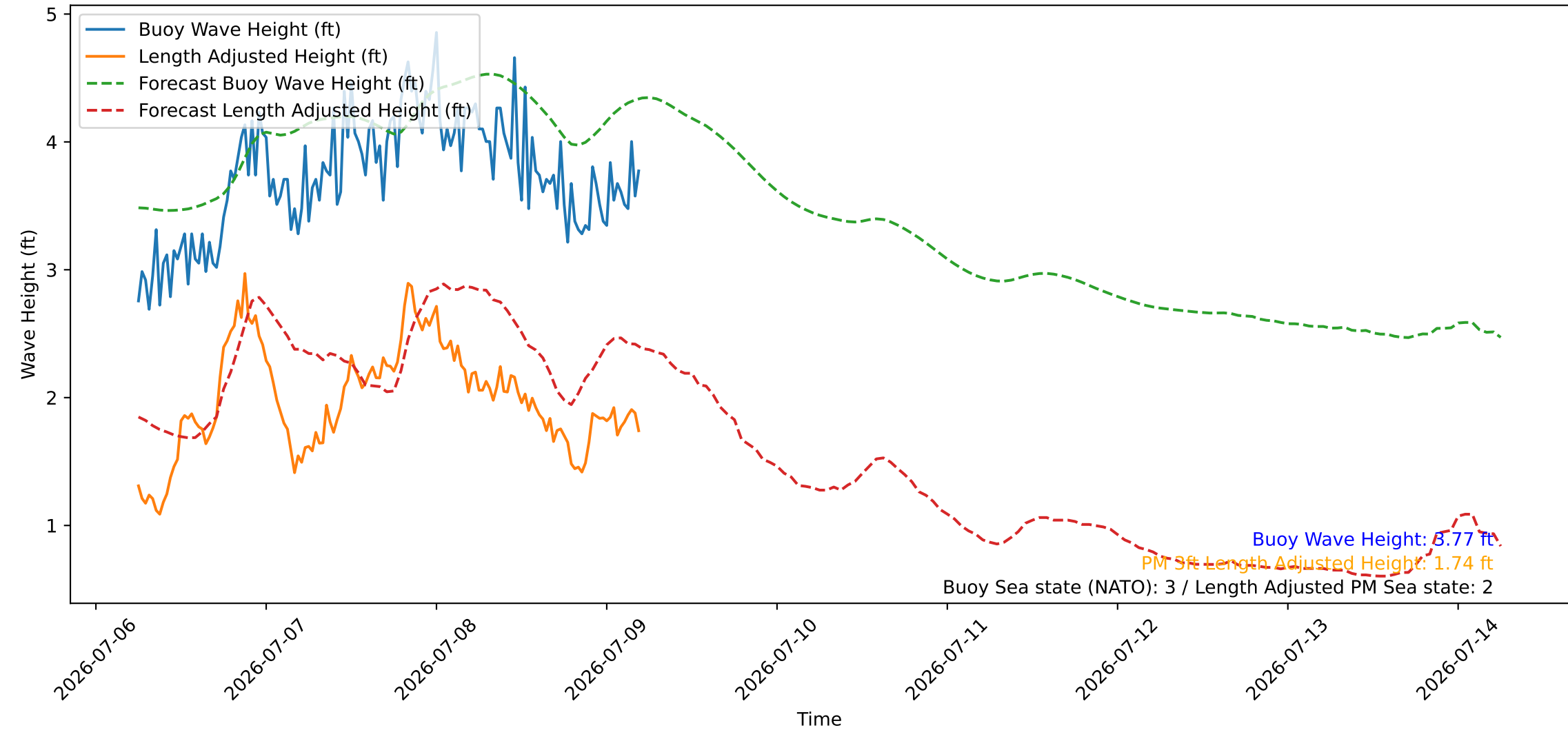
Wave Heights over Time for Red Beach at 2026-07-09 05:30:46
