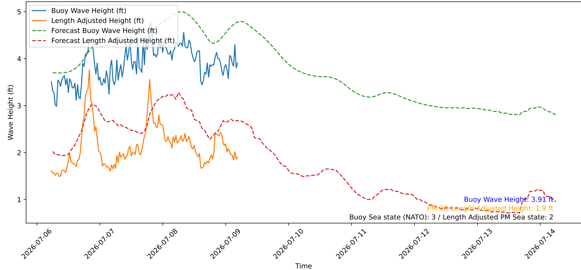
Wave Heights over Time for Green Beach at 2026-07-09 05:31:08
