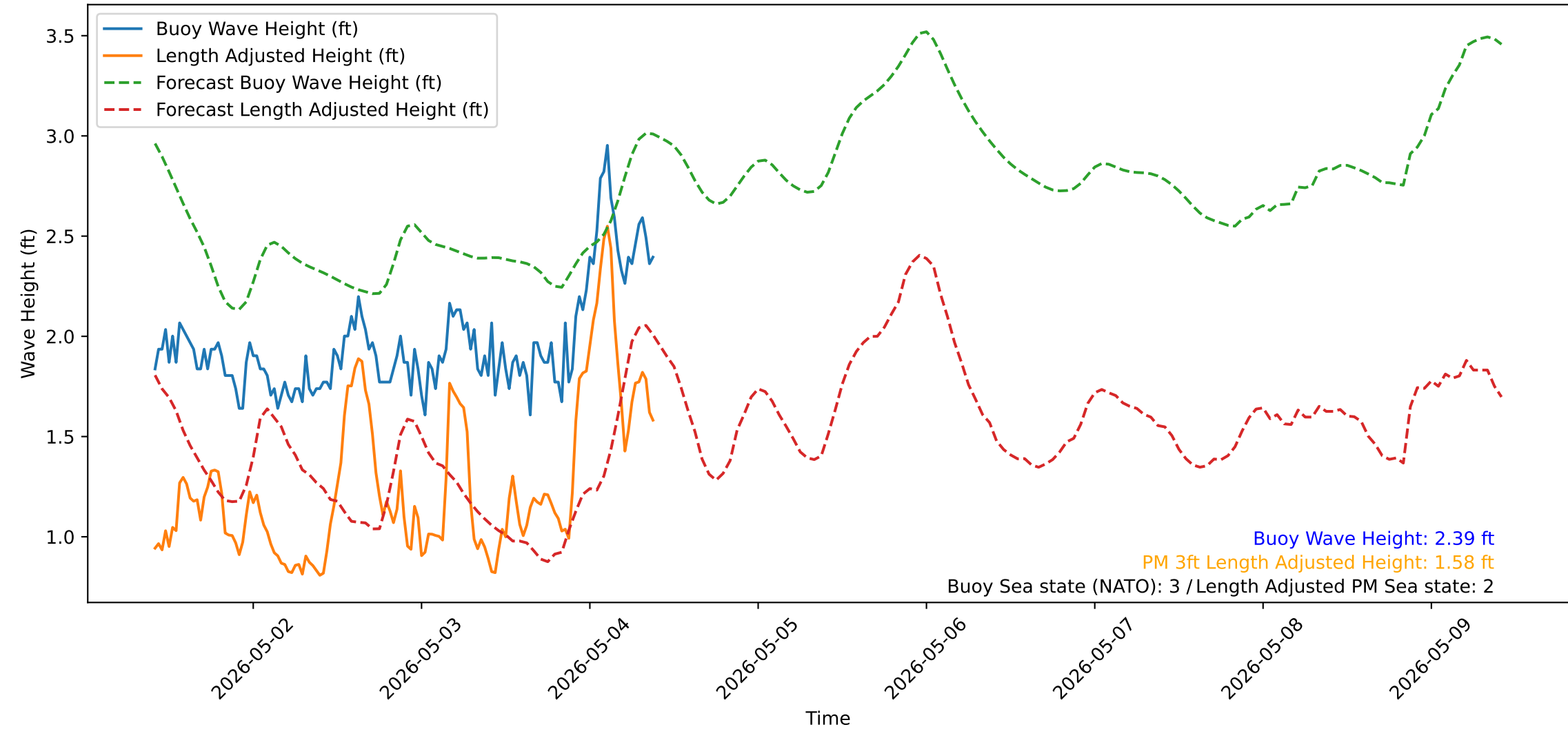
Wave Heights over Time for Red Beach at 2026-05-04 09:40:50
