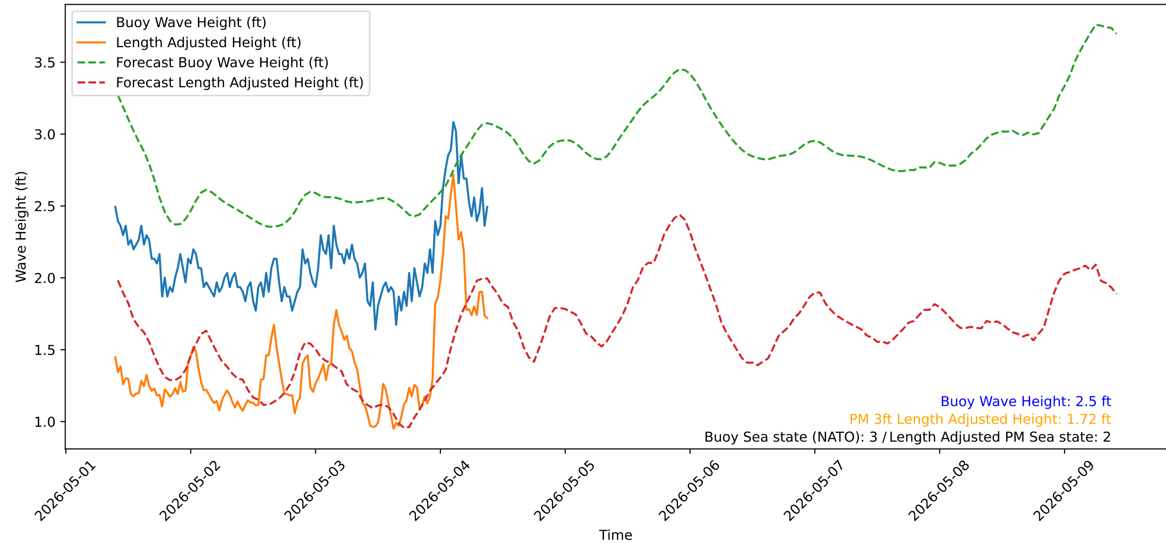
Wave Heights over Time for Oceanside Harbor at 2026-05-04 09:40:31
