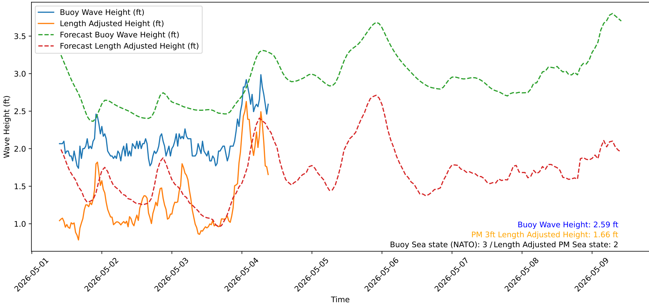
Wave Heights over Time for Green Beach at 2026-05-04 09:41:13
