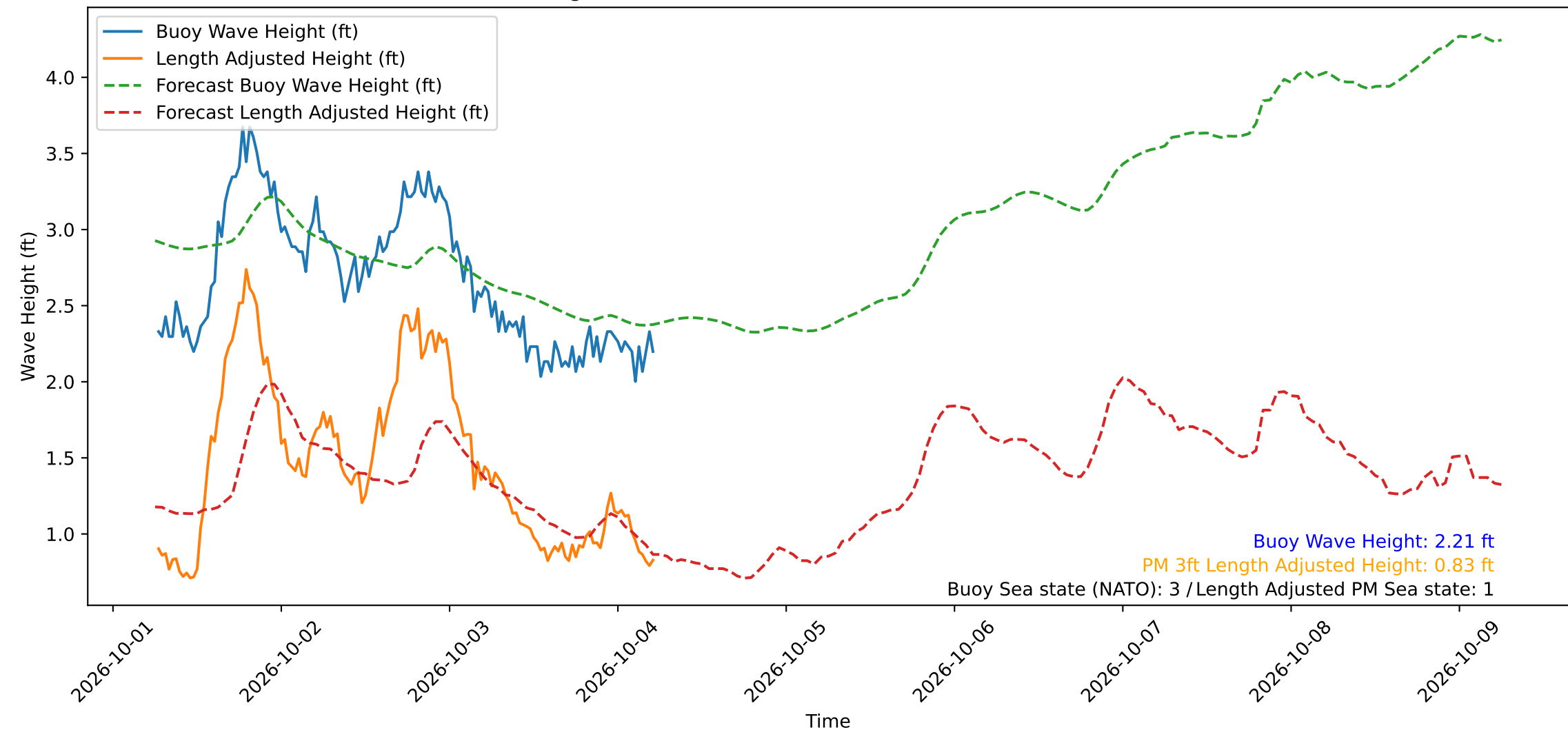
Wave Heights over Time for Green Beach at 2026-10-04 06:01:11
