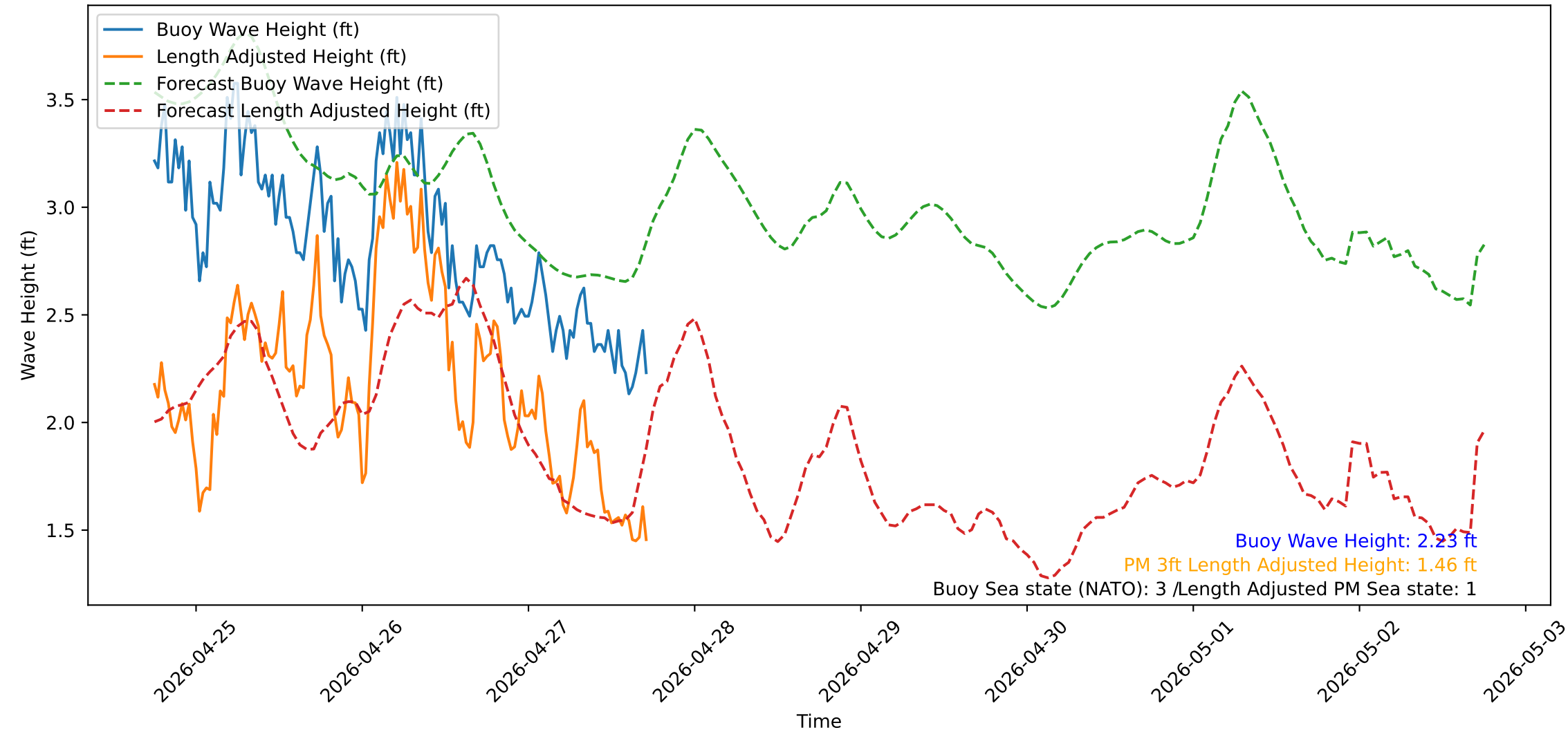
Wave Heights over Time for Green Beach at 2026-04-27 18:01:12
