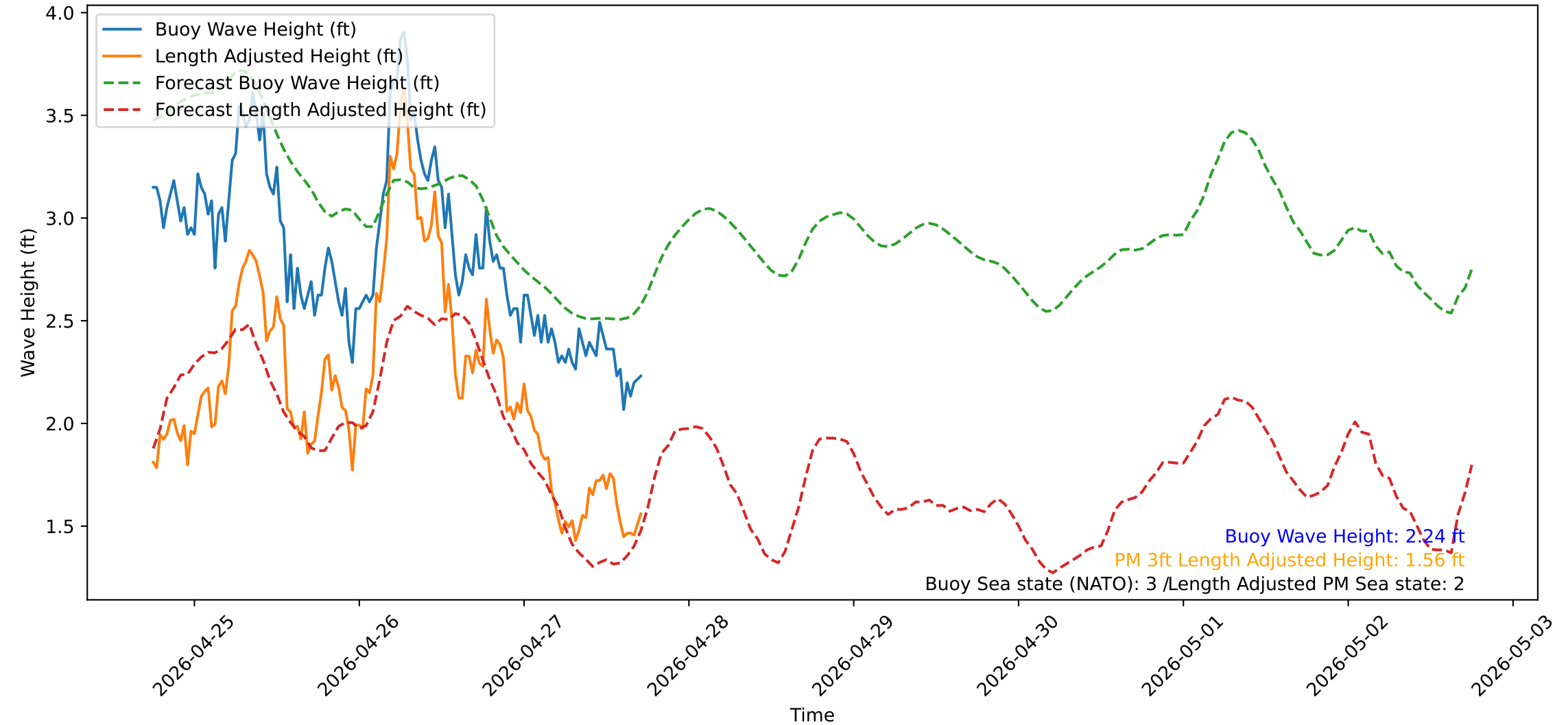
Wave Heights over Time for Oceanside Harbor at 2026-04-27 18:00:31
