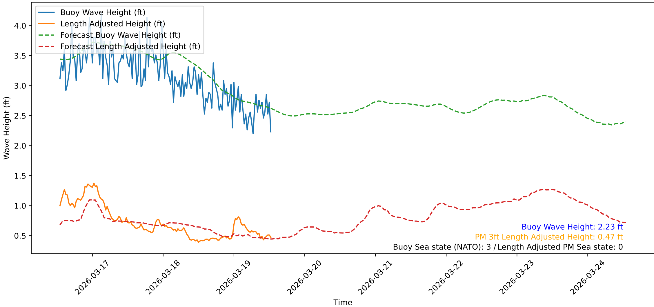
Wave Heights over Time for Green Beach at 2026-03-19 13:11:10
