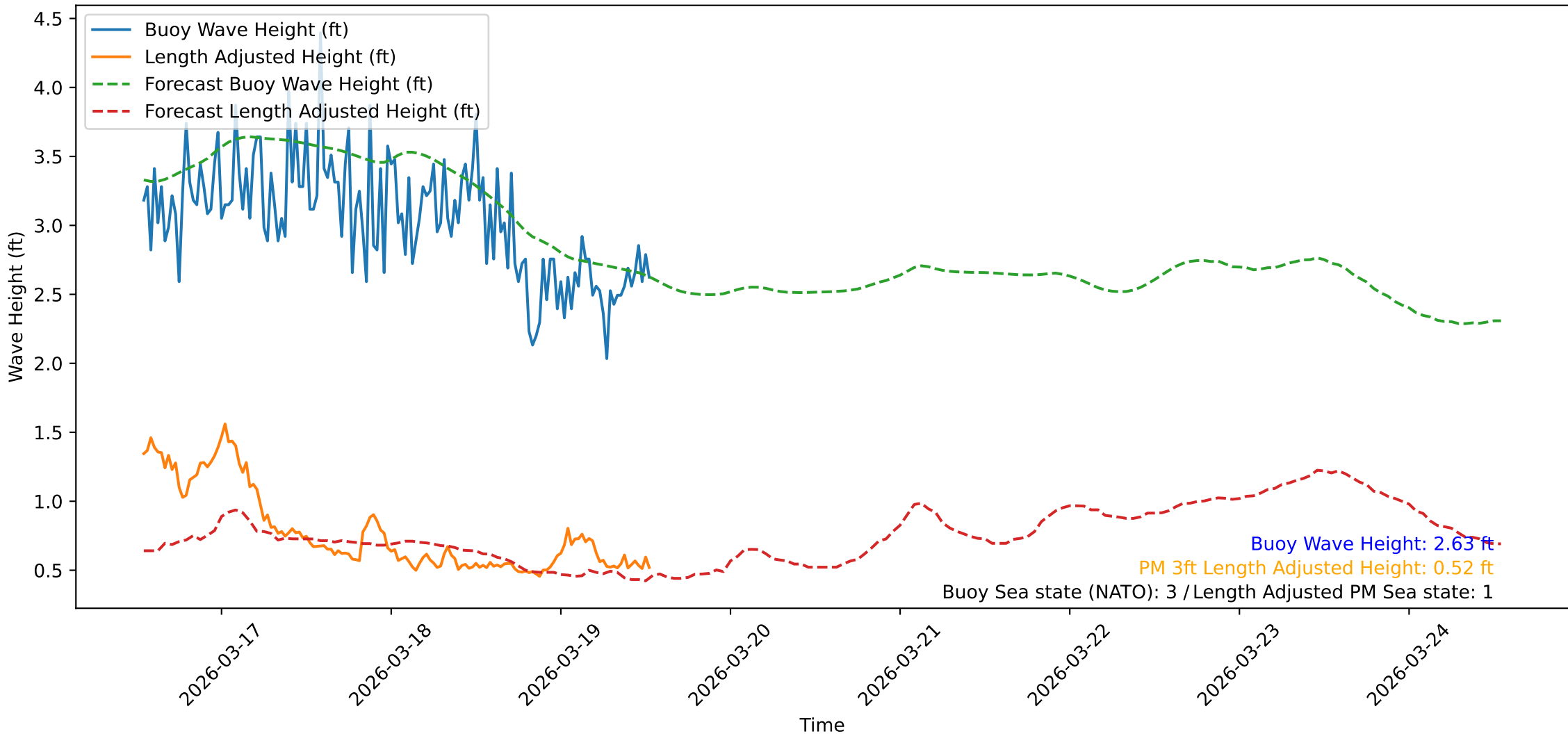
Wave Heights over Time for Oceanside Harbor at 2026-03-19 13:10:31
