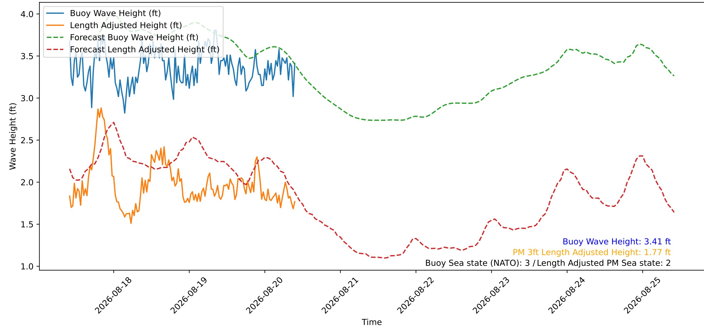
Wave Heights over Time for Oceanside Harbor at 2026-08-20 10:10:26
