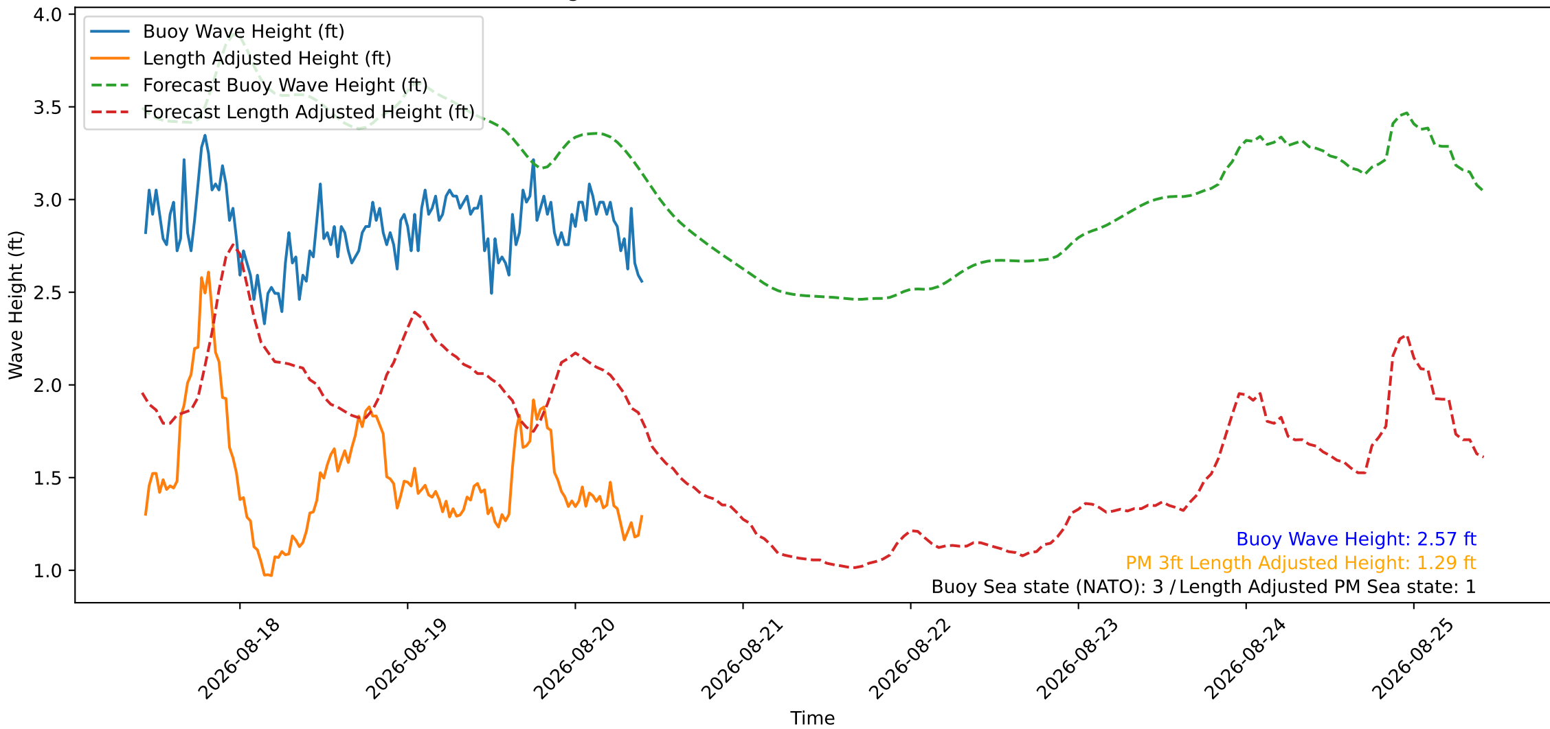
Wave Heights over Time for Red Beach at 2026-08-20 10:10:46
