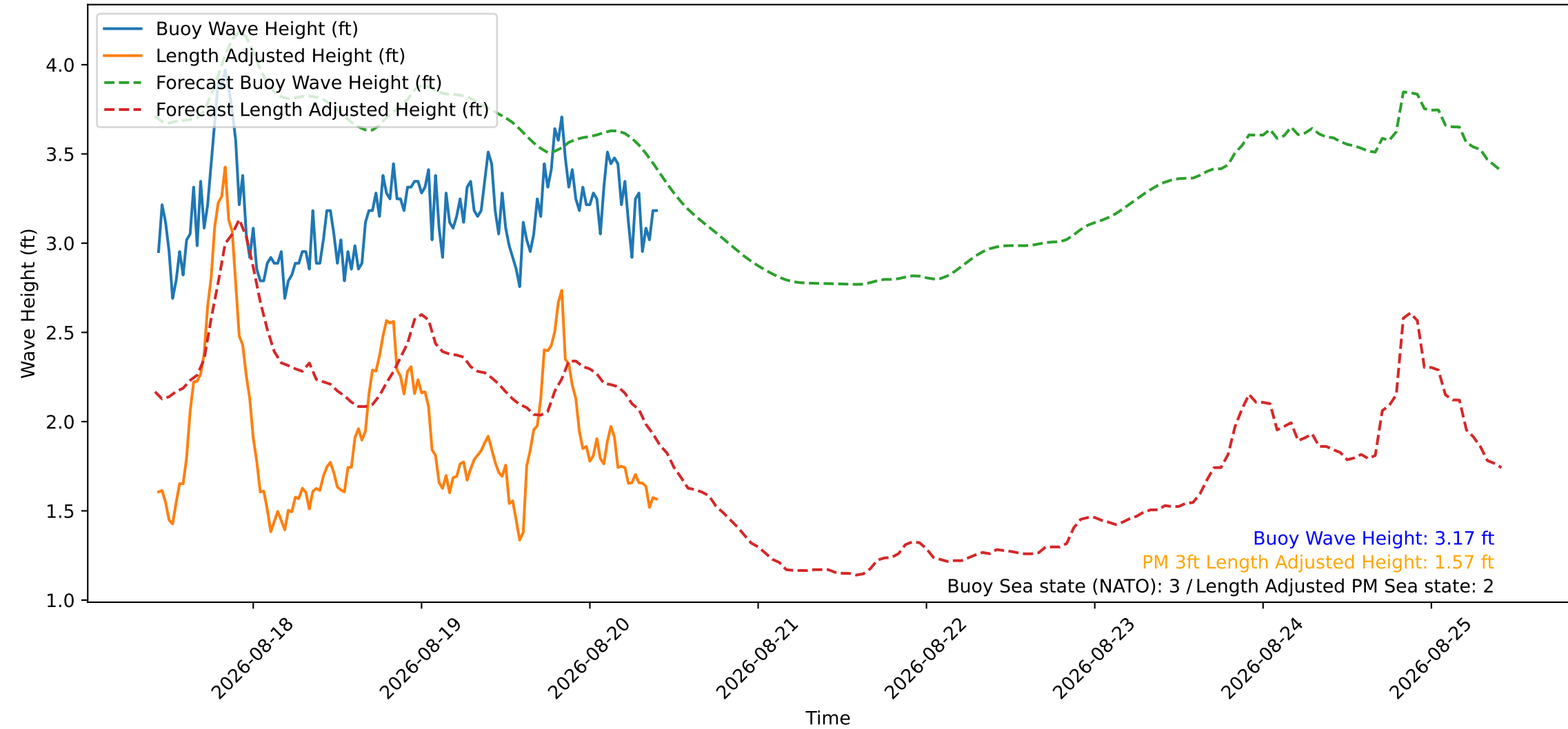
Wave Heights over Time for Green Beach at 2026-08-20 10:11:09
