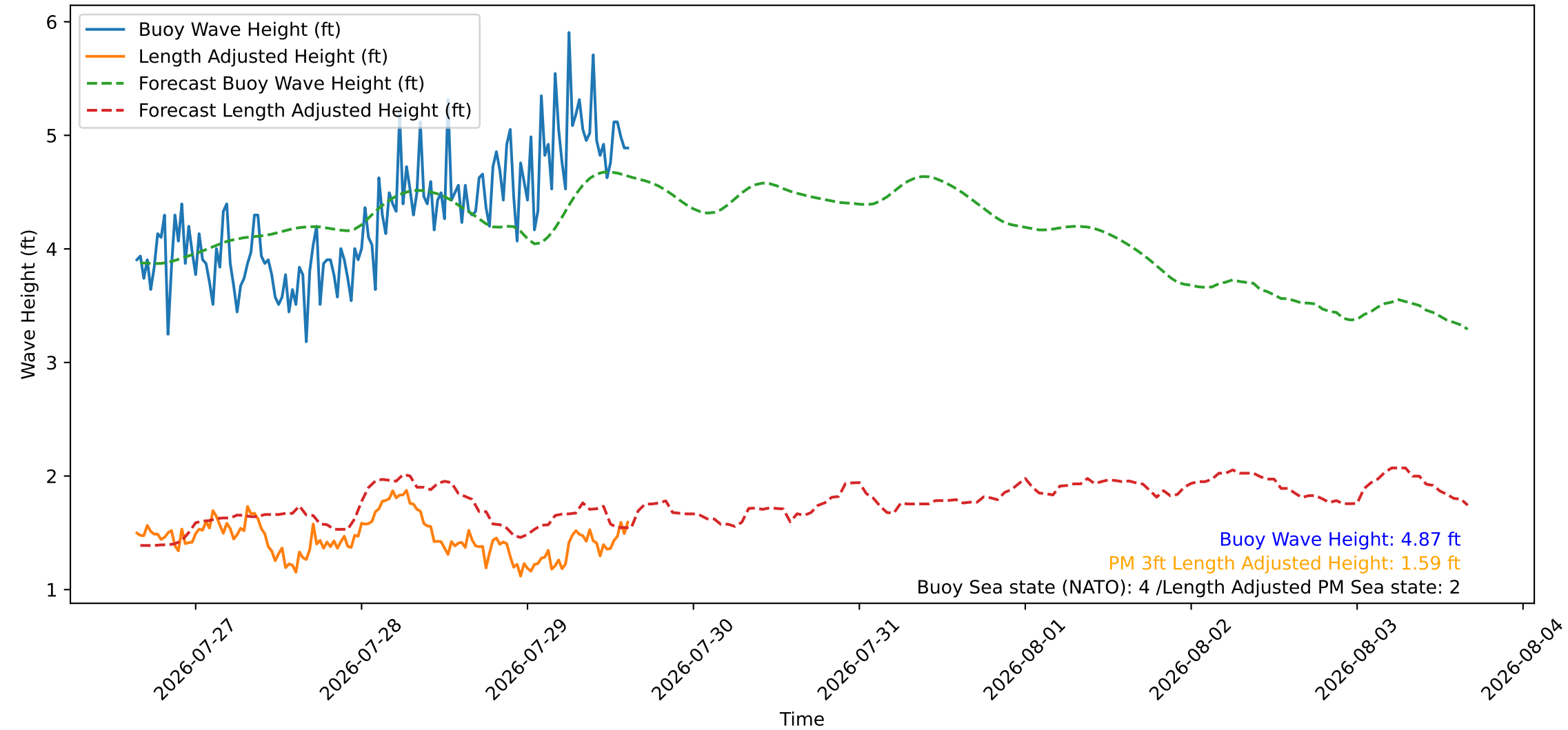
Wave Heights over Time for Oceanside Harbor at 2026-07-29 15:30:26
