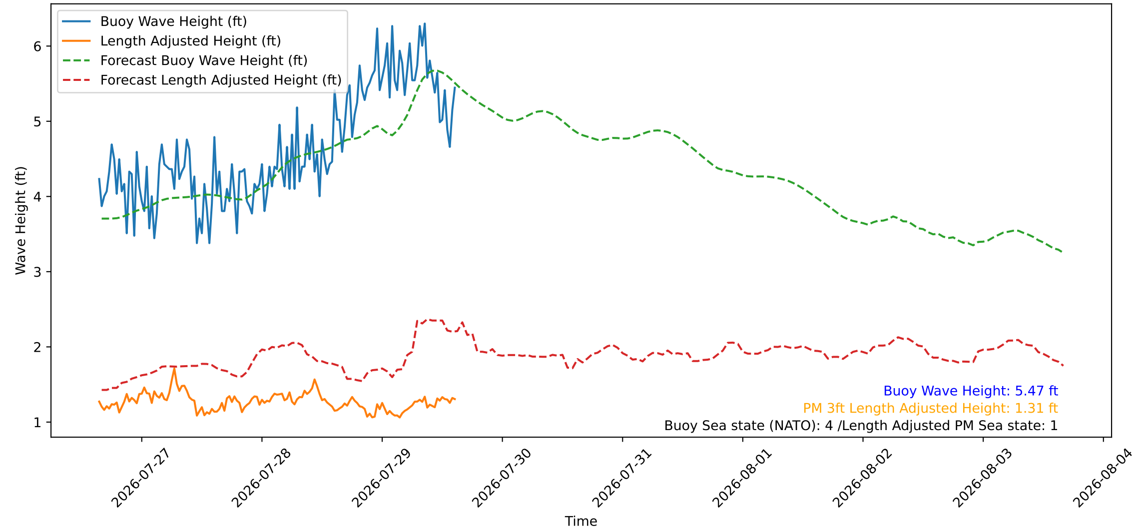
Wave Heights over Time for Green Beach at 2026-07-29 15:31:08
