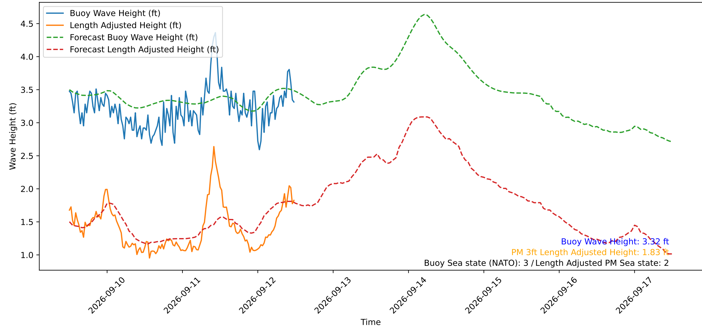
Wave Heights over Time for Oceanside Harbor at 2026-09-12 12:10:30
