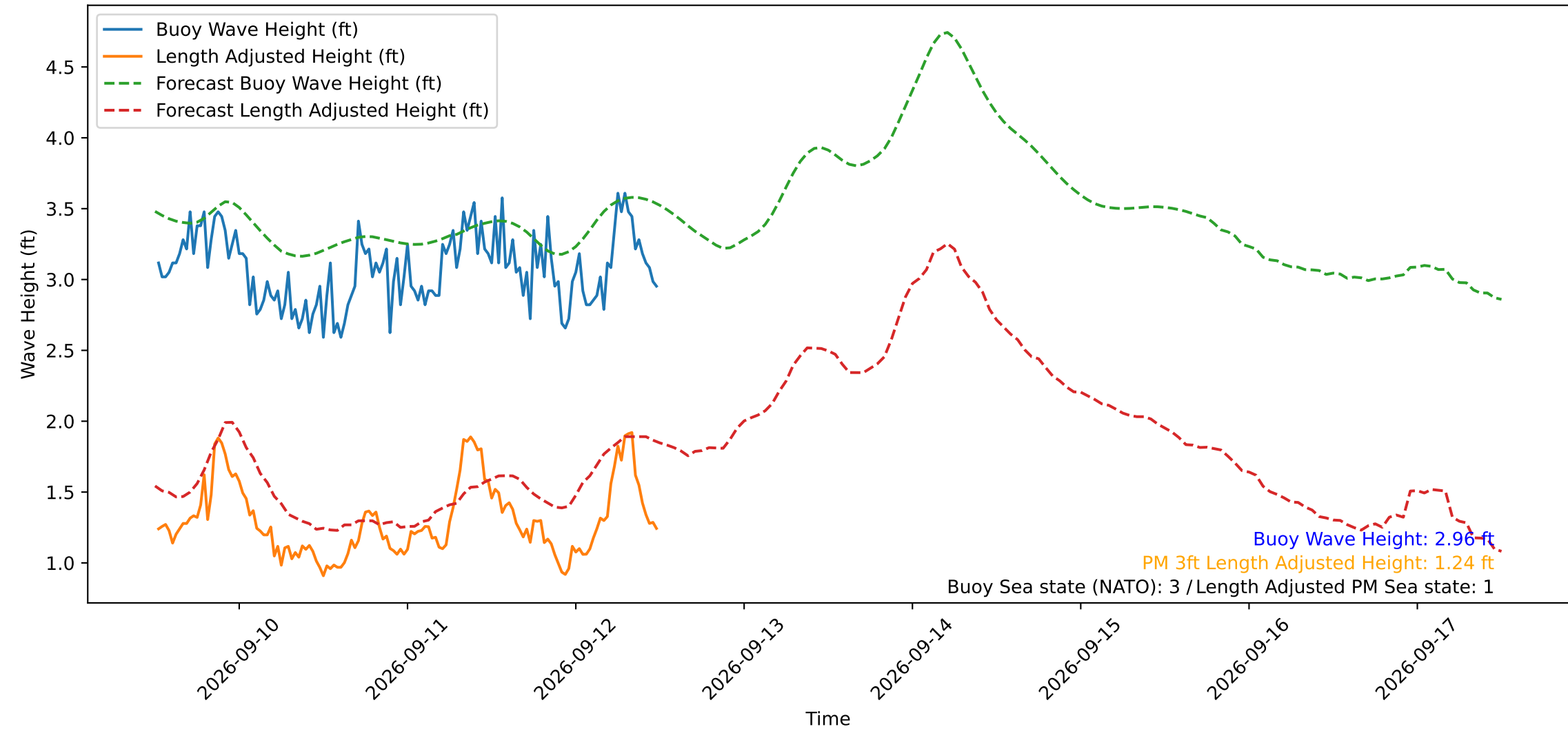
Wave Heights over Time for Green Beach at 2026-09-12 12:11:12
