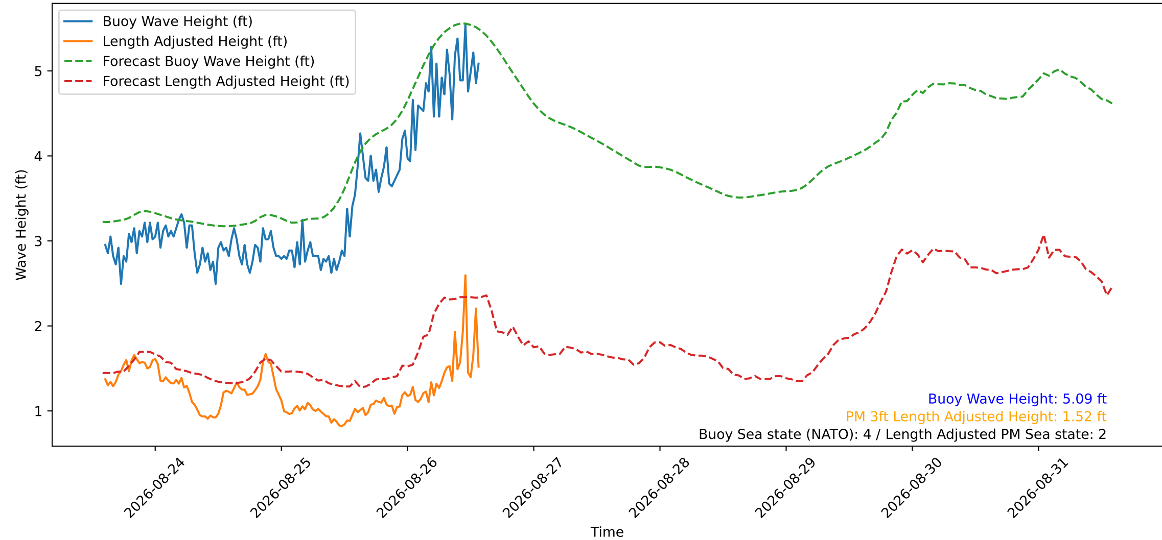
Wave Heights over Time for Green Beach at 2026-08-26 14:21:14
