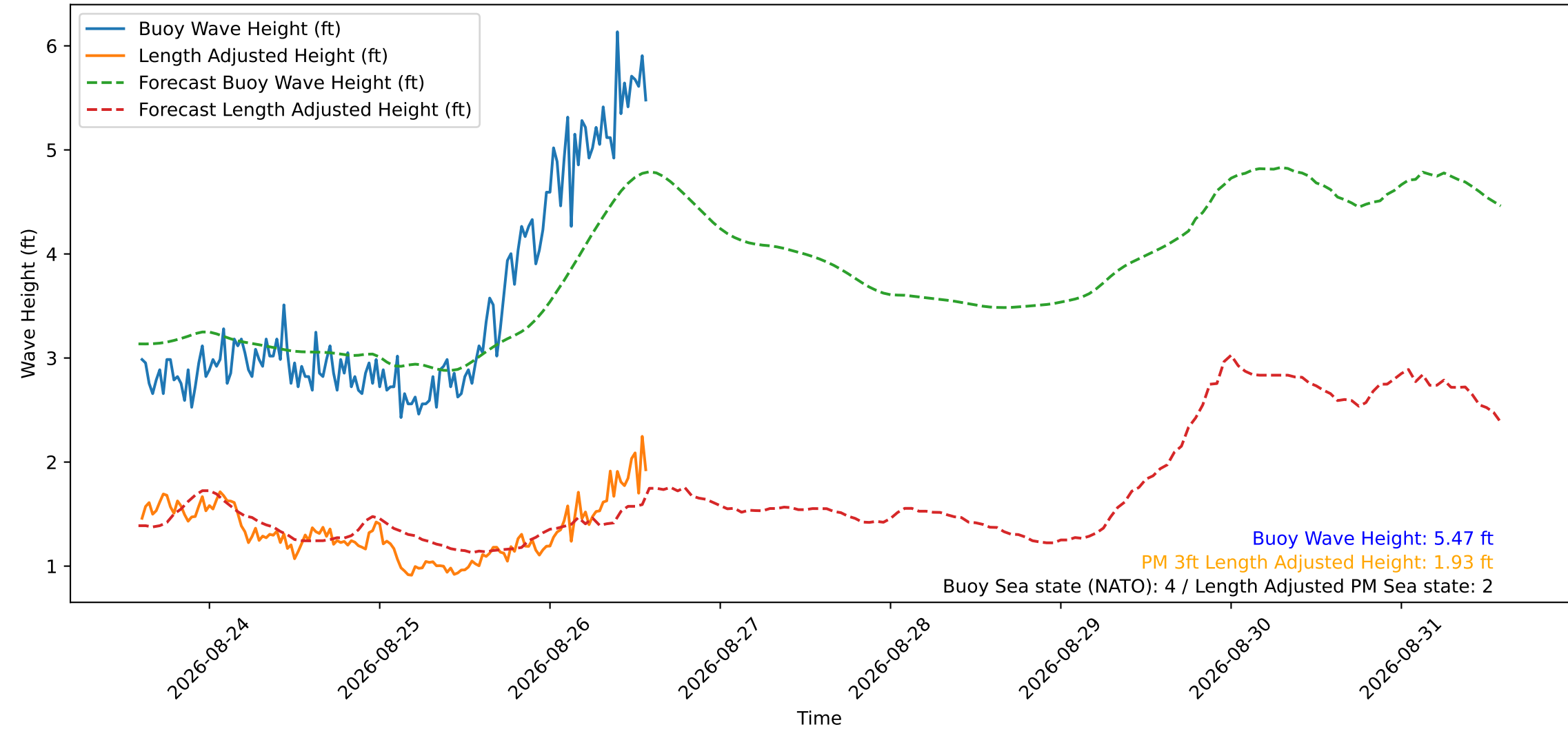
Wave Heights over Time for Oceanside Harbor at 2026-08-26 14:20:29
