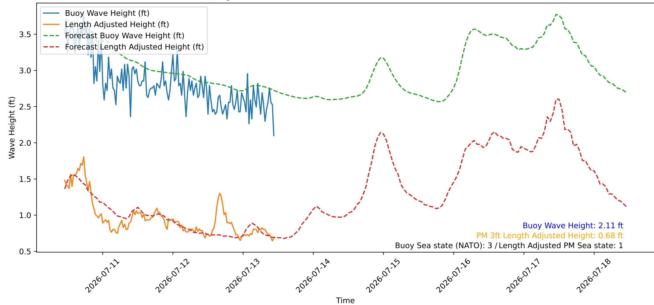
Wave Heights over Time for Oceanside Harbor at 2026-07-13 11:10:26
