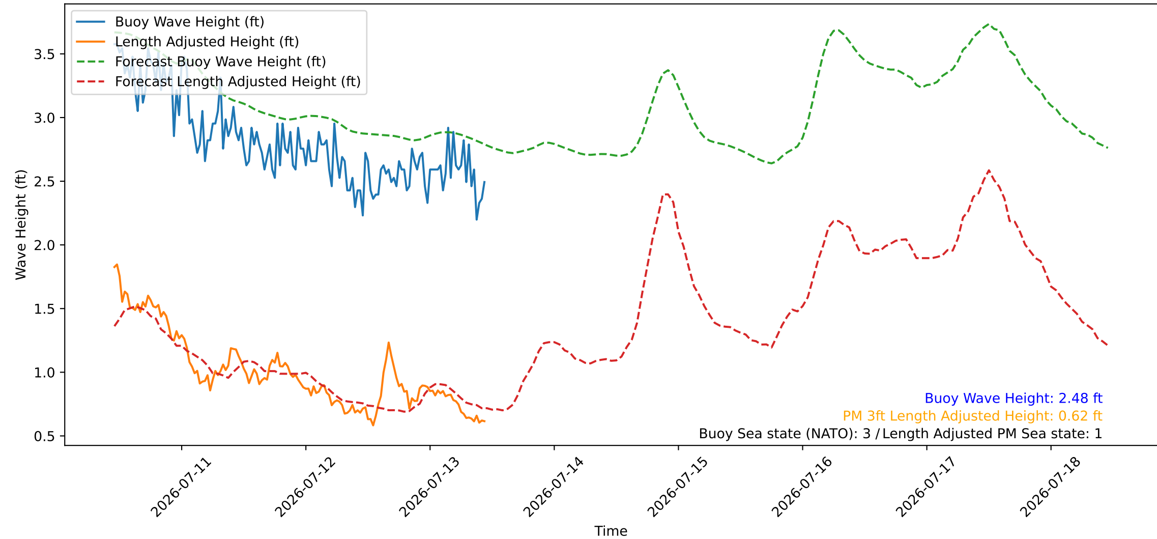
Wave Heights over Time for Green Beach at 2026-07-13 11:11:08
