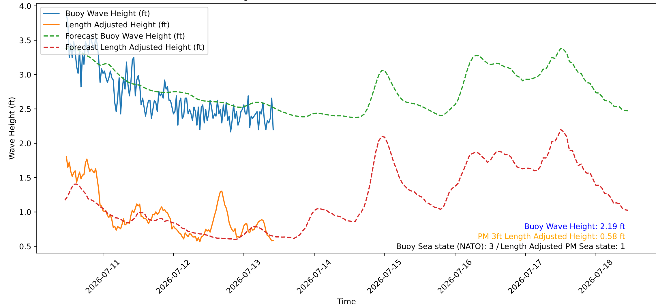
Wave Heights over Time for Red Beach at 2026-07-13 11:10:46
