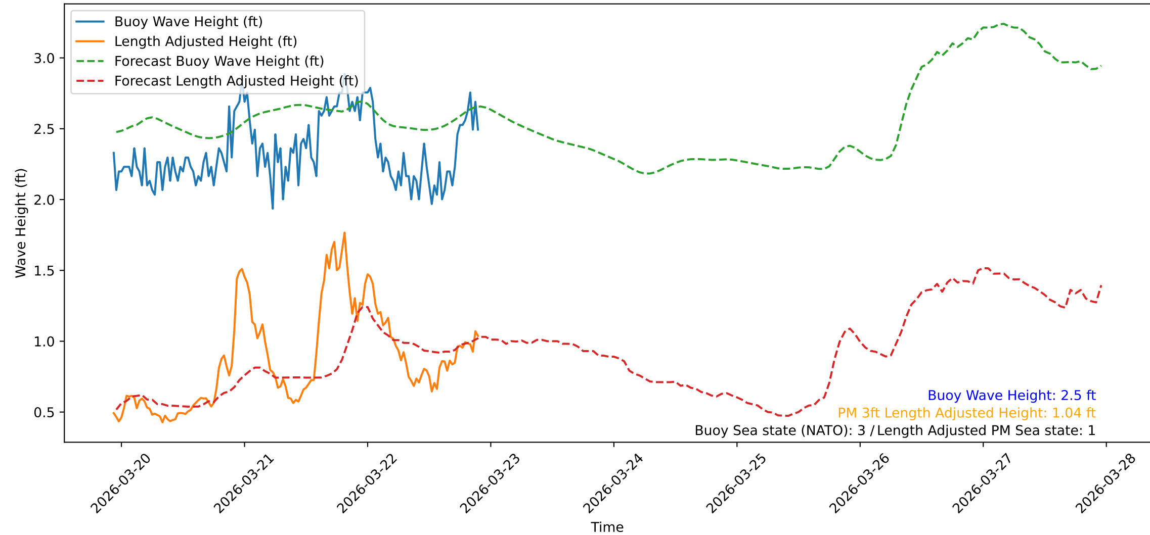
Wave Heights over Time for Green Beach at 2026-03-22 22:31:09
