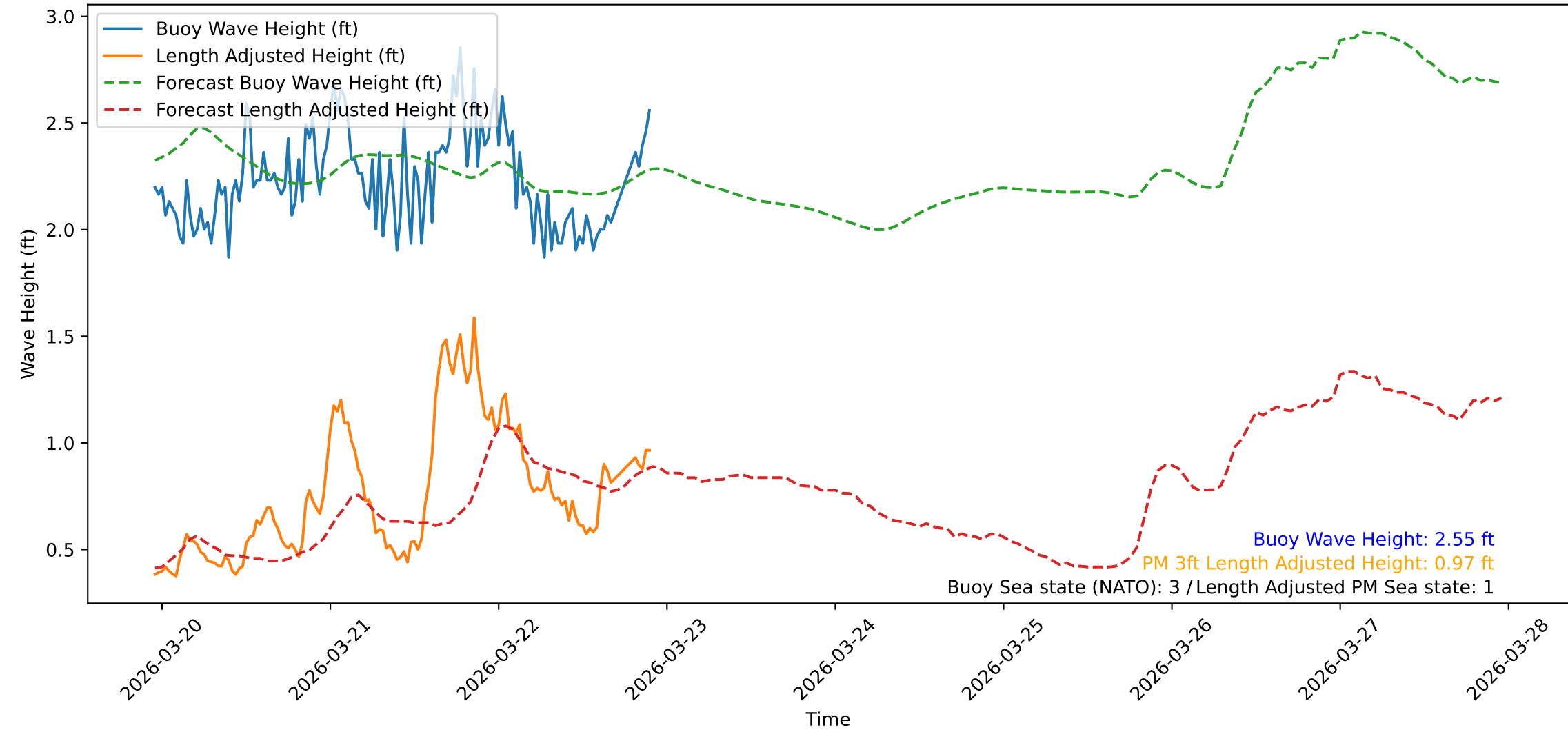
Wave Heights over Time for Red Beach at 2026-03-22 22:30:47
