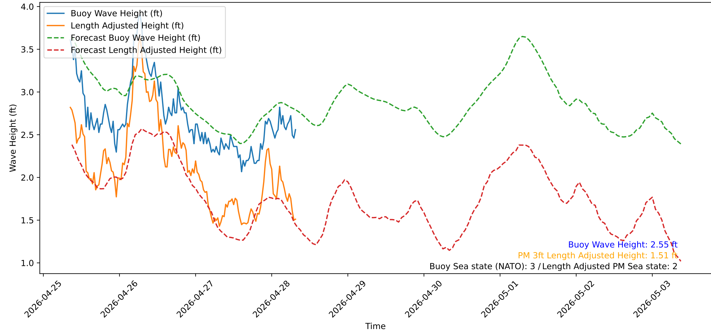
Wave Heights over Time for Oceanside Harbor at 2026-04-28 08:30:31
