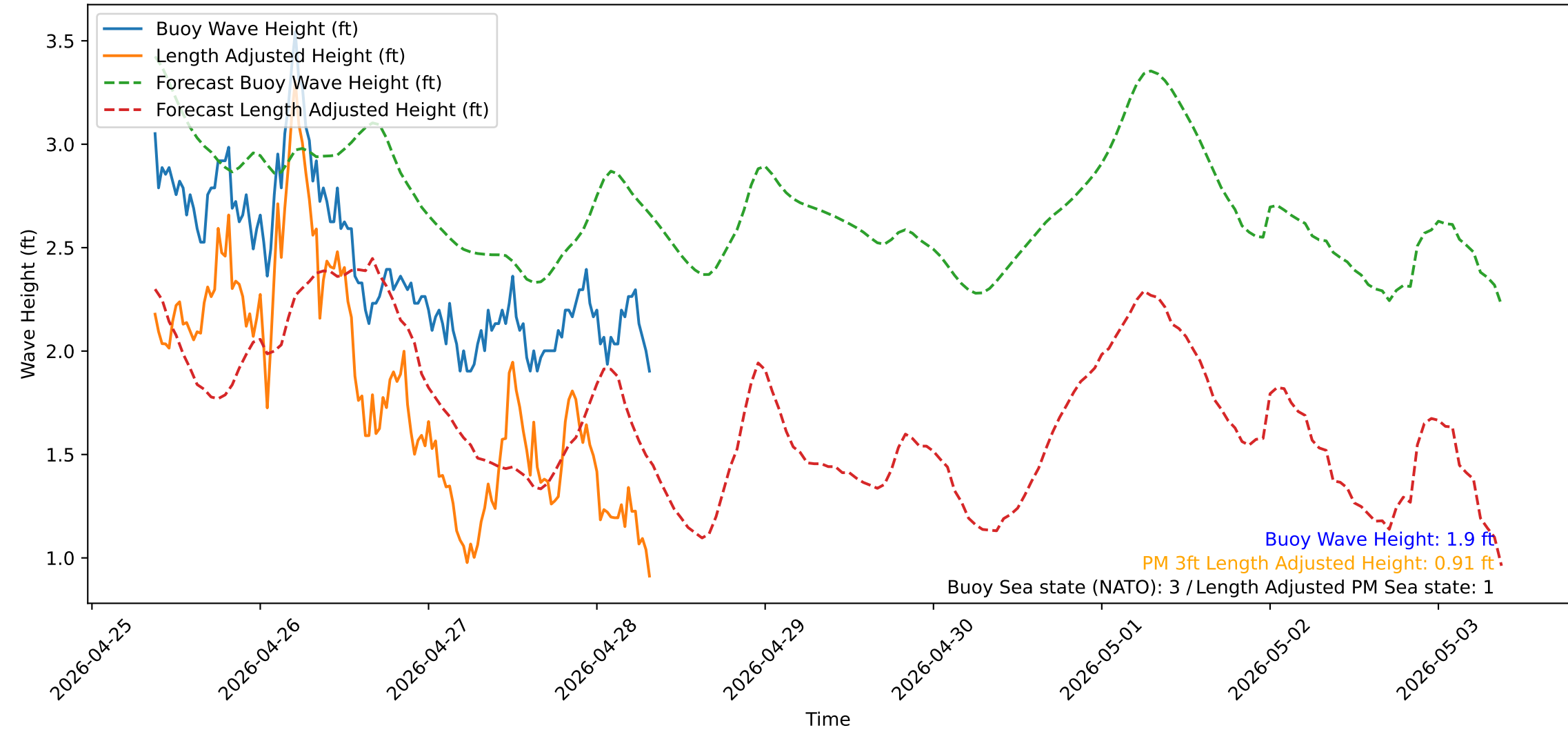
Wave Heights over Time for Red Beach at 2026-04-28 08:30:50
