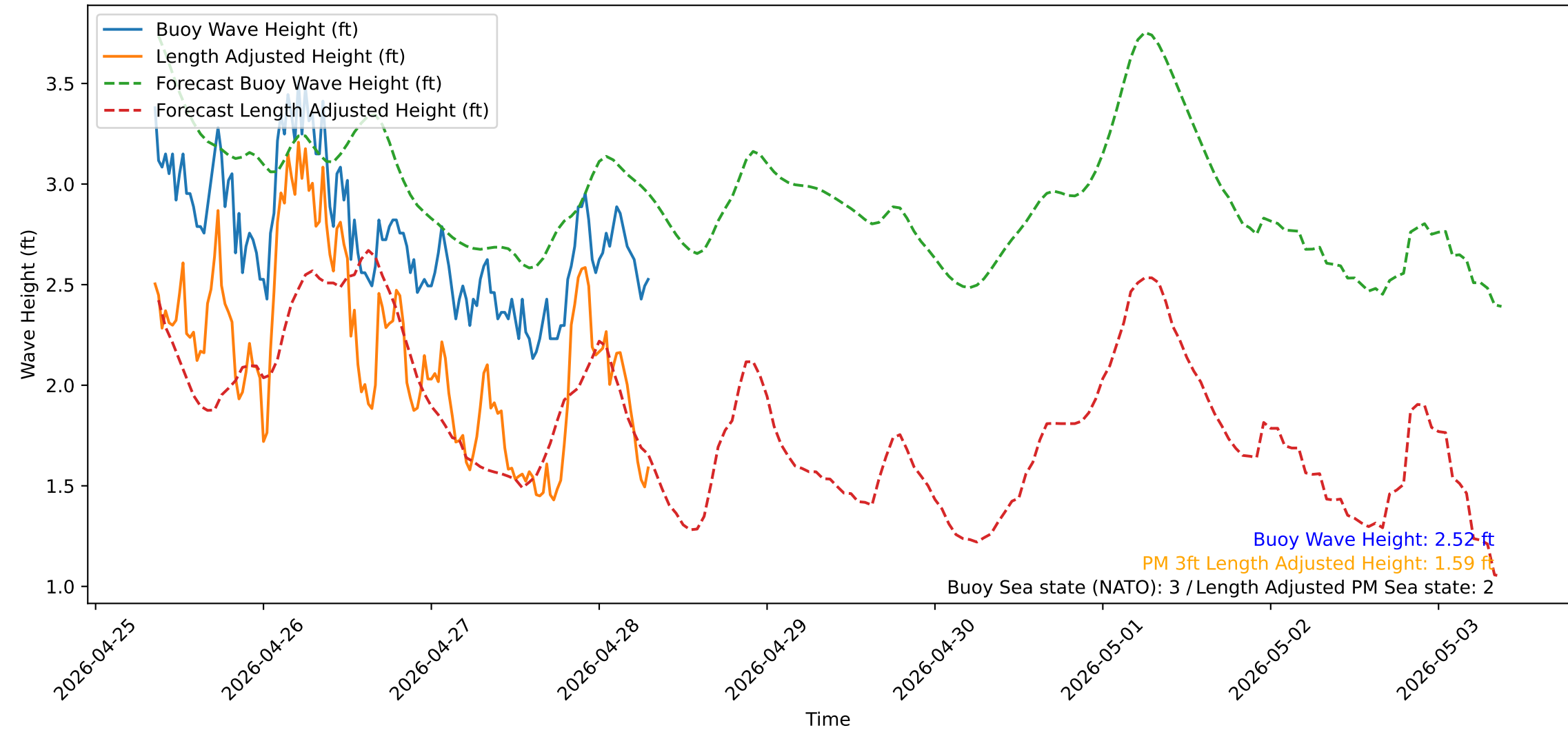
Wave Heights over Time for Green Beach at 2026-04-28 08:31:12
