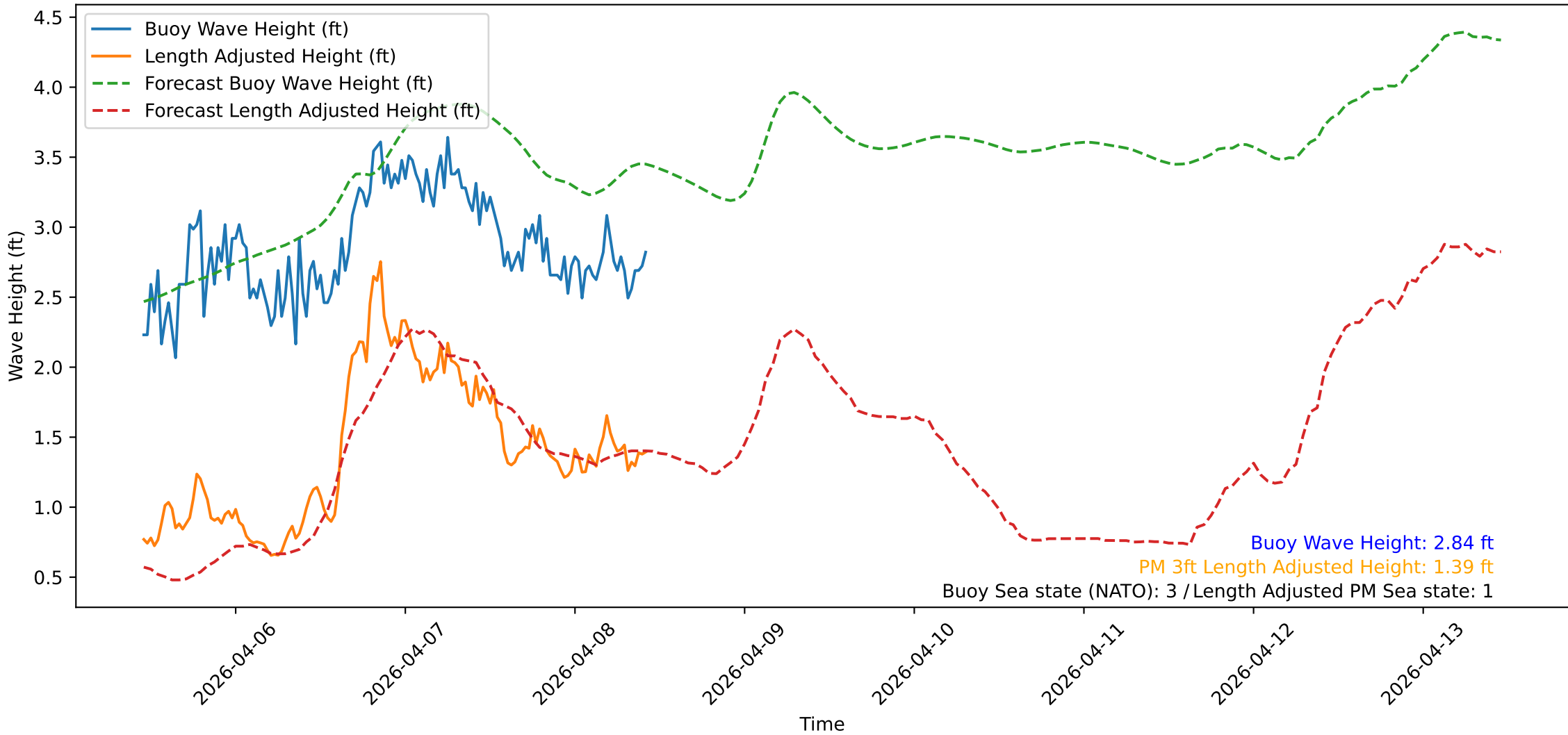
Wave Heights over Time for Oceanside Harbor at 2026-04-08 10:50:31
