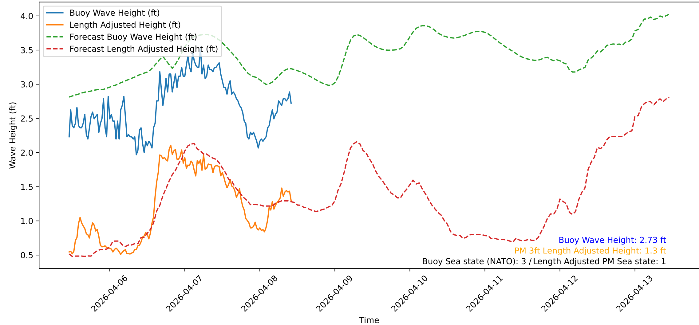
Wave Heights over Time for Red Beach at 2026-04-08 10:50:47
