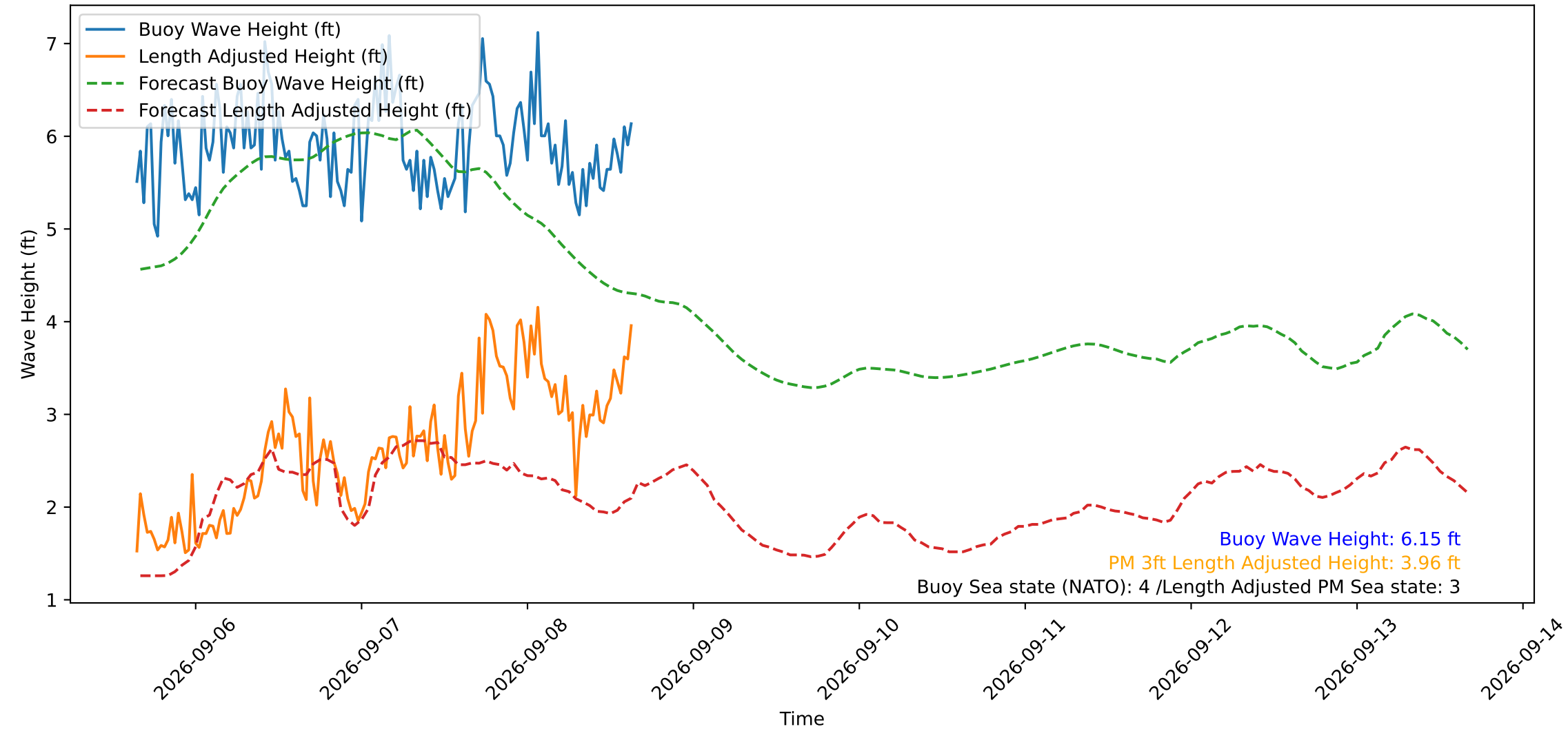
Wave Heights over Time for Oceanside Harbor at 2026-09-08 15:40:29
