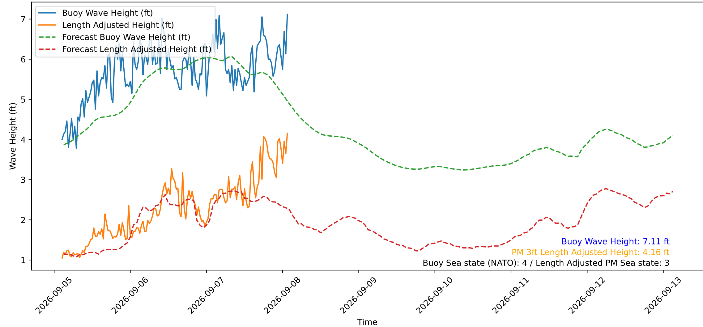
Wave Heights over Time for Oceanside Harbor at 2026-09-08 02:30:30
