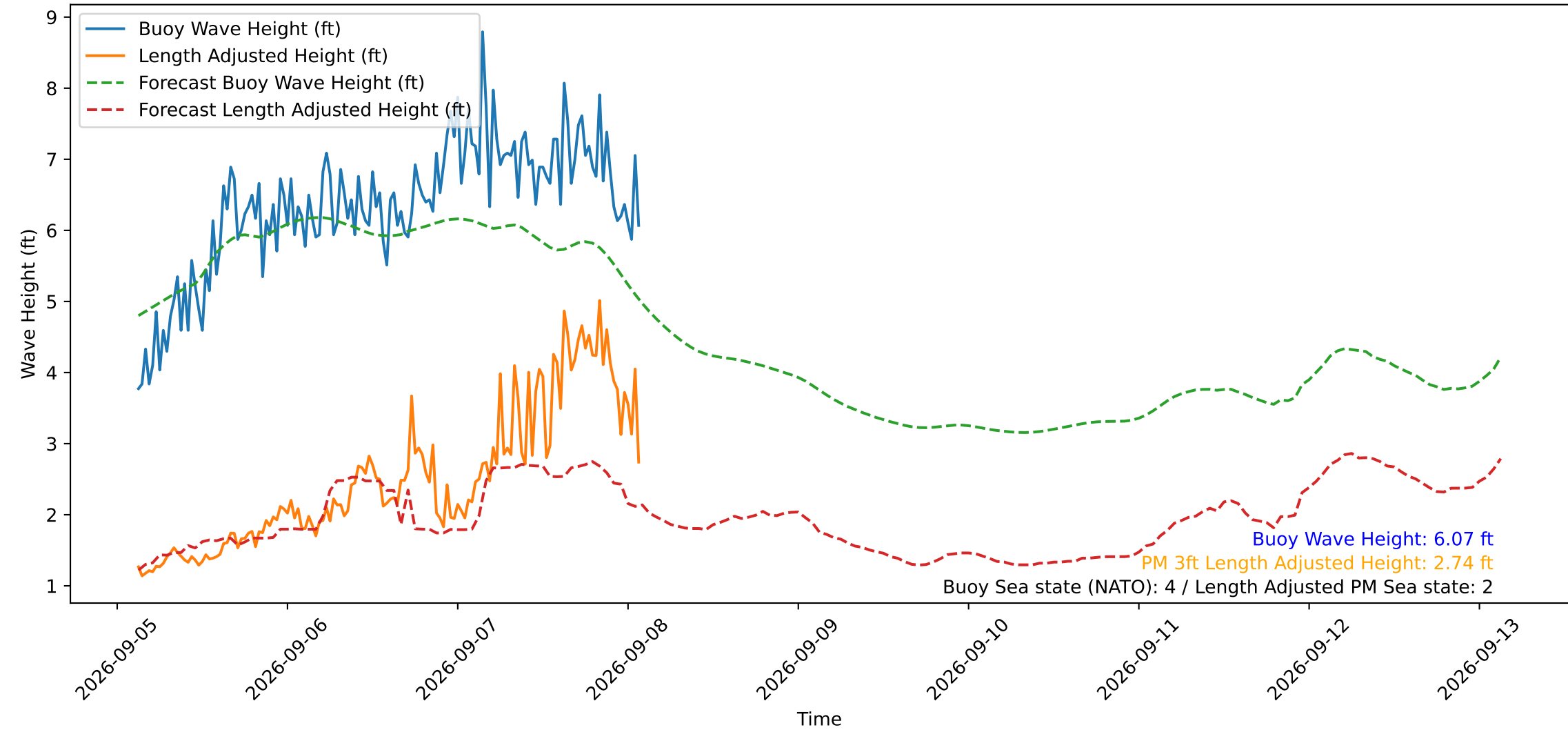
Wave Heights over Time for Green Beach at 2026-09-08 02:31:11
