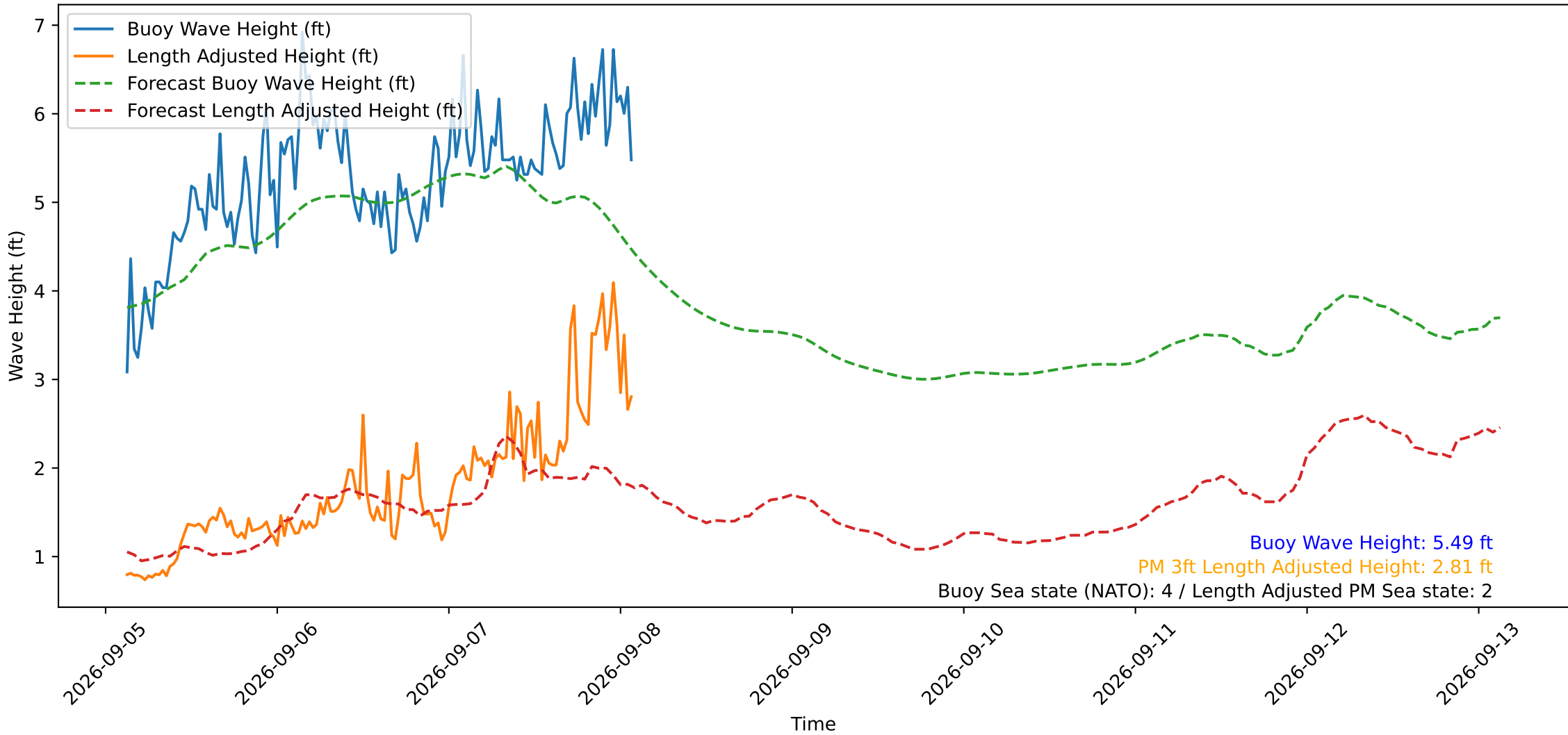
Wave Heights over Time for Red Beach at 2026-09-08 02:30:49
