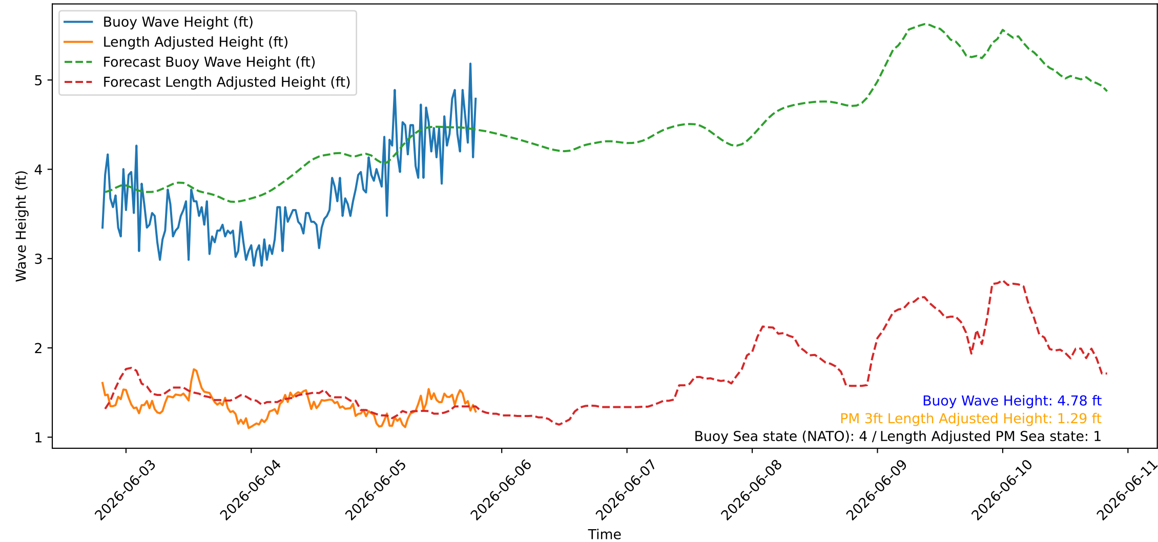
Wave Heights over Time for Oceanside Harbor at 2026-06-05 19:40:26
