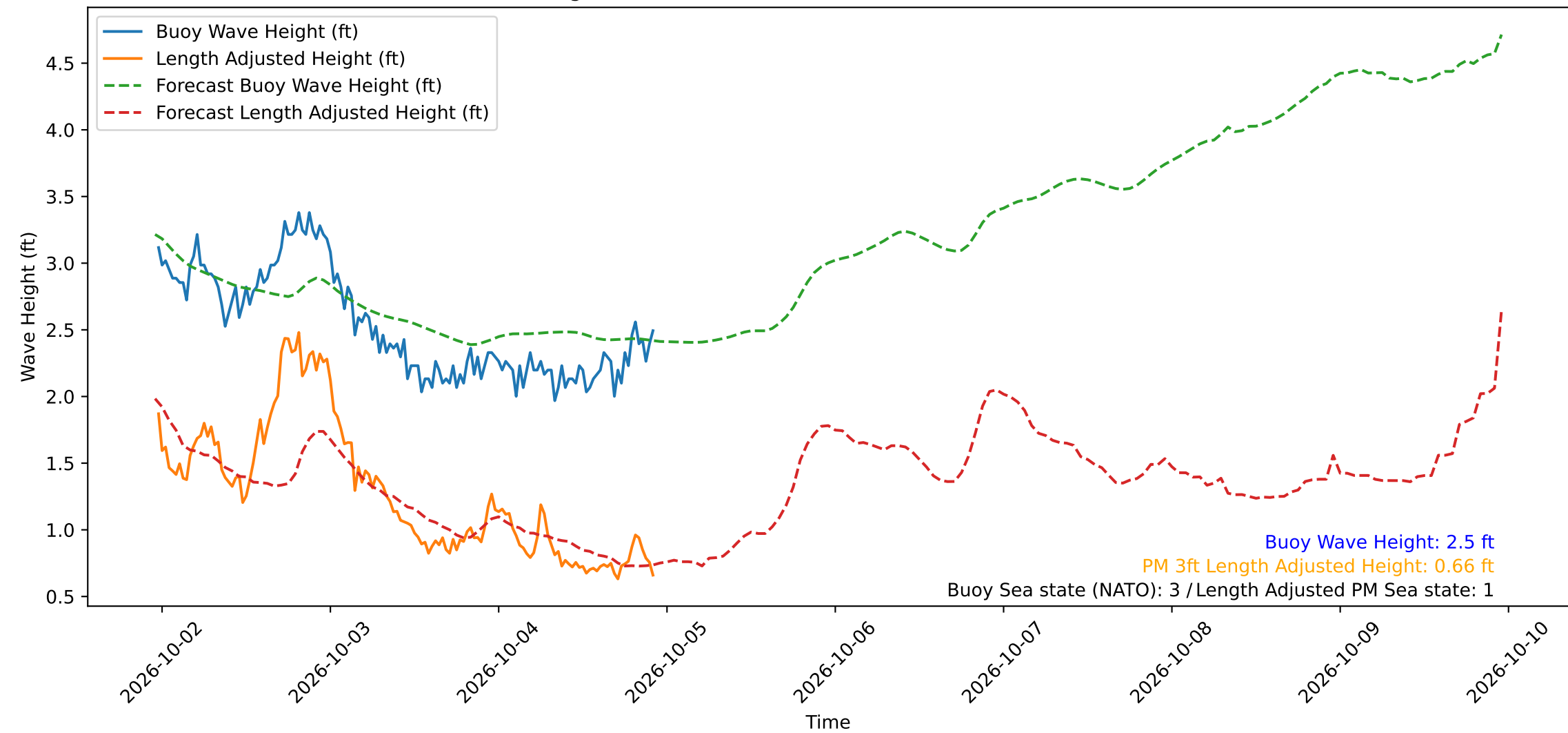
Wave Heights over Time for Green Beach at 2026-10-04 23:01:11
