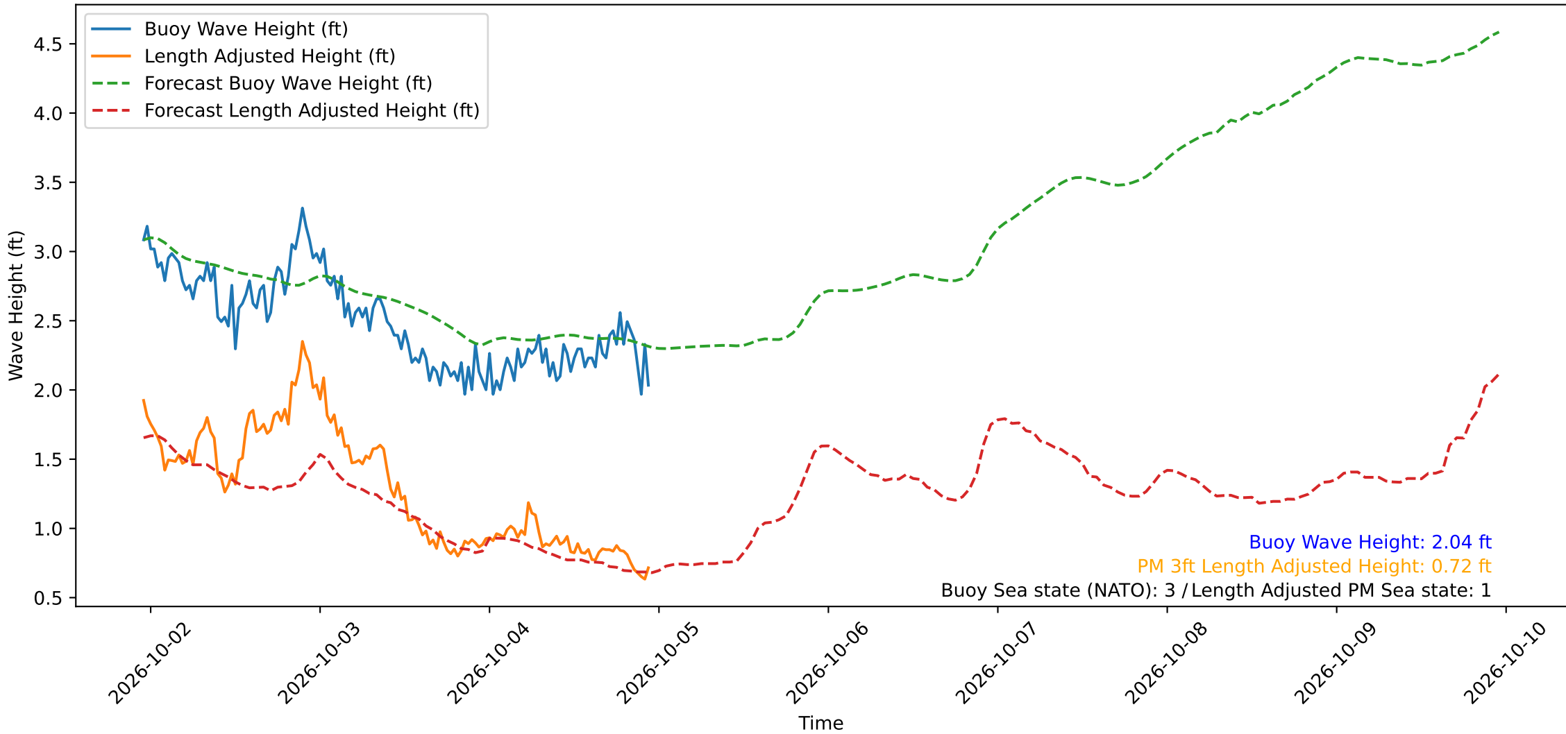
Wave Heights over Time for Oceanside Harbor at 2026-10-04 23:00:30
