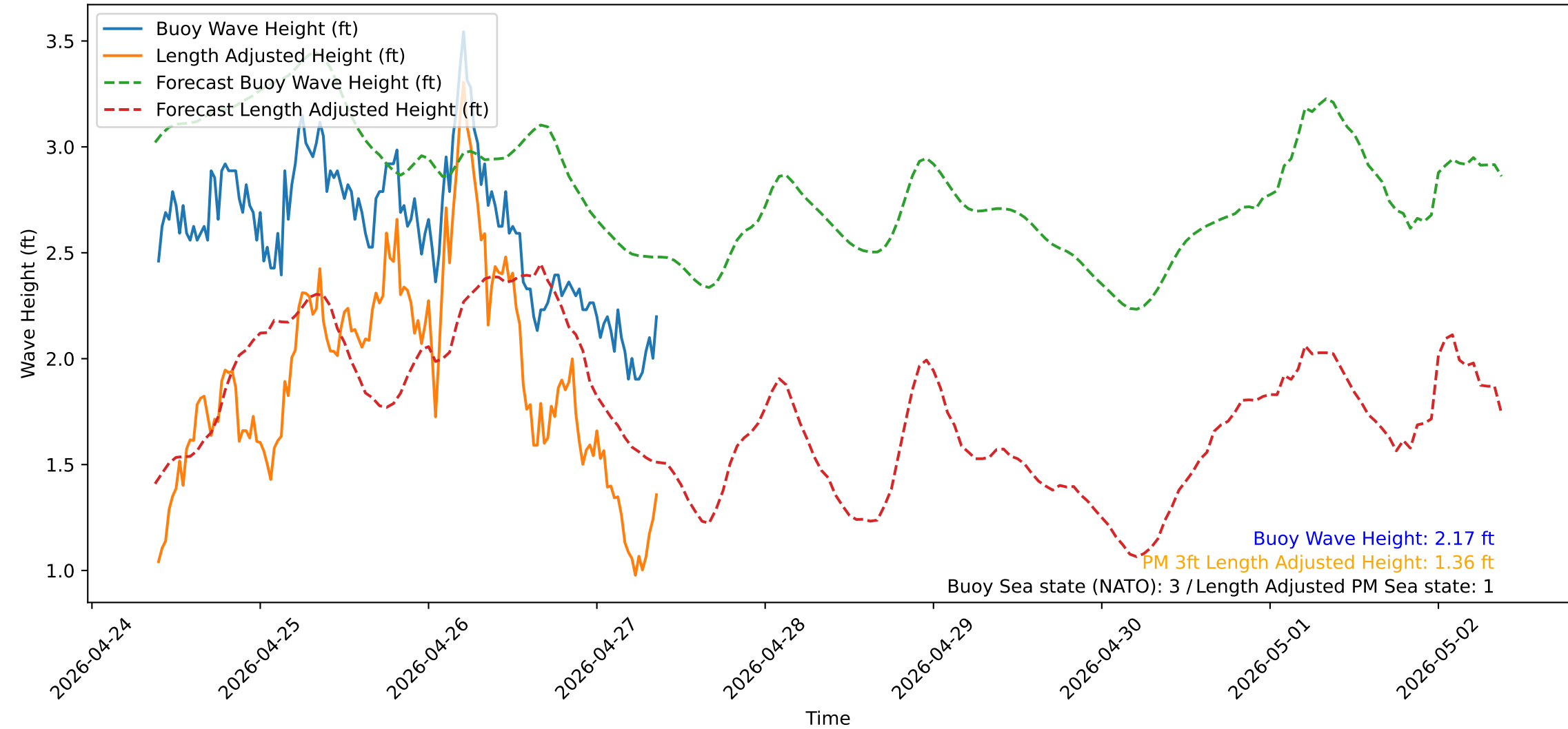
Wave Heights over Time for Red Beach at 2026-04-27 09:10:51
