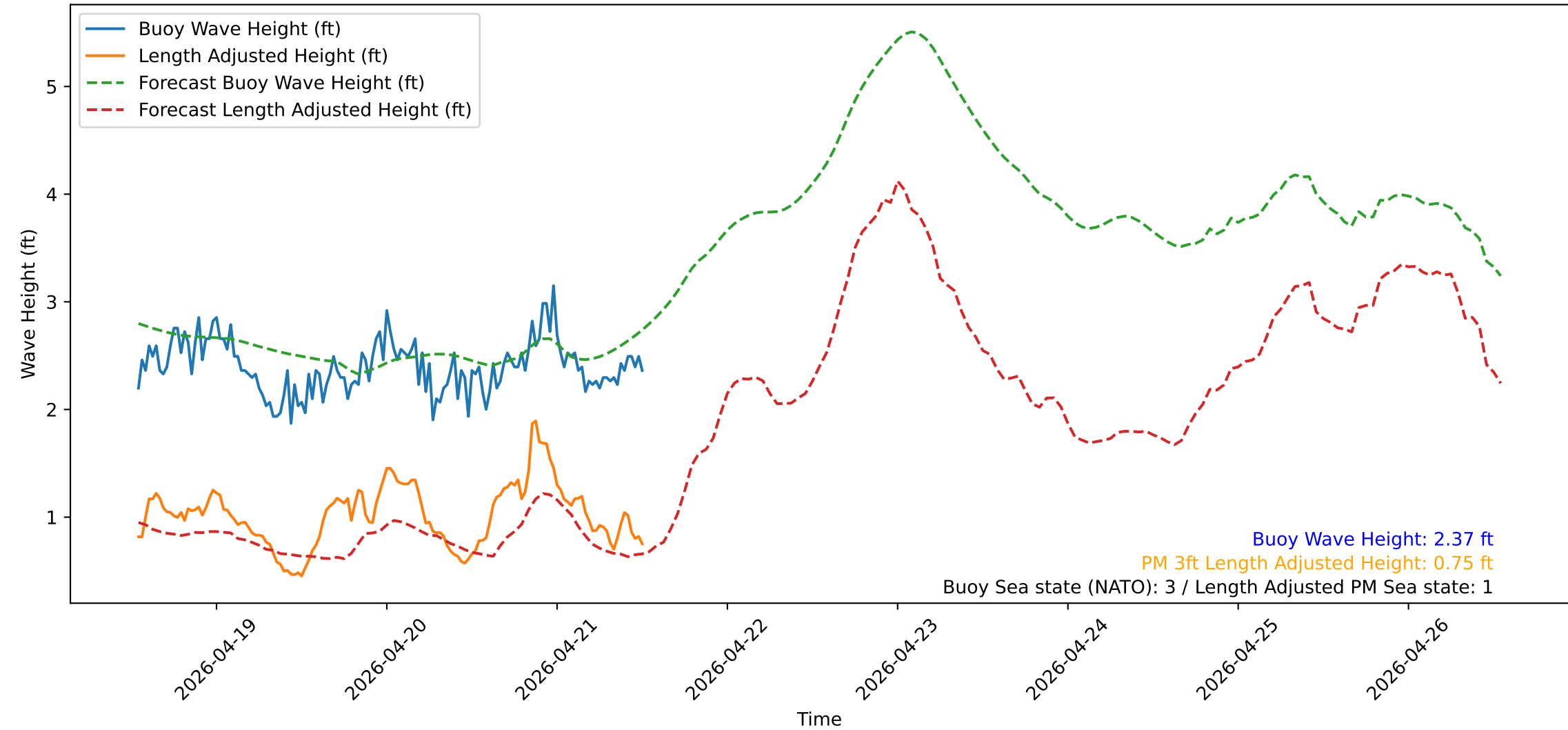
Wave Heights over Time for Green Beach at 2026-04-21 13:01:12
