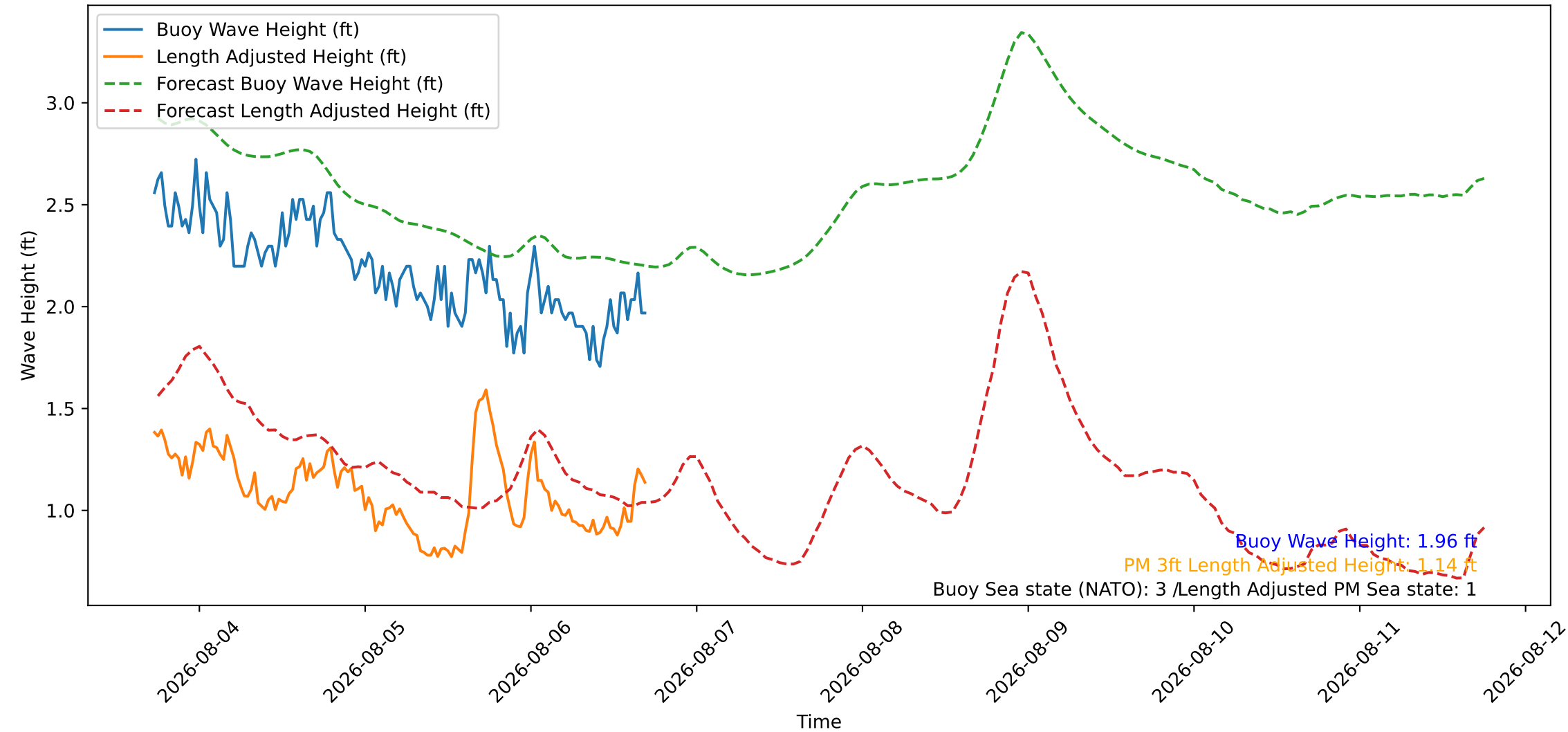
Wave Heights over Time for Oceanside Harbor at 2026-08-06 17:30:26
