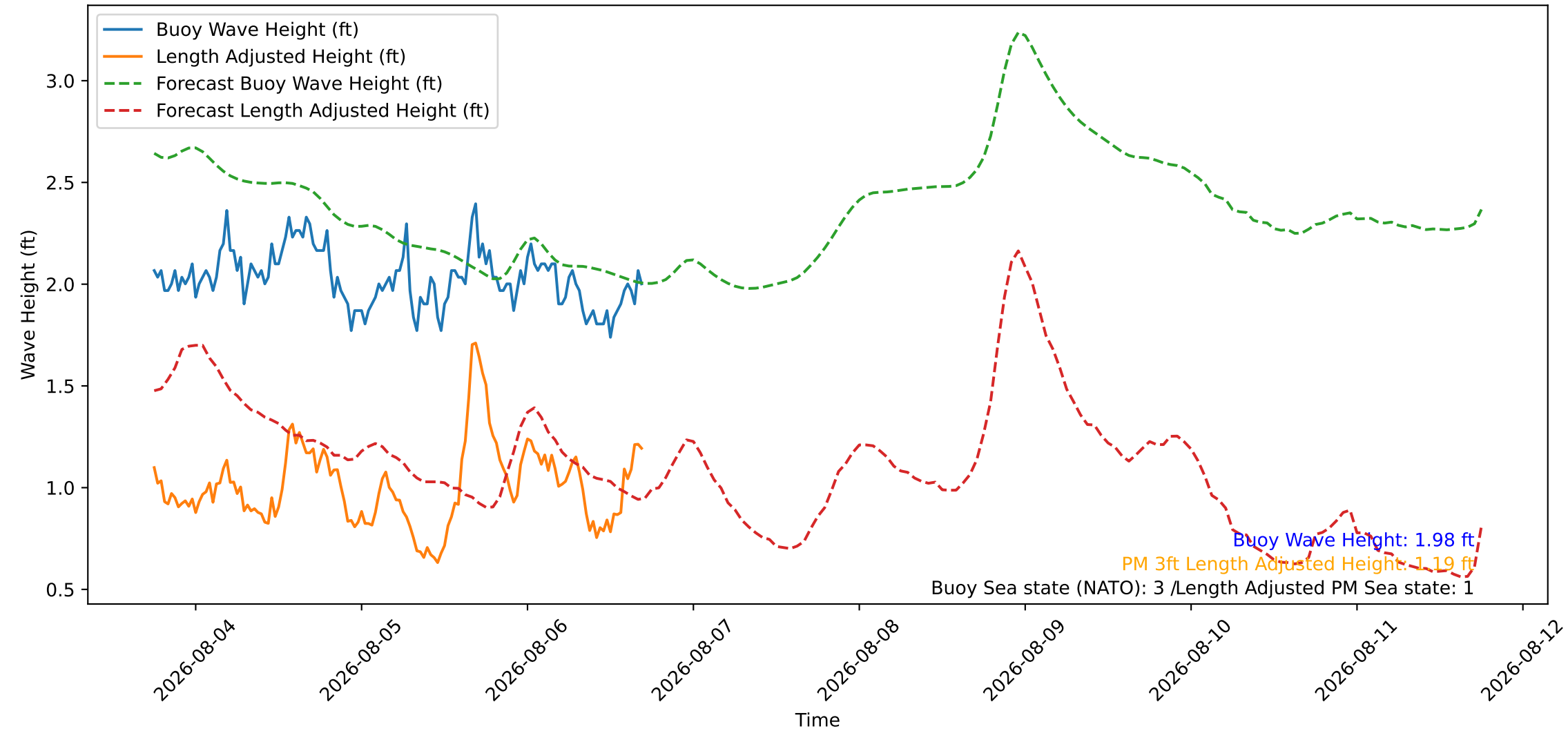
Wave Heights over Time for Red Beach at 2026-08-06 17:30:45
