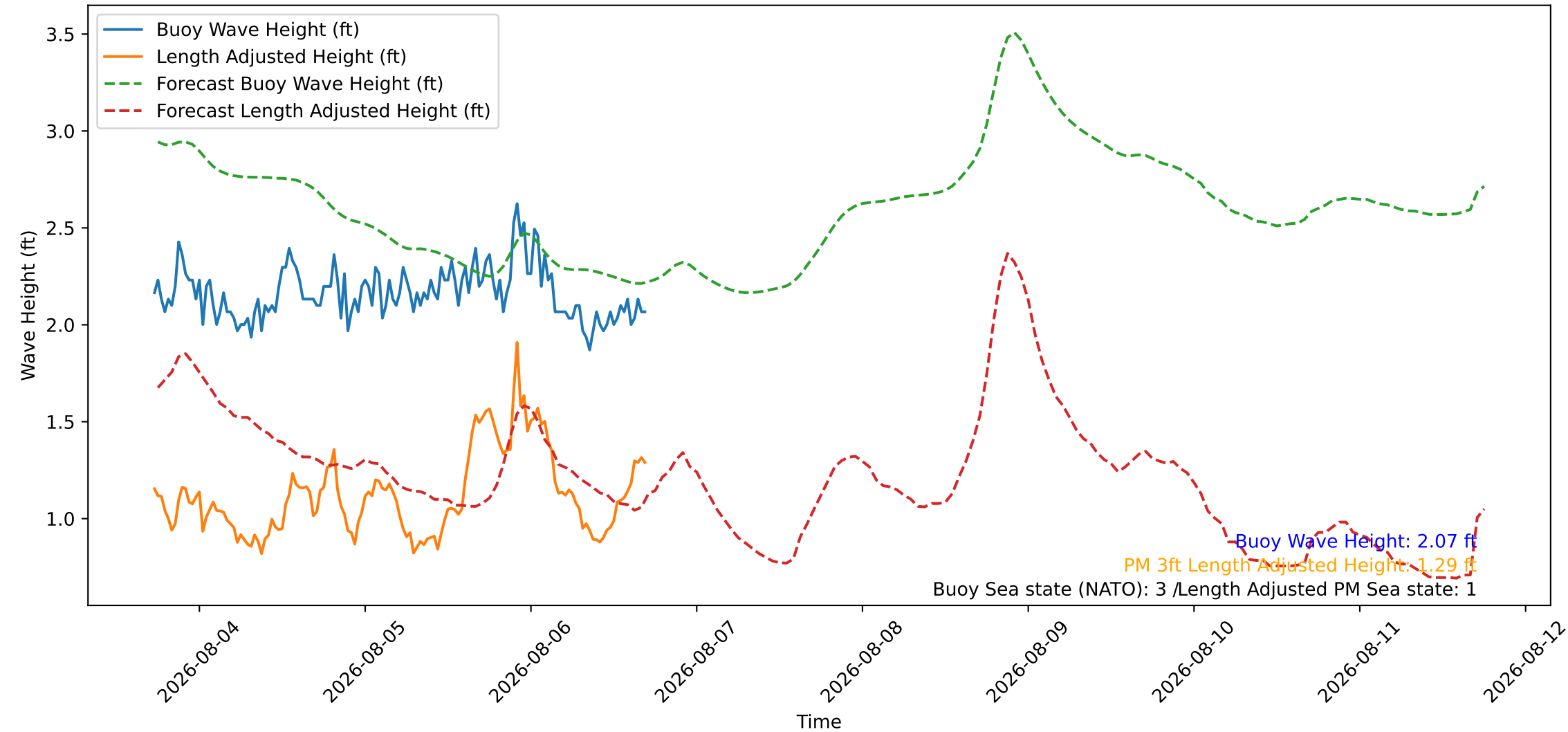
Wave Heights over Time for Green Beach at 2026-08-06 17:31:07
