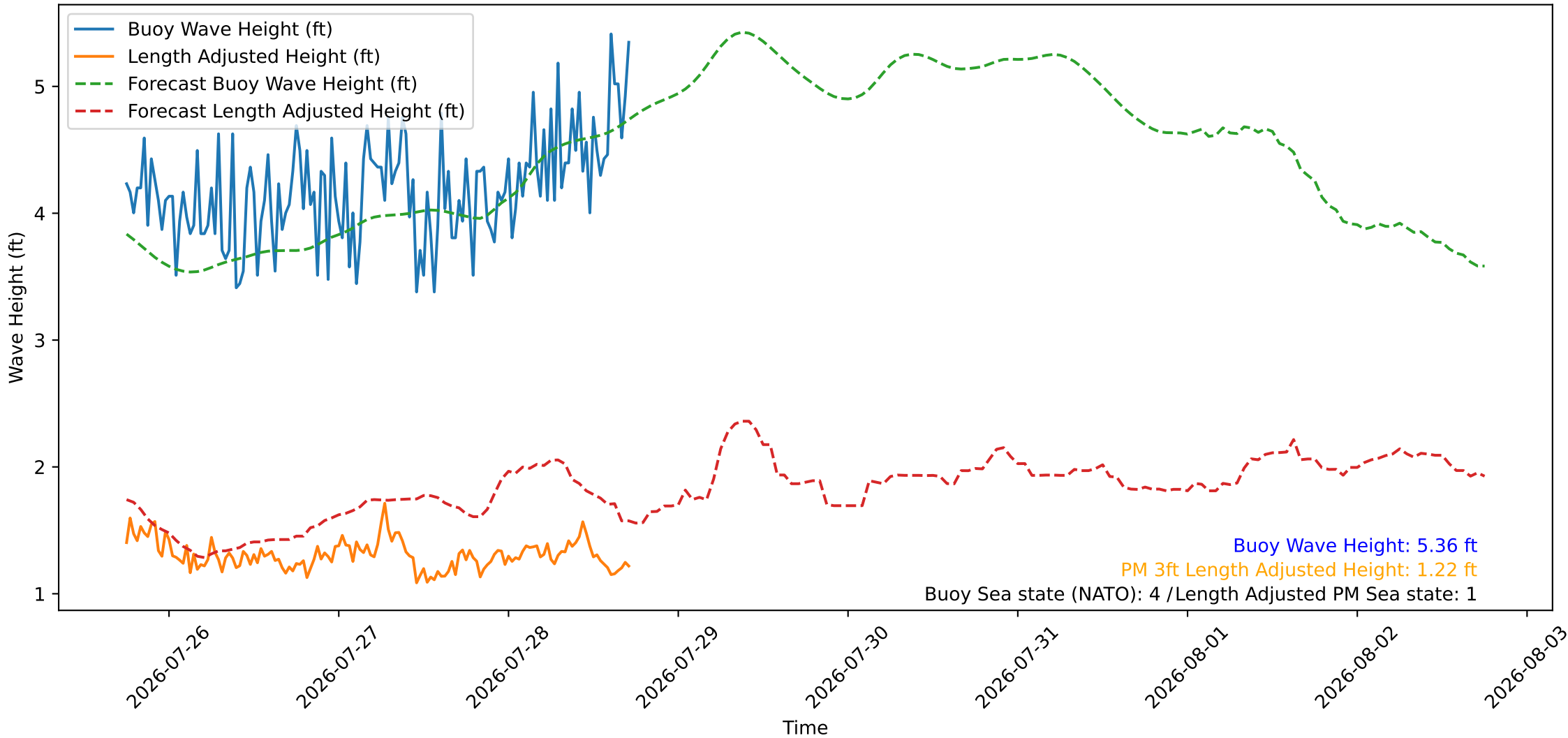
Wave Heights over Time for Green Beach at 2026-07-28 18:01:08
