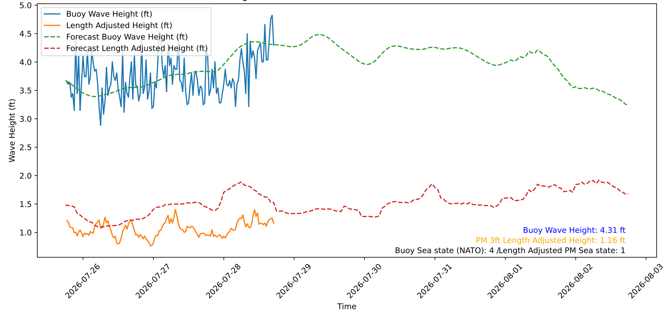
Wave Heights over Time for Red Beach at 2026-07-28 18:00:46
