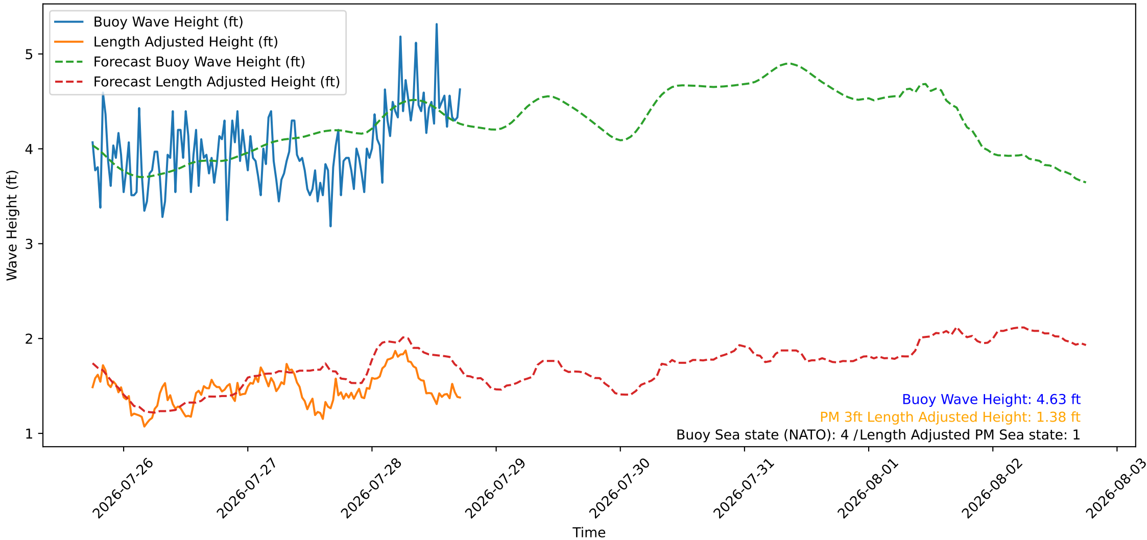
Wave Heights over Time for Oceanside Harbor at 2026-07-28 18:00:26
