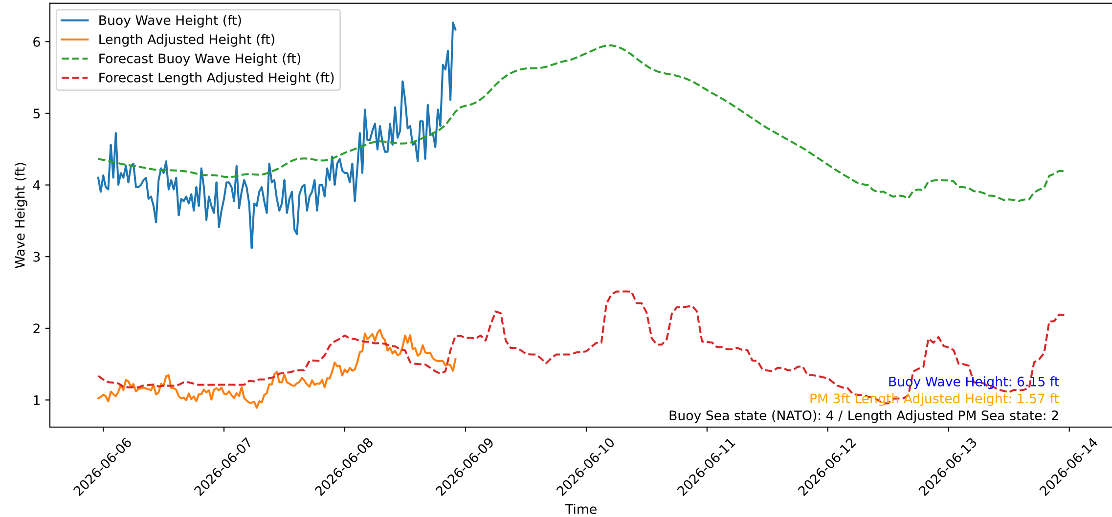
Wave Heights over Time for Green Beach at 2026-06-08 23:01:08
