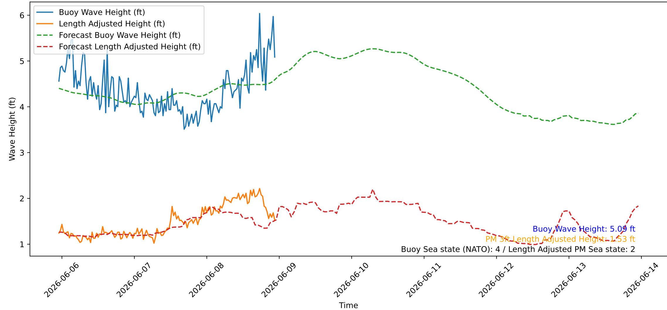
Wave Heights over Time for Oceanside Harbor at 2026-06-08 23:00:26
