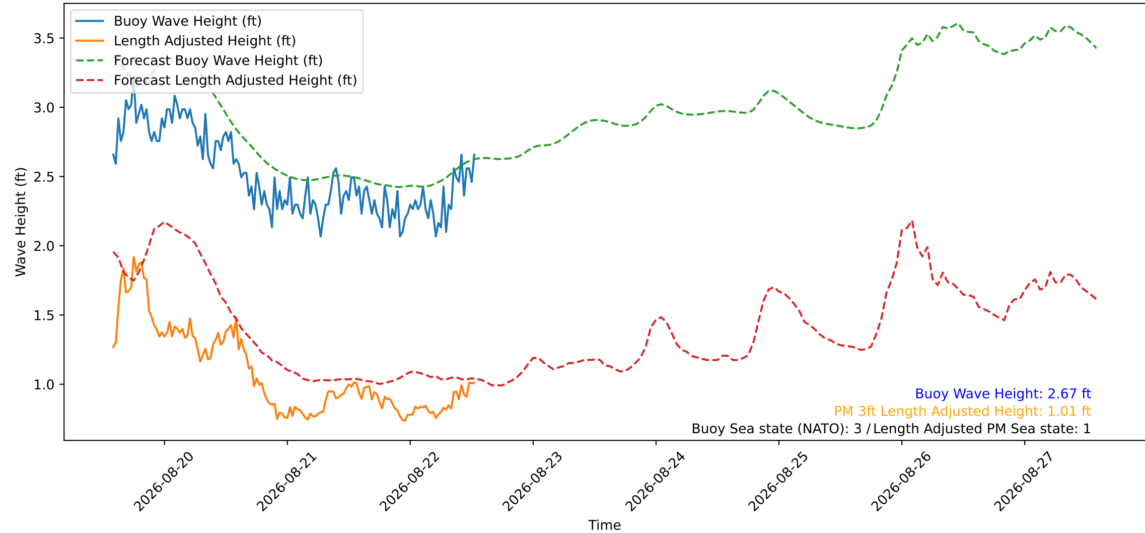
Wave Heights over Time for Red Beach at 2026-08-22 13:30:50
