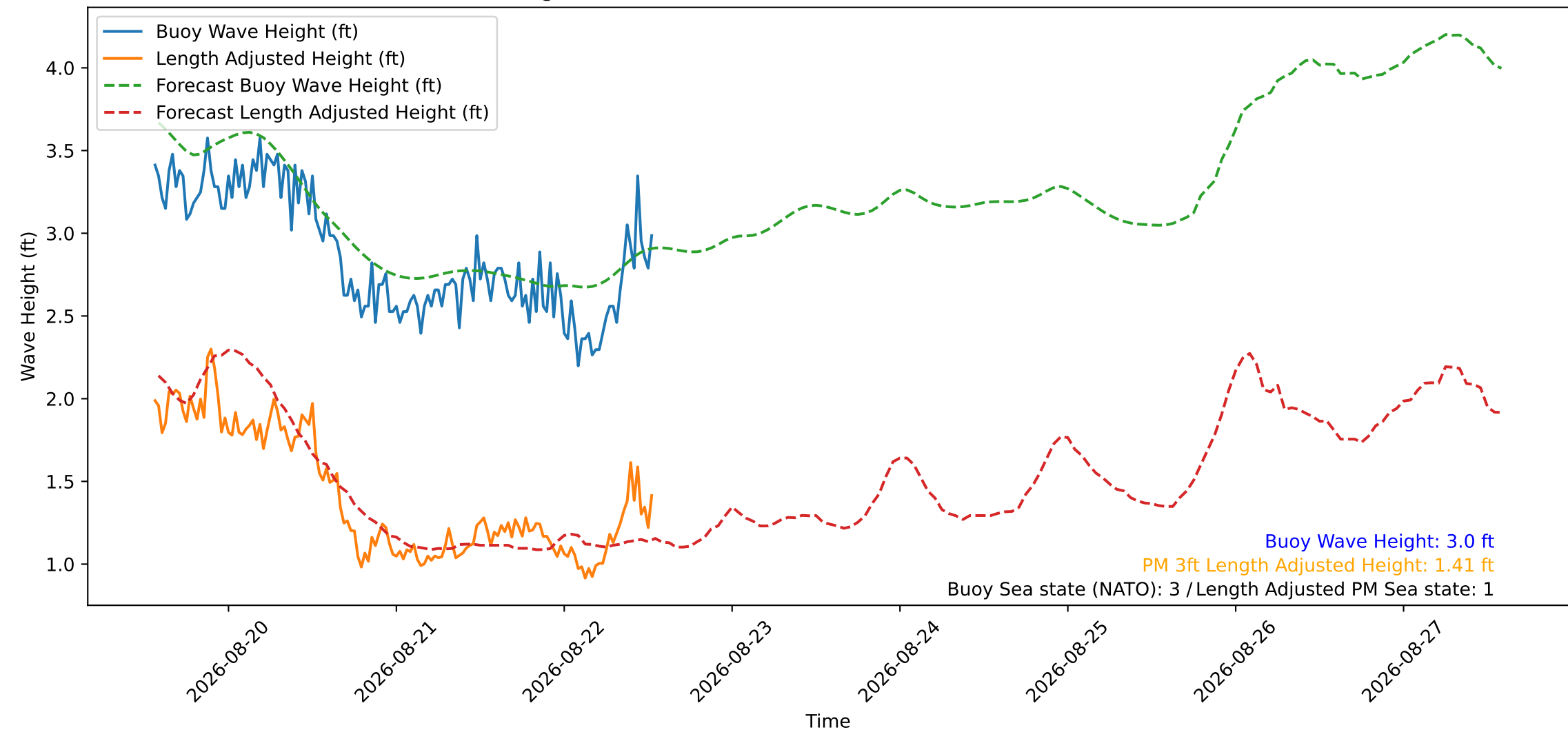
Wave Heights over Time for Oceanside Harbor at 2026-08-22 13:30:30
