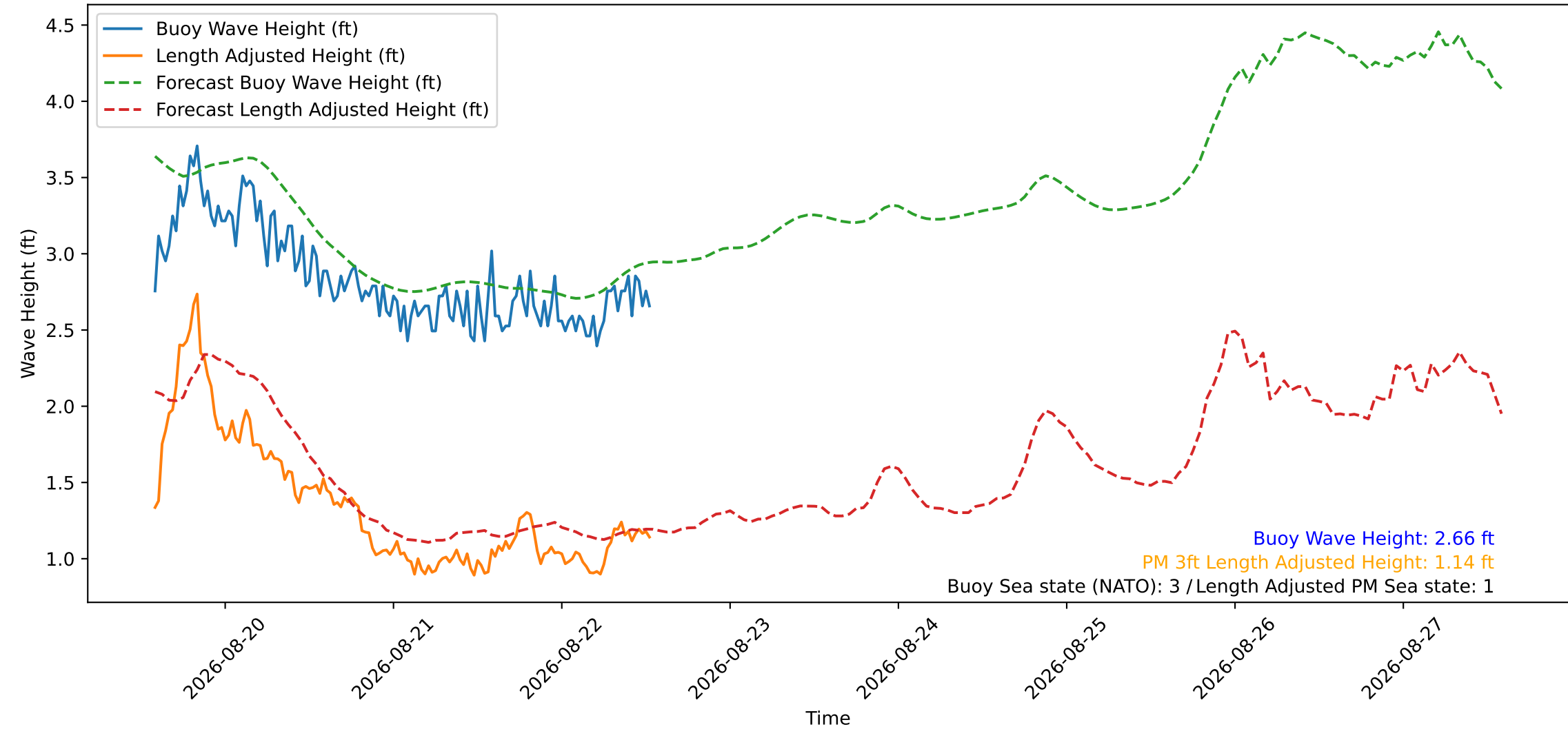
Wave Heights over Time for Green Beach at 2026-08-22 13:31:12
