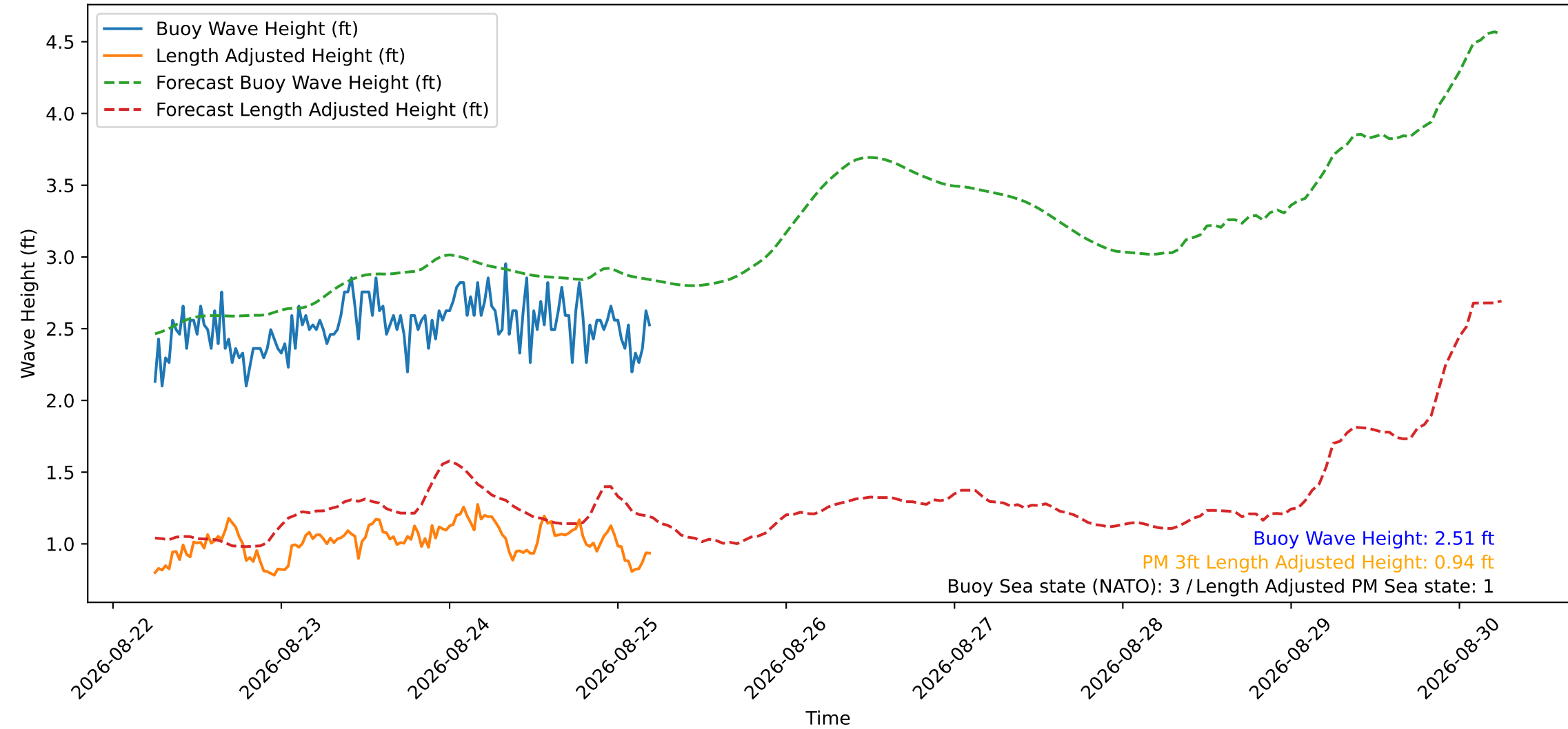
Wave Heights over Time for Red Beach at 2026-08-25 05:30:49
