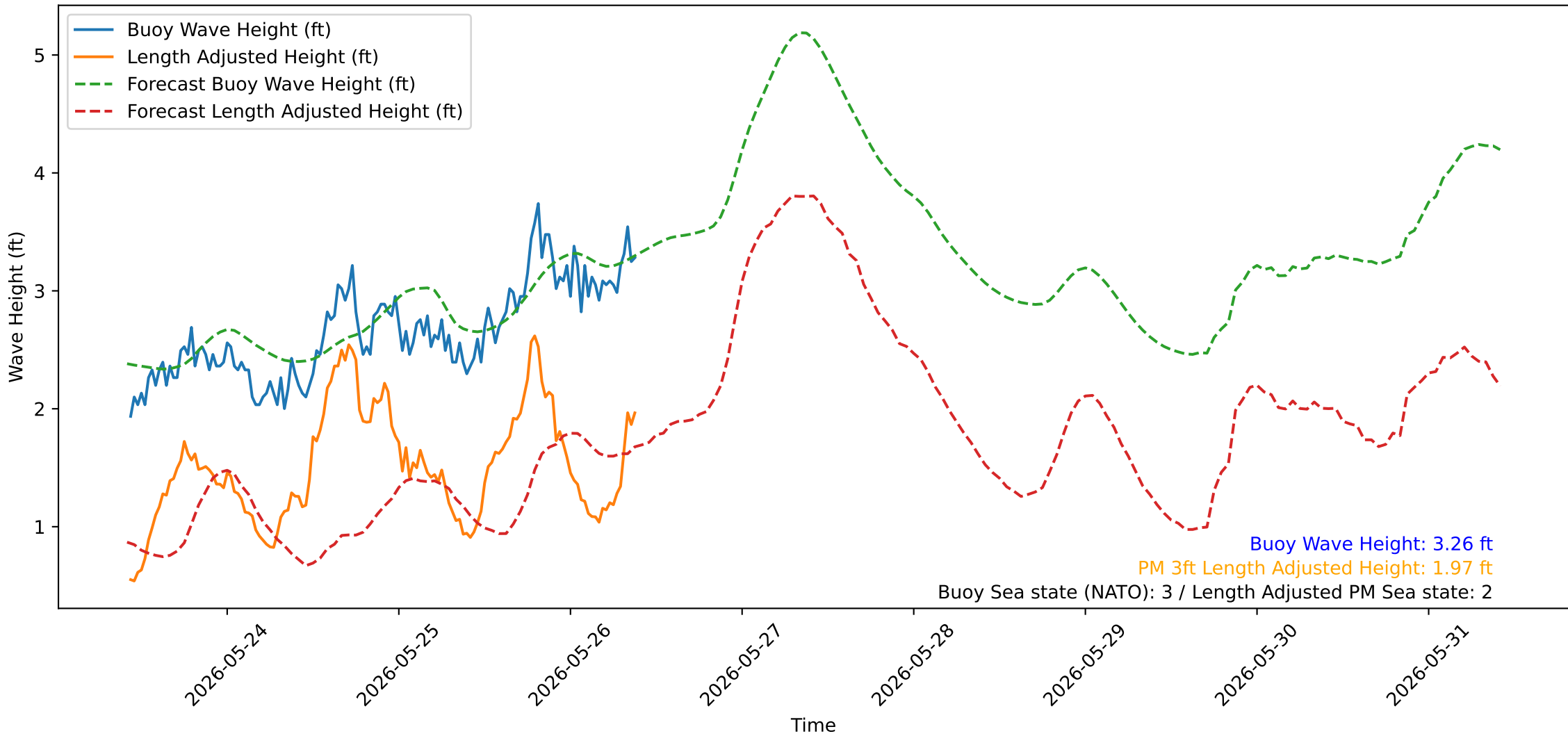
Wave Heights over Time for Red Beach at 2026-05-26 10:00:47
