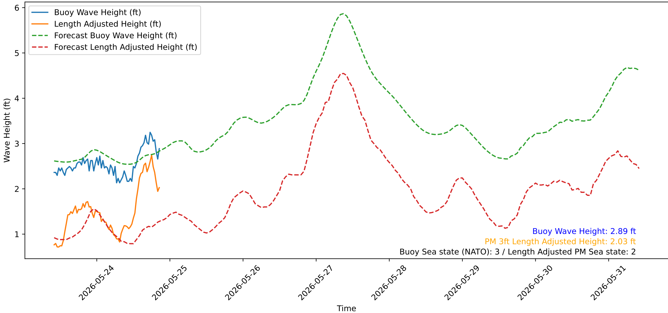
Wave Heights over Time for Oceanside Harbor at 2026-05-26 10:00:28
