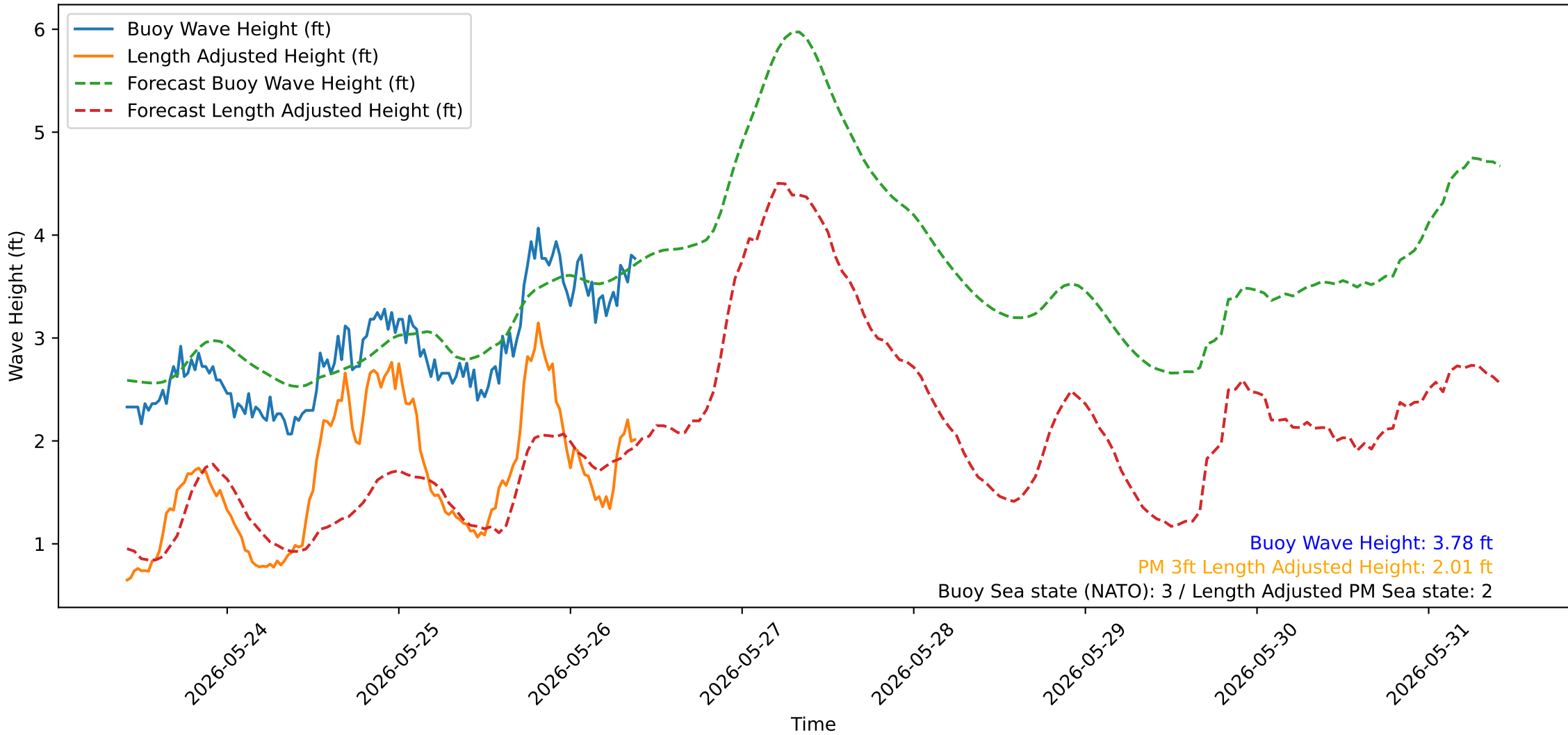
Wave Heights over Time for Green Beach at 2026-05-26 10:01:09
