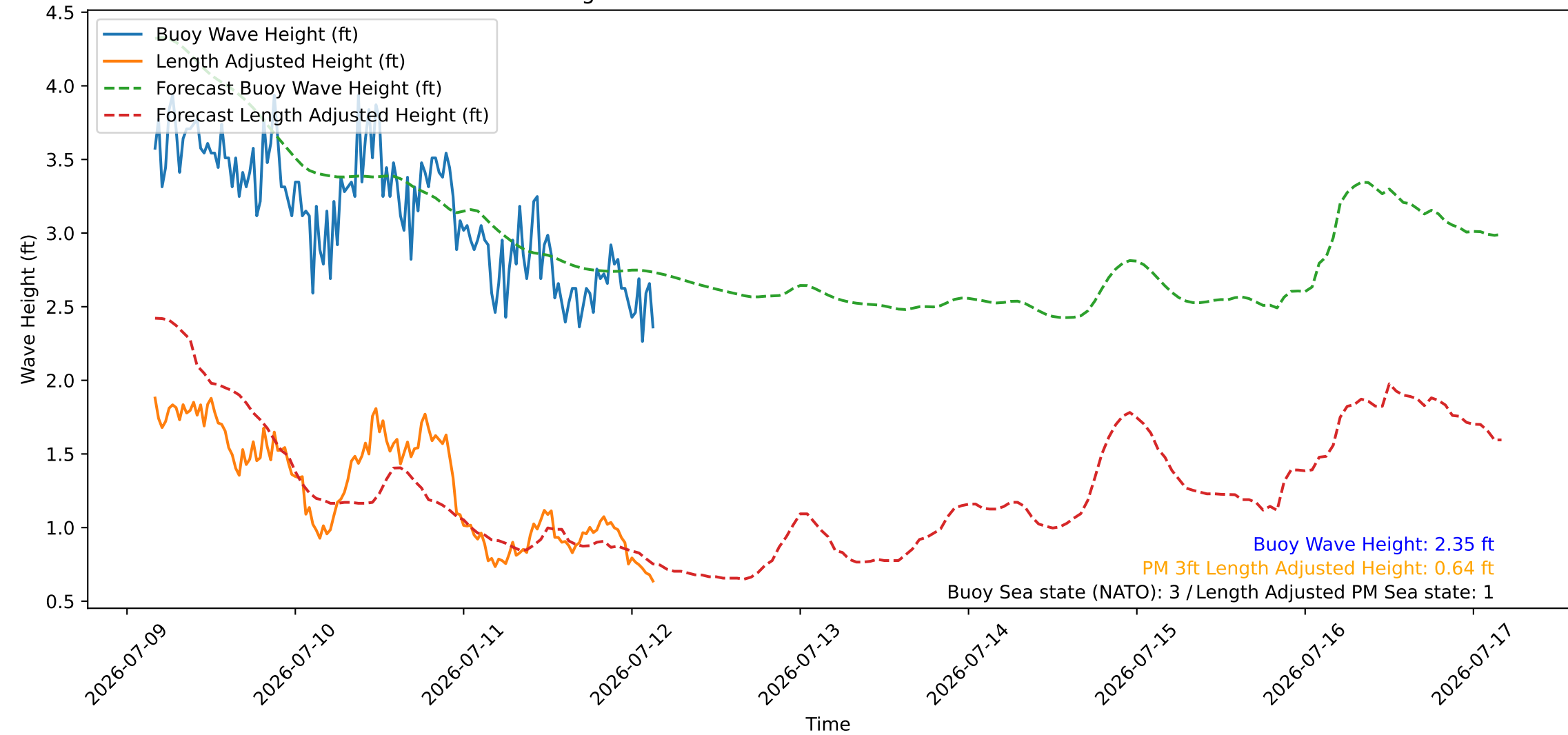
Wave Heights over Time for Red Beach at 2026-07-12 03:40:45
