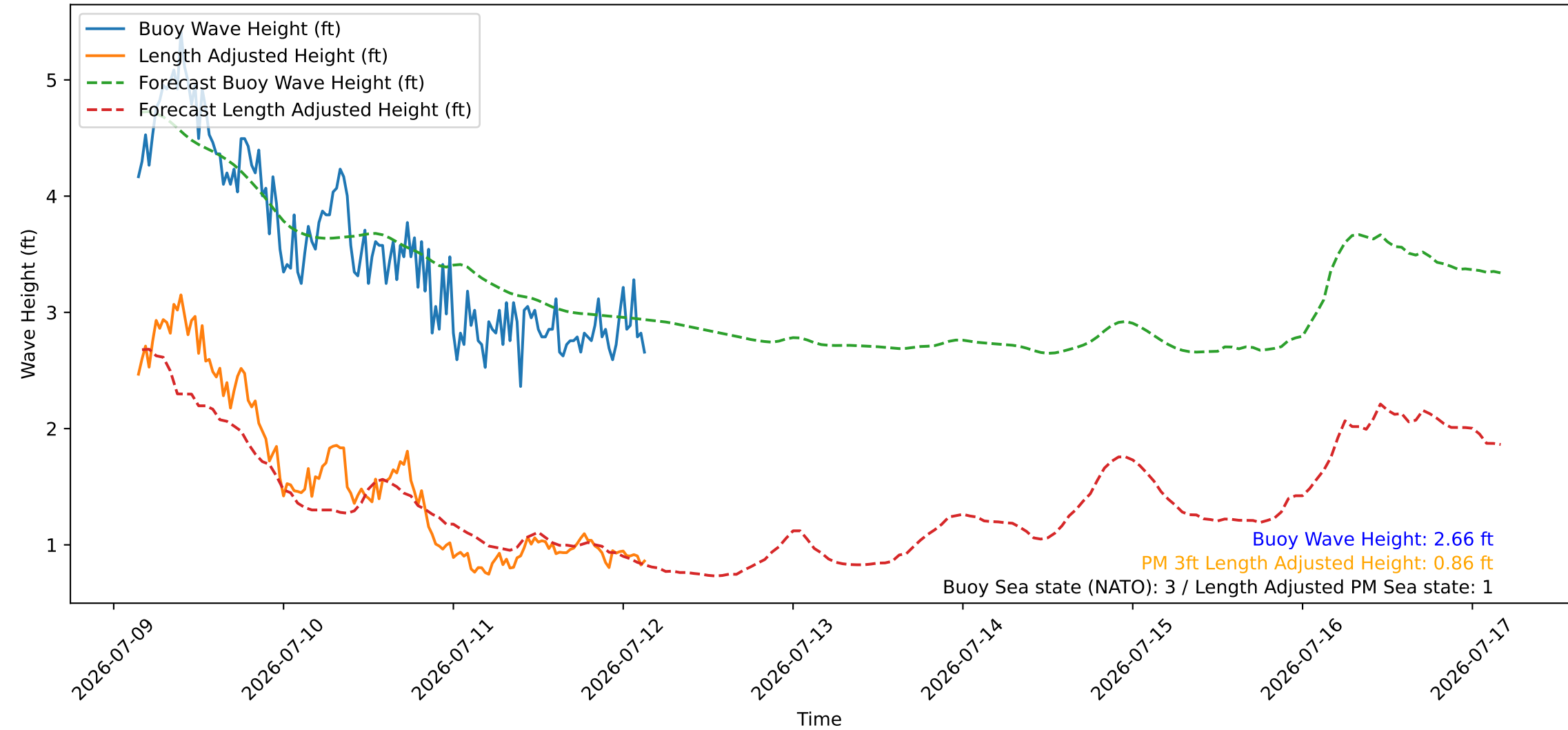
Wave Heights over Time for Oceanside Harbor at 2026-07-12 03:40:26
