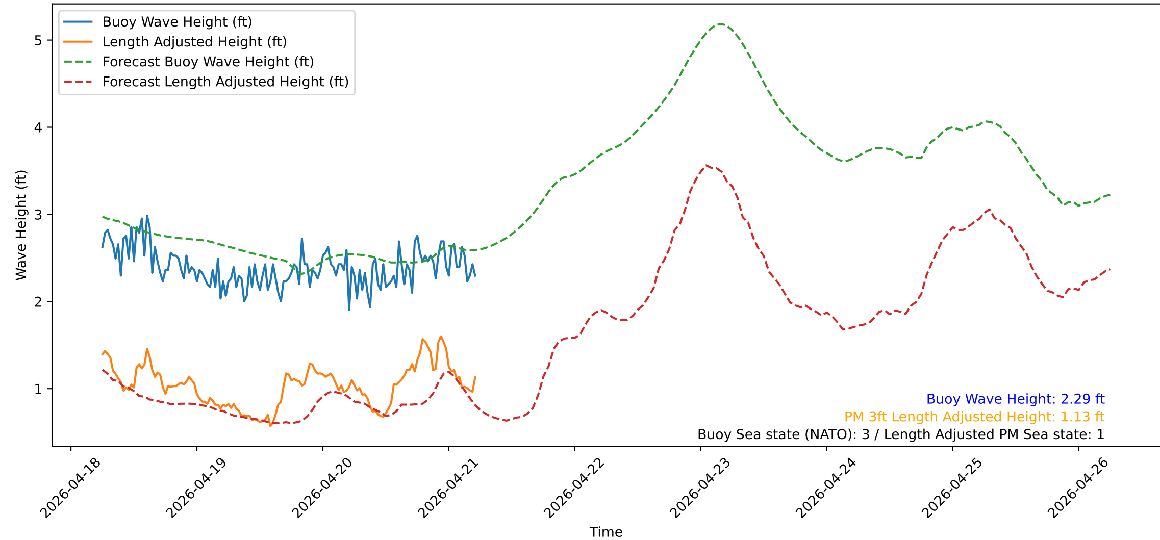
Wave Heights over Time for Oceanside Harbor at 2026-04-21 05:50:31
