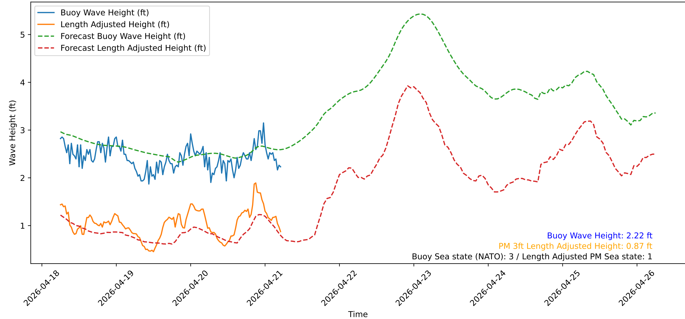
Wave Heights over Time for Green Beach at 2026-04-21 05:51:14
