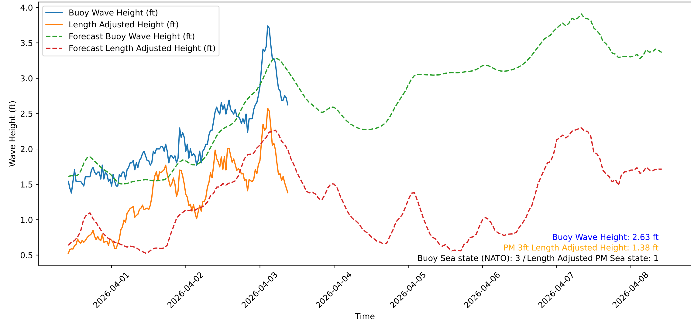
Wave Heights over Time for Red Beach at 2026-04-03 09:50:47
