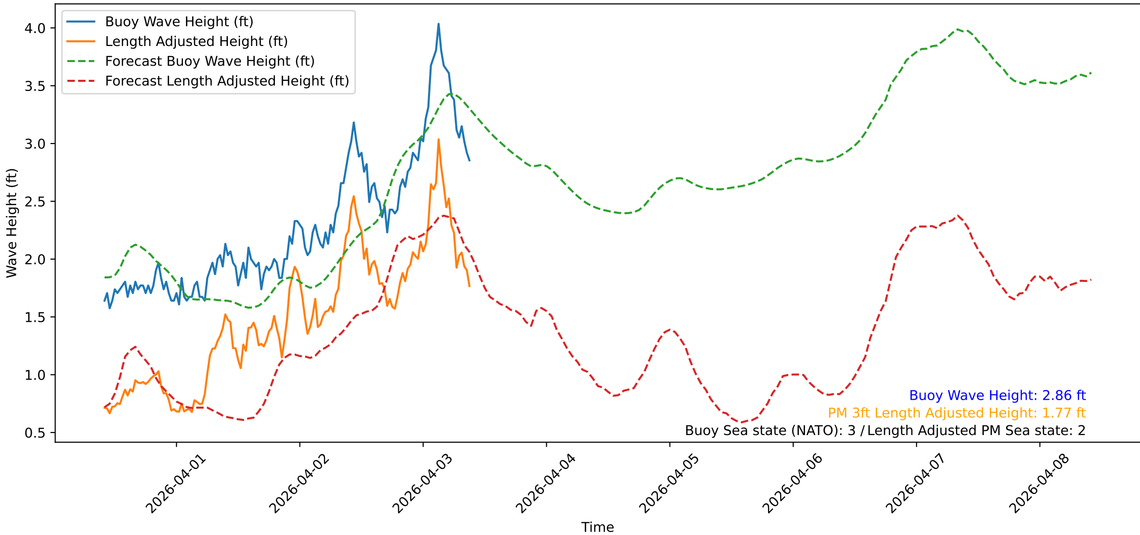
Wave Heights over Time for Oceanside Harbor at 2026-04-03 09:50:31
