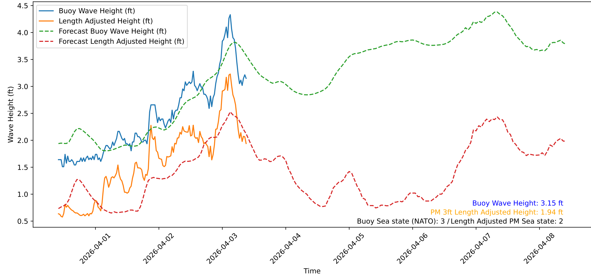
Wave Heights over Time for Green Beach at 2026-04-03 09:51:09
