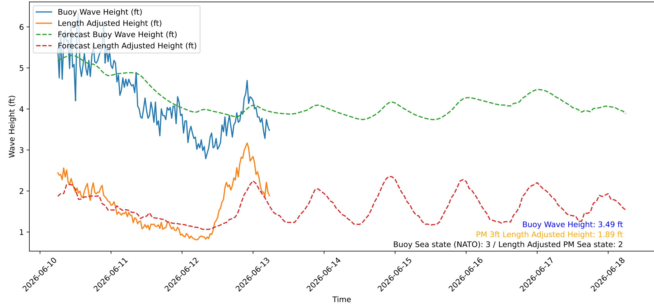
Wave Heights over Time for Oceanside Harbor at 2026-06-13 06:10:26
