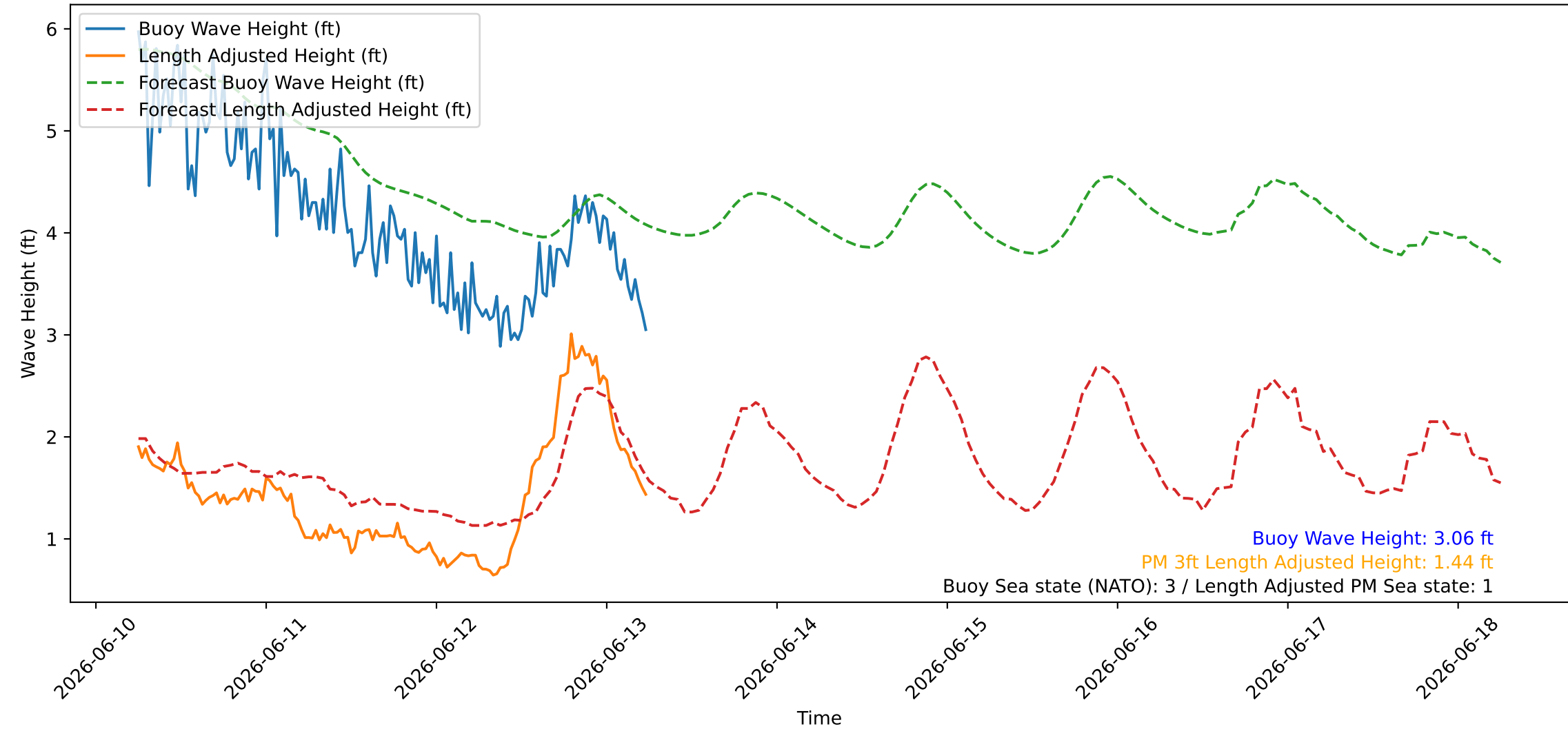
Wave Heights over Time for Green Beach at 2026-06-13 06:11:08
