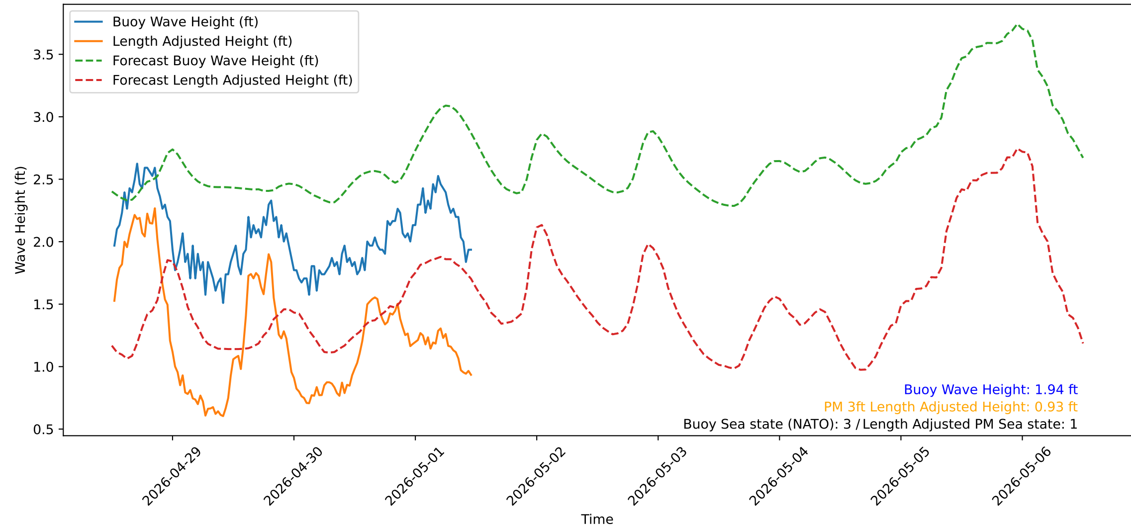
Wave Heights over Time for Red Beach at 2026-05-01 12:10:51
