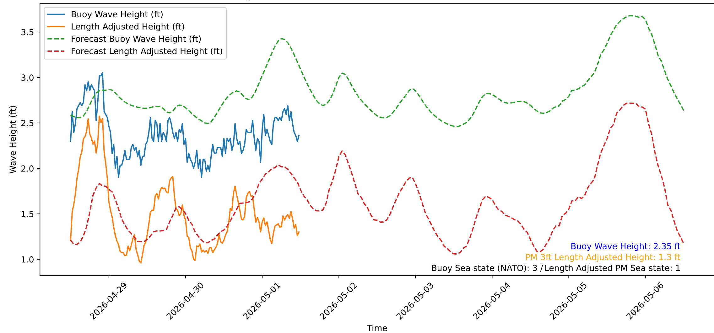
Wave Heights over Time for Oceanside Harbor at 2026-05-01 12:10:32
