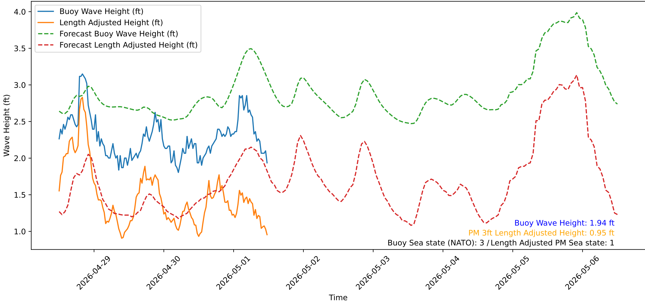
Wave Heights over Time for Green Beach at 2026-05-01 12:11:13
