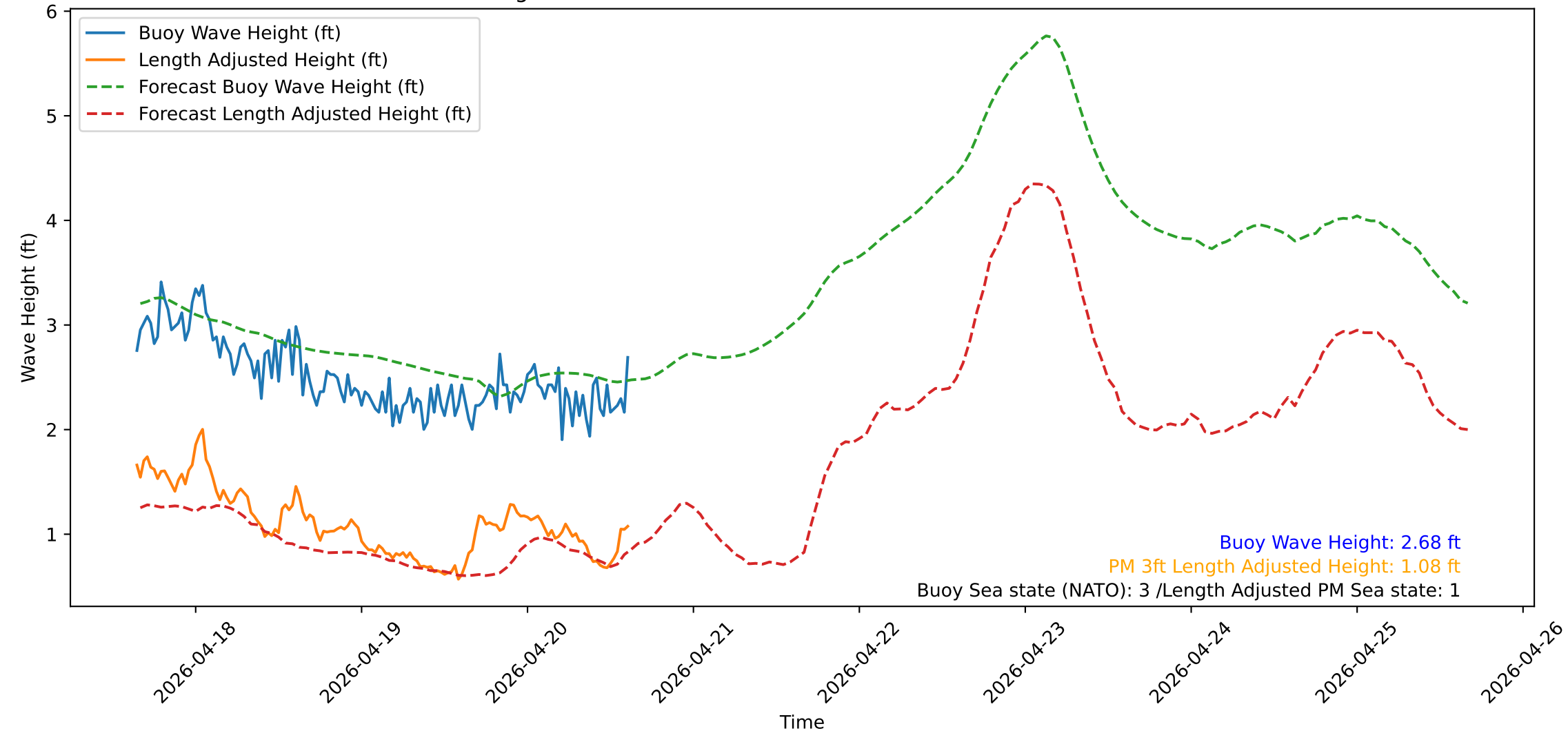
Wave Heights over Time for Oceanside Harbor at 2026-04-20 15:30:32
