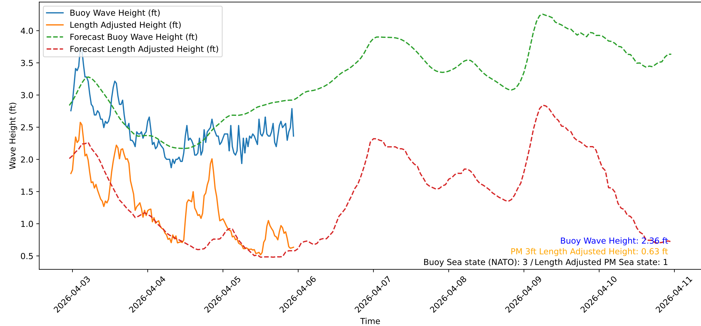
Wave Heights over Time for Red Beach at 2026-04-05 23:20:49
