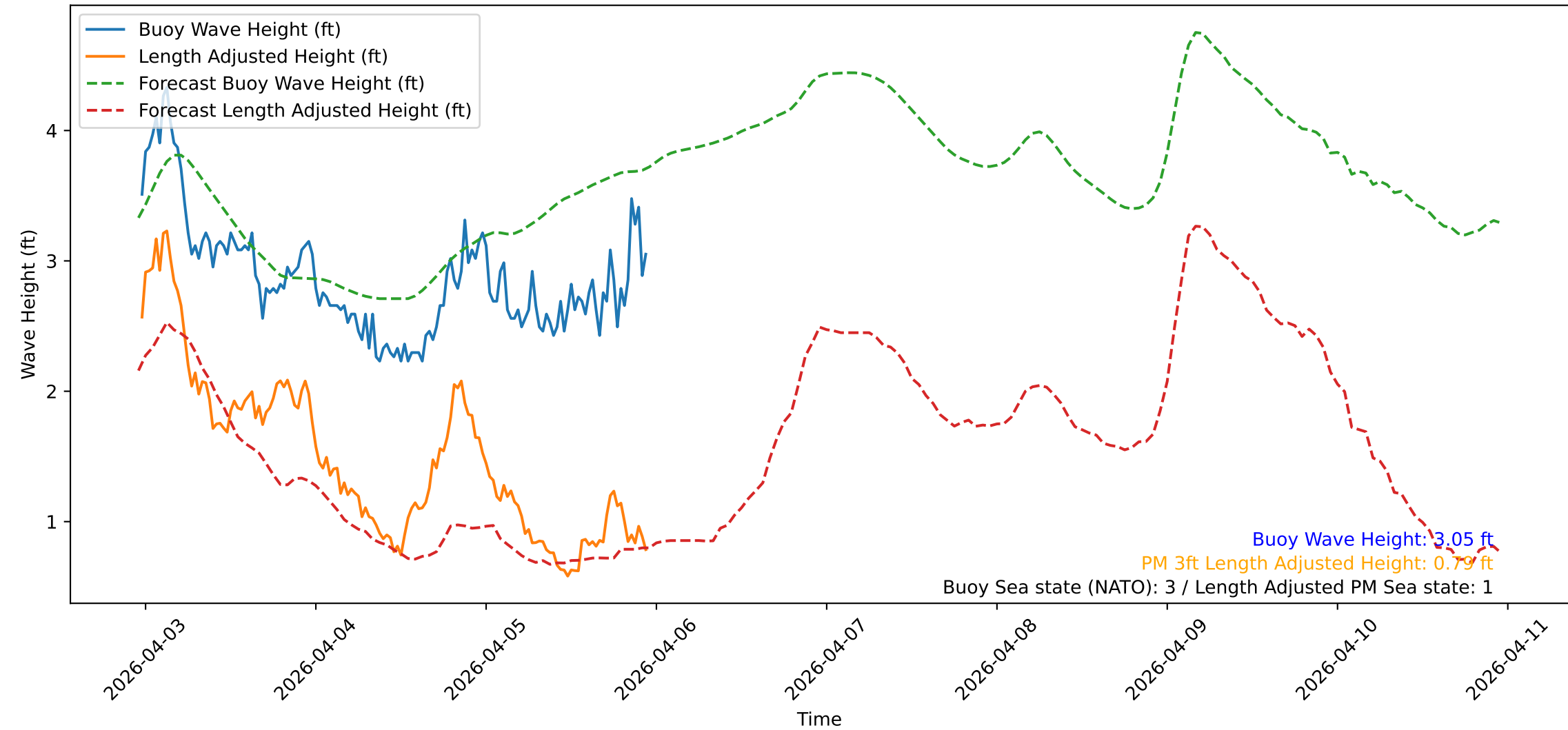
Wave Heights over Time for Green Beach at 2026-04-05 23:21:13
