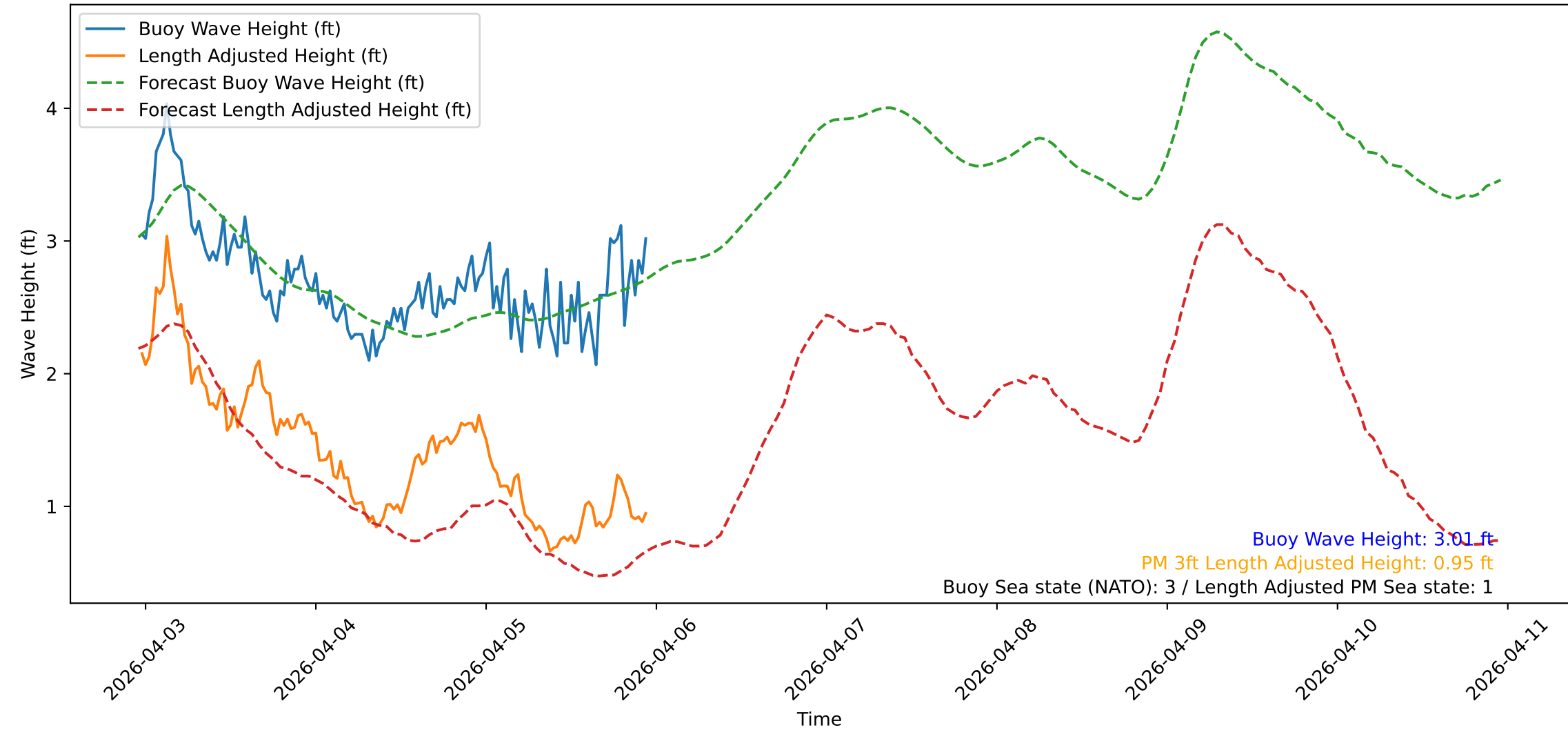
Wave Heights over Time for Oceanside Harbor at 2026-04-05 23:20:33
