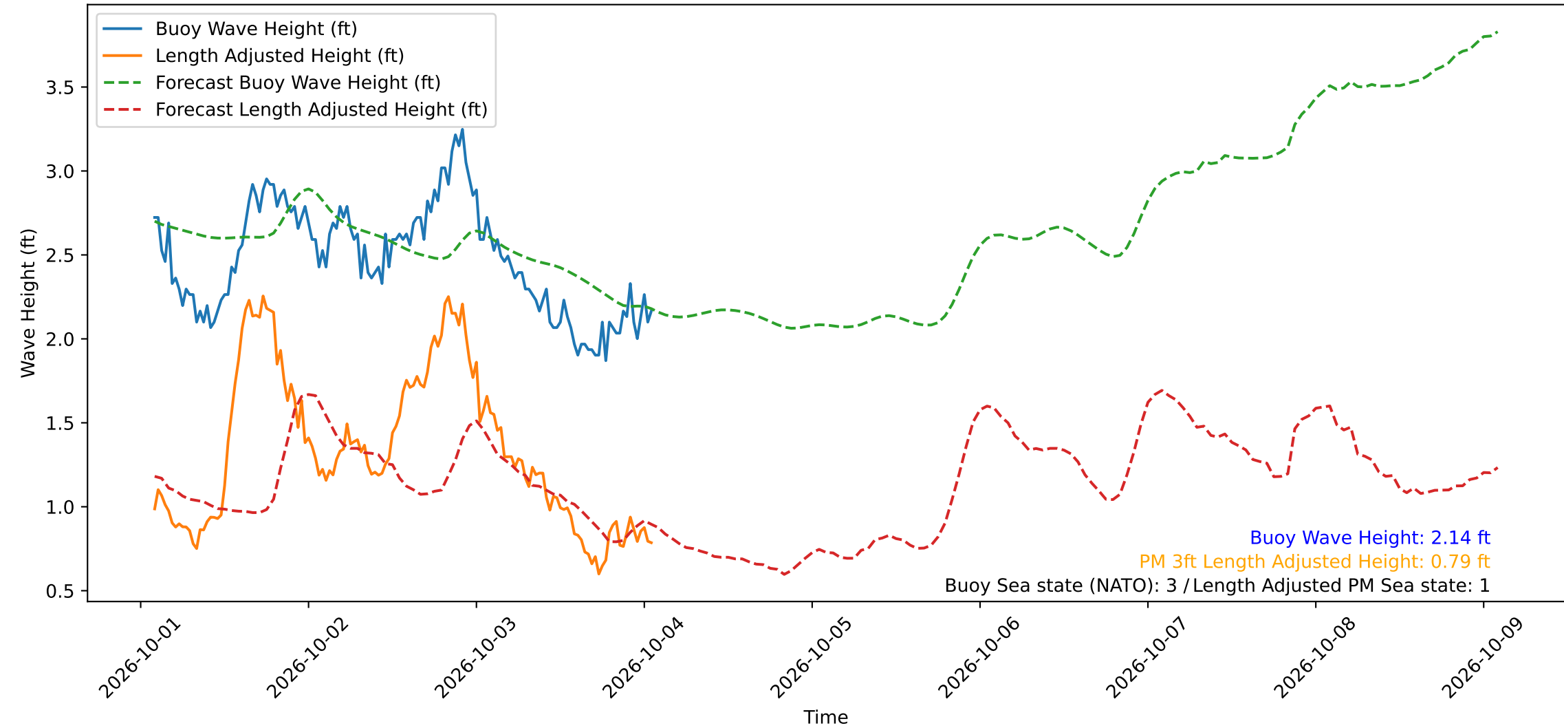
Wave Heights over Time for Red Beach at 2026-10-04 01:40:49
