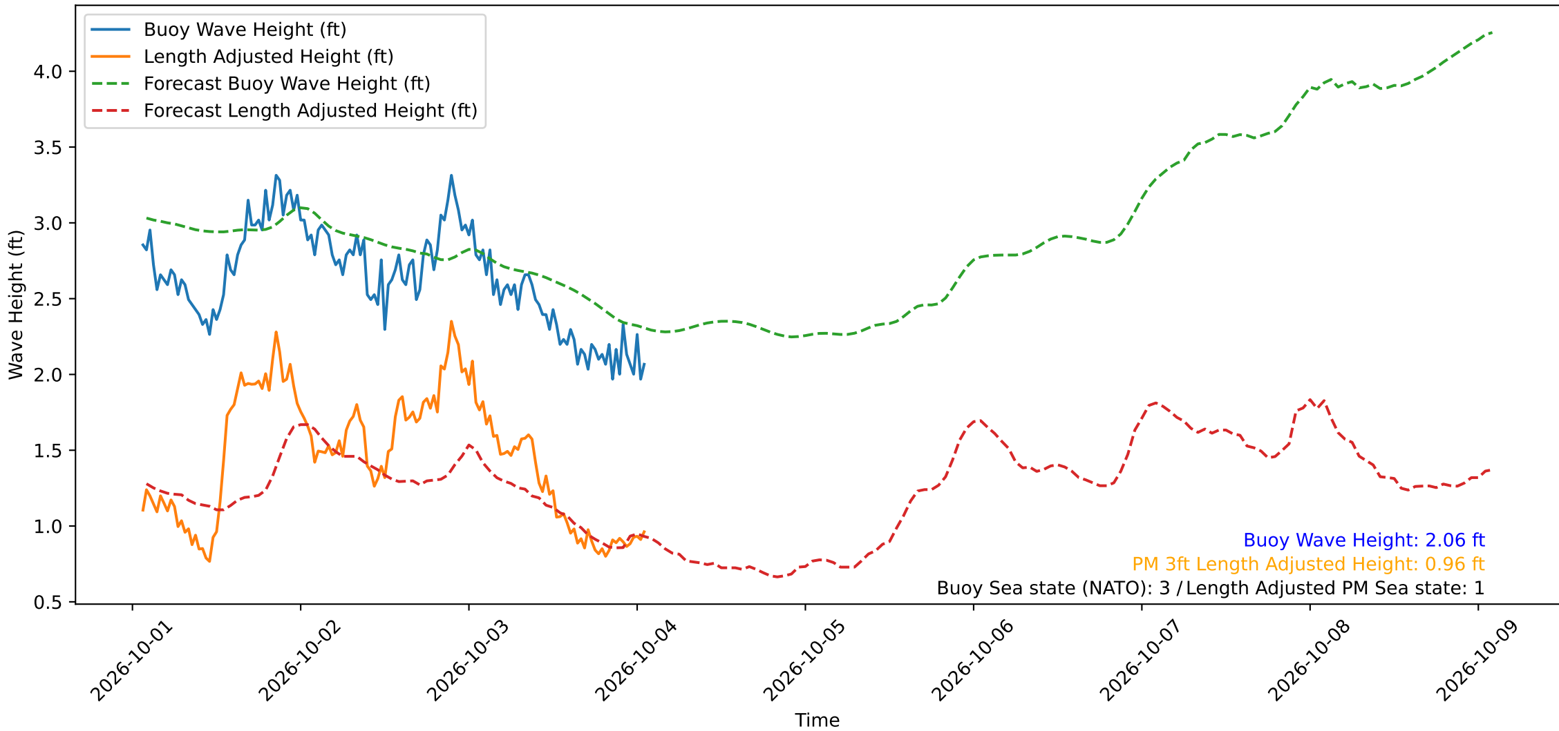
Wave Heights over Time for Oceanside Harbor at 2026-10-04 01:40:30
