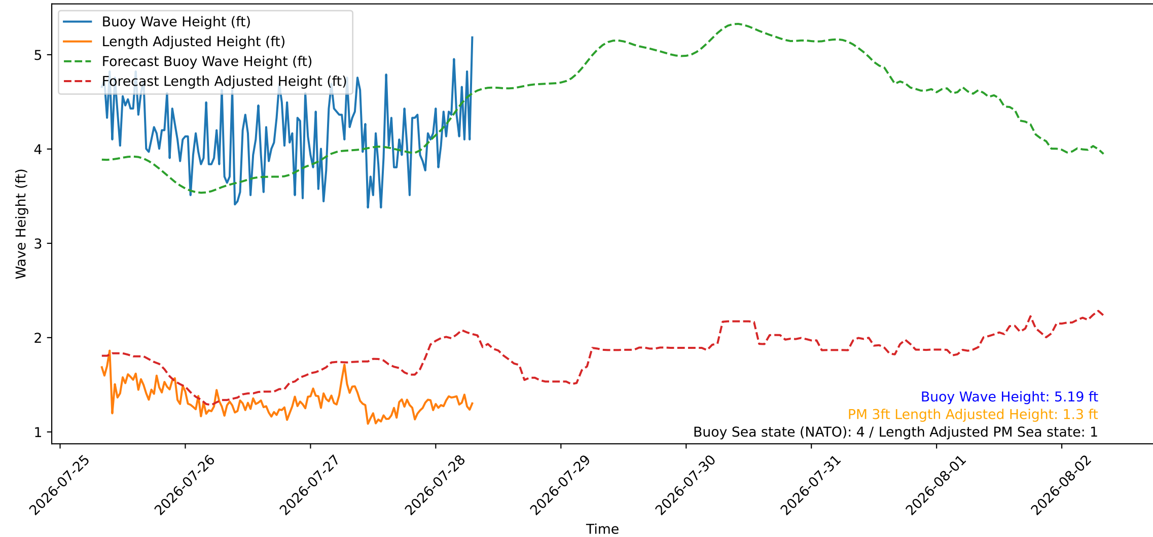
Wave Heights over Time for Green Beach at 2026-07-28 07:51:09
