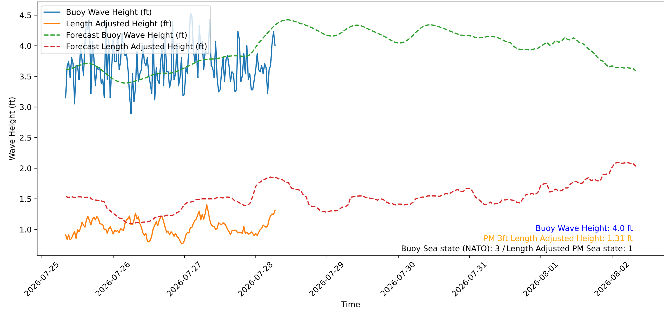
Wave Heights over Time for Red Beach at 2026-07-28 07:50:47
