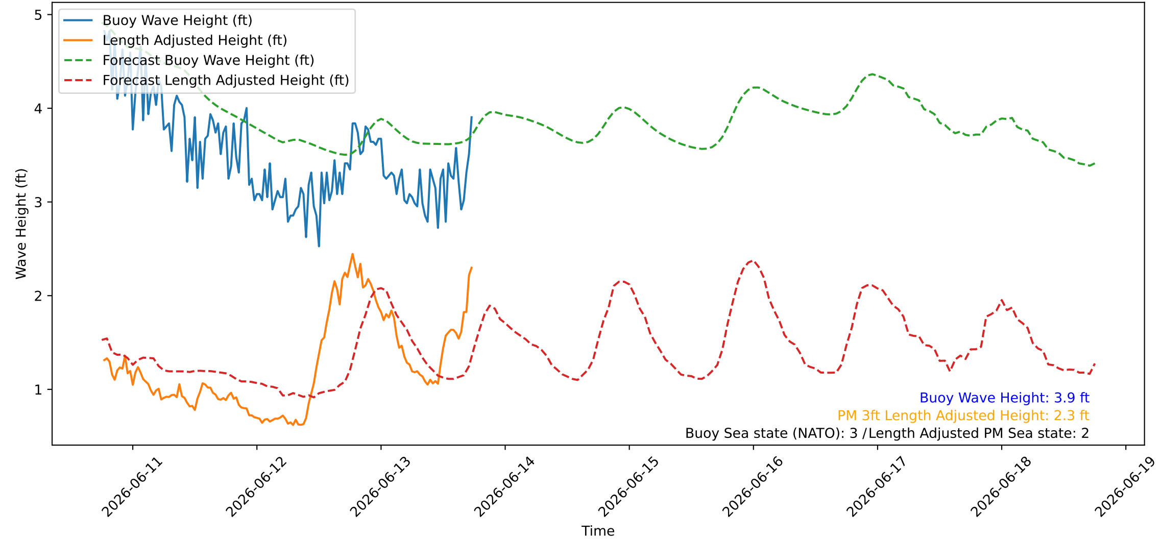
Wave Heights over Time for Red Beach at 2026-06-13 18:10:45
