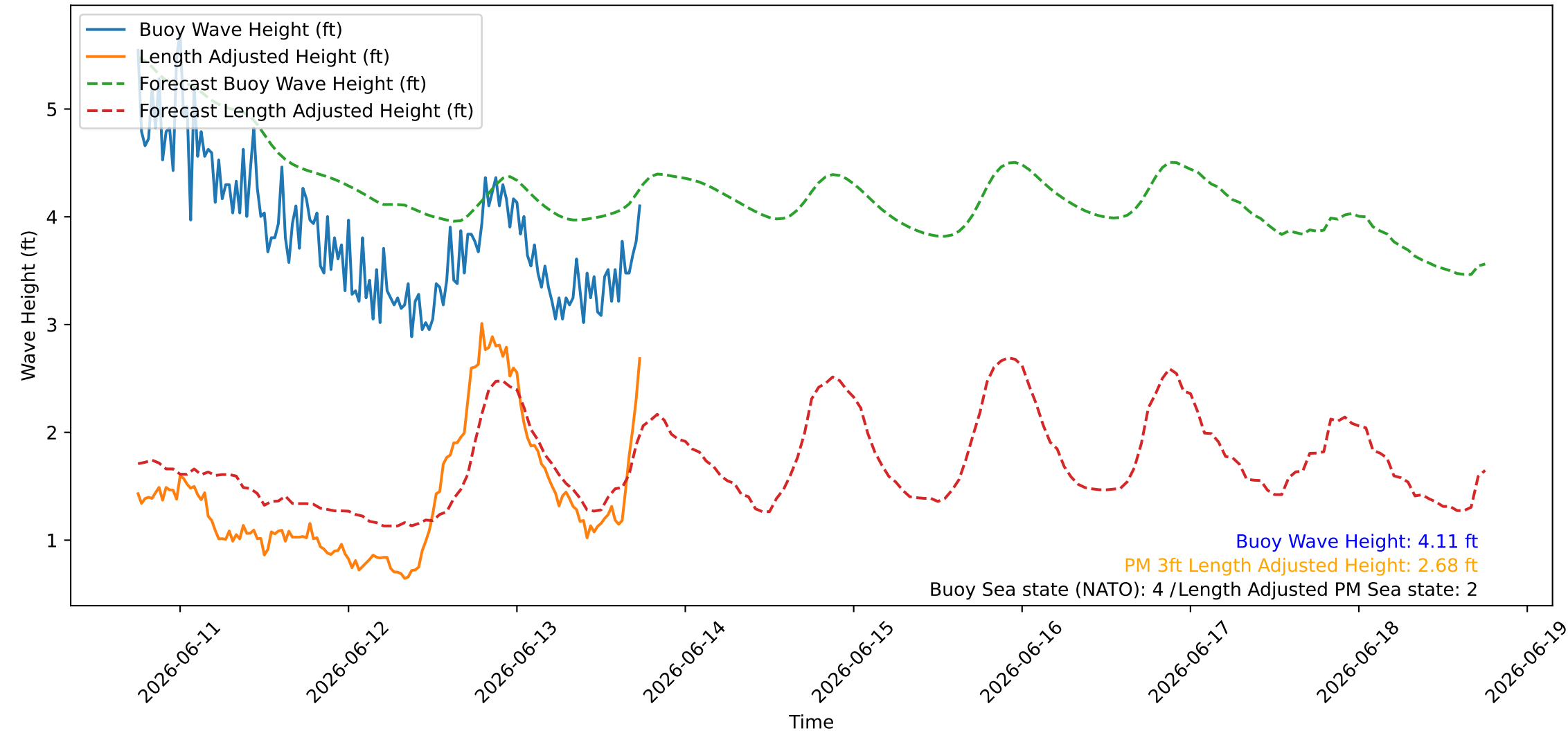
Wave Heights over Time for Green Beach at 2026-06-13 18:11:08
