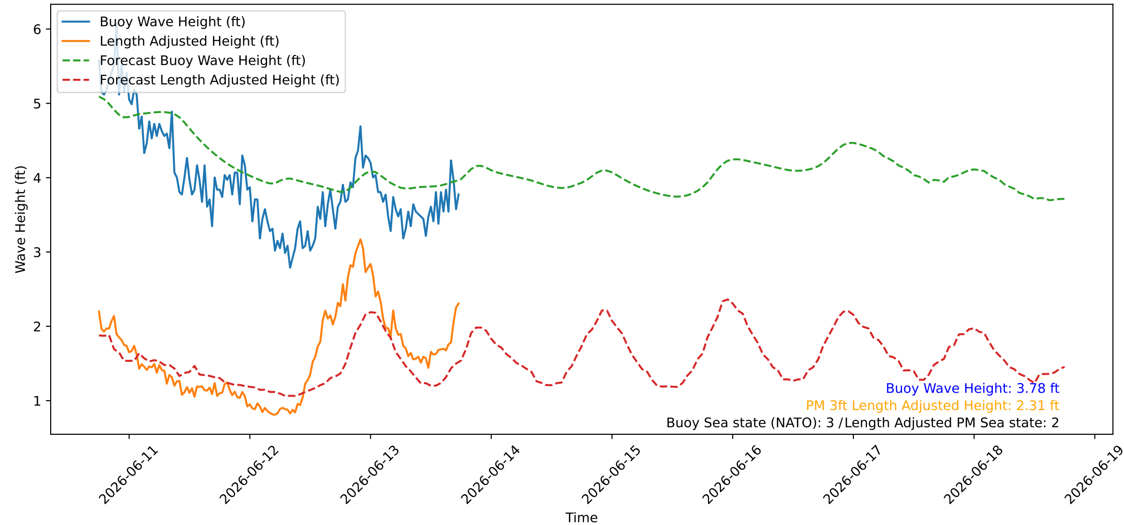
Wave Heights over Time for Oceanside Harbor at 2026-06-13 18:10:26
