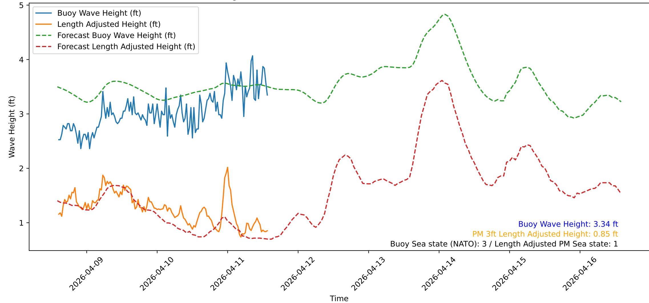
Wave Heights over Time for Green Beach at 2026-04-11 14:21:14
