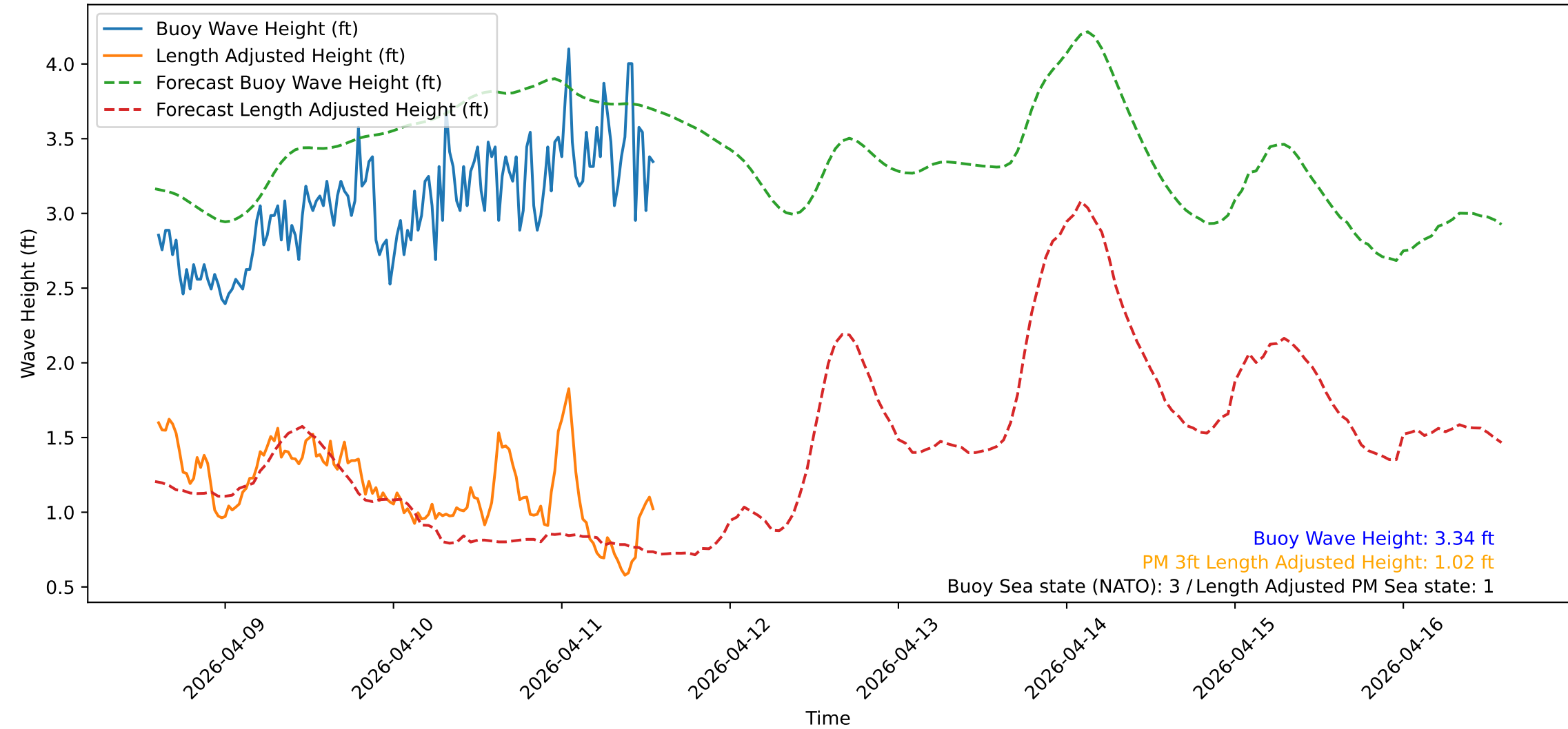
Wave Heights over Time for Red Beach at 2026-04-11 14:20:51
