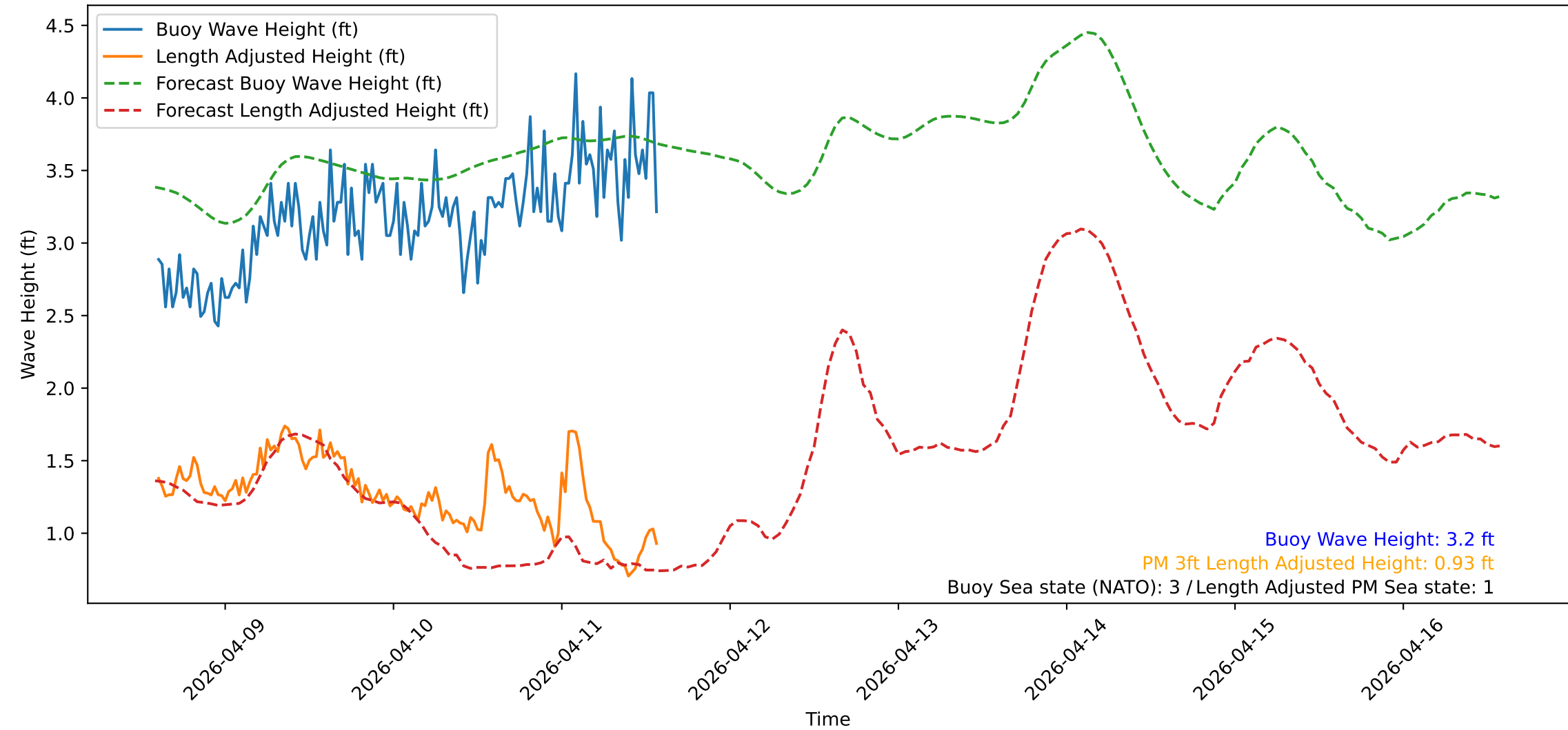
Wave Heights over Time for Oceanside Harbor at 2026-04-11 14:20:31
