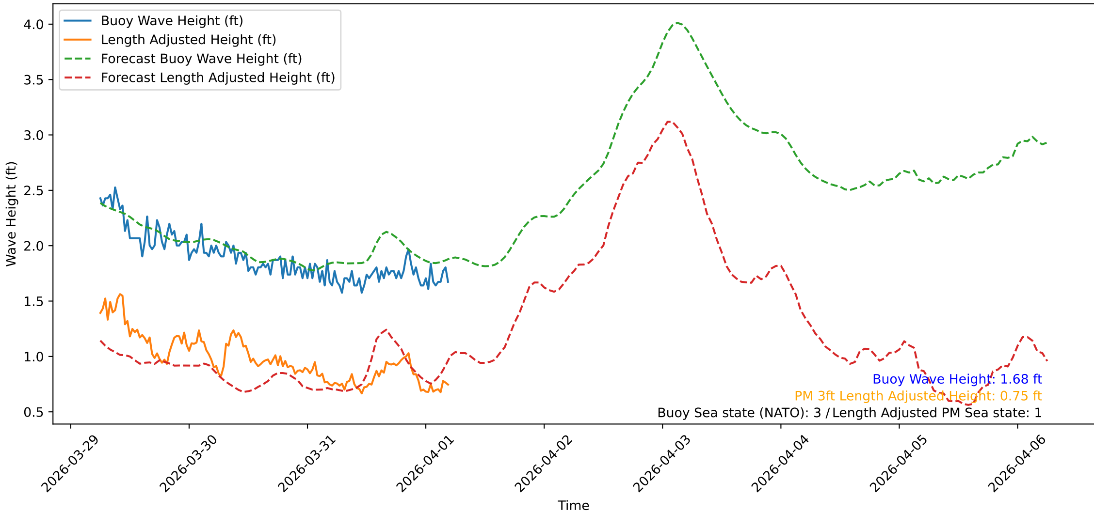
Wave Heights over Time for Oceanside Harbor at 2026-04-01 05:50:32
