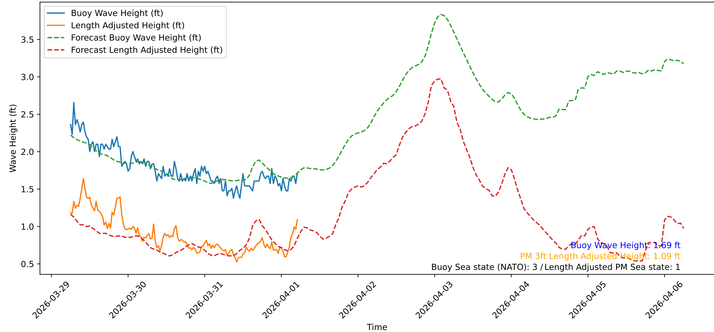
Wave Heights over Time for Red Beach at 2026-04-01 05:50:48
