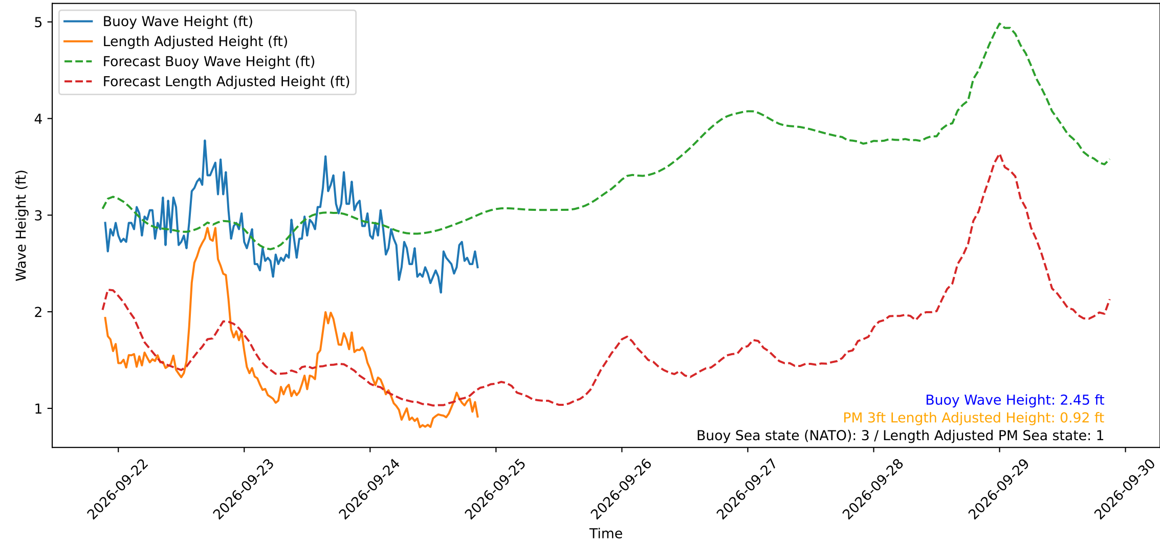
Wave Heights over Time for Oceanside Harbor at 2026-09-24 21:20:29
