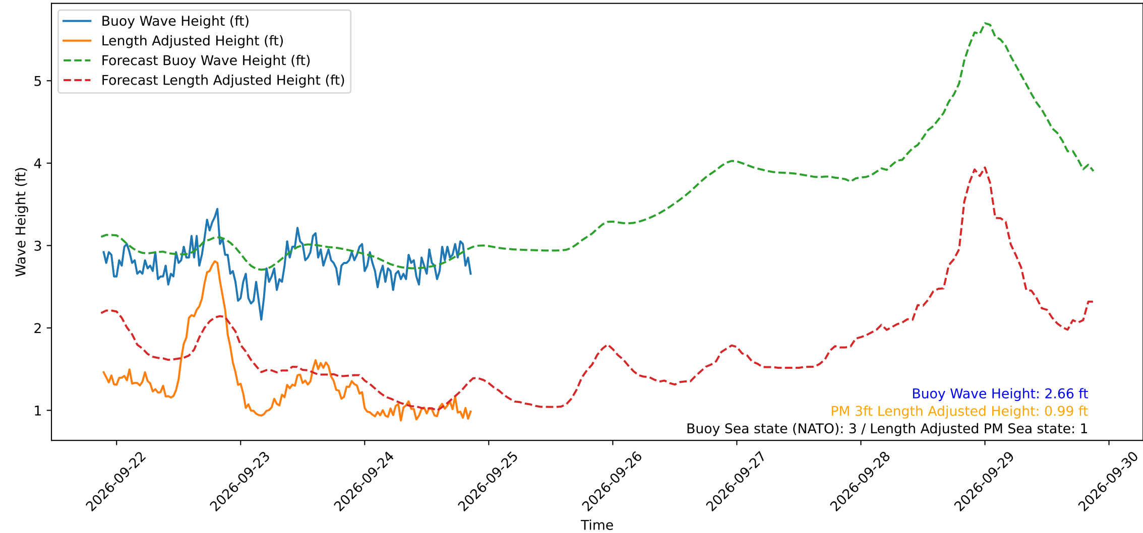
Wave Heights over Time for Green Beach at 2026-09-24 21:21:14
