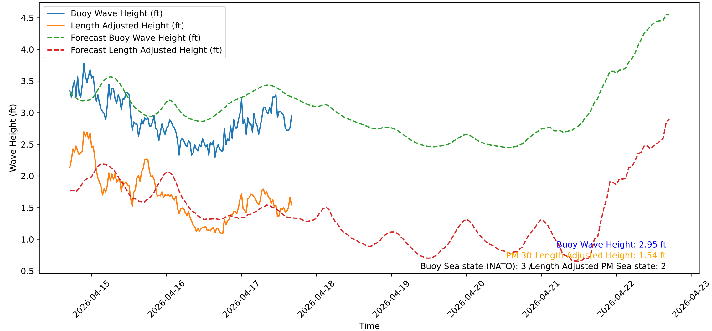
Wave Heights over Time for Oceanside Harbor at 2026-04-17 16:50:31
