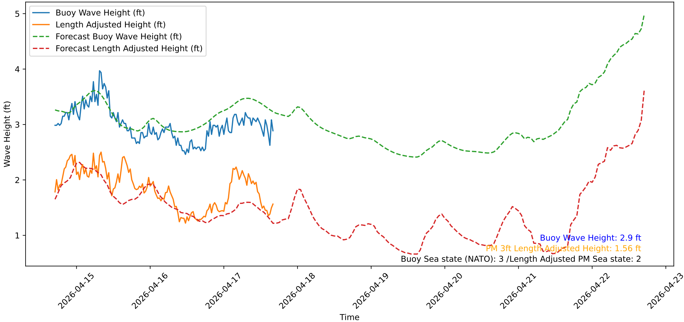
Wave Heights over Time for Green Beach at 2026-04-17 16:51:14
