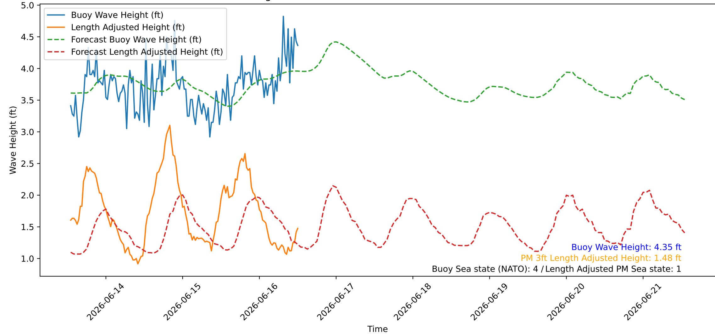
Wave Heights over Time for Red Beach at 2026-06-16 12:40:45
