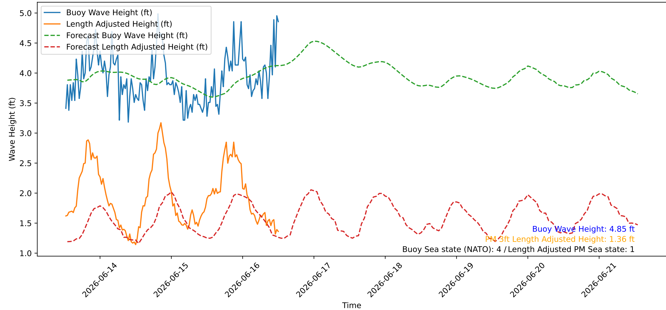
Wave Heights over Time for Oceanside Harbor at 2026-06-16 12:40:26
