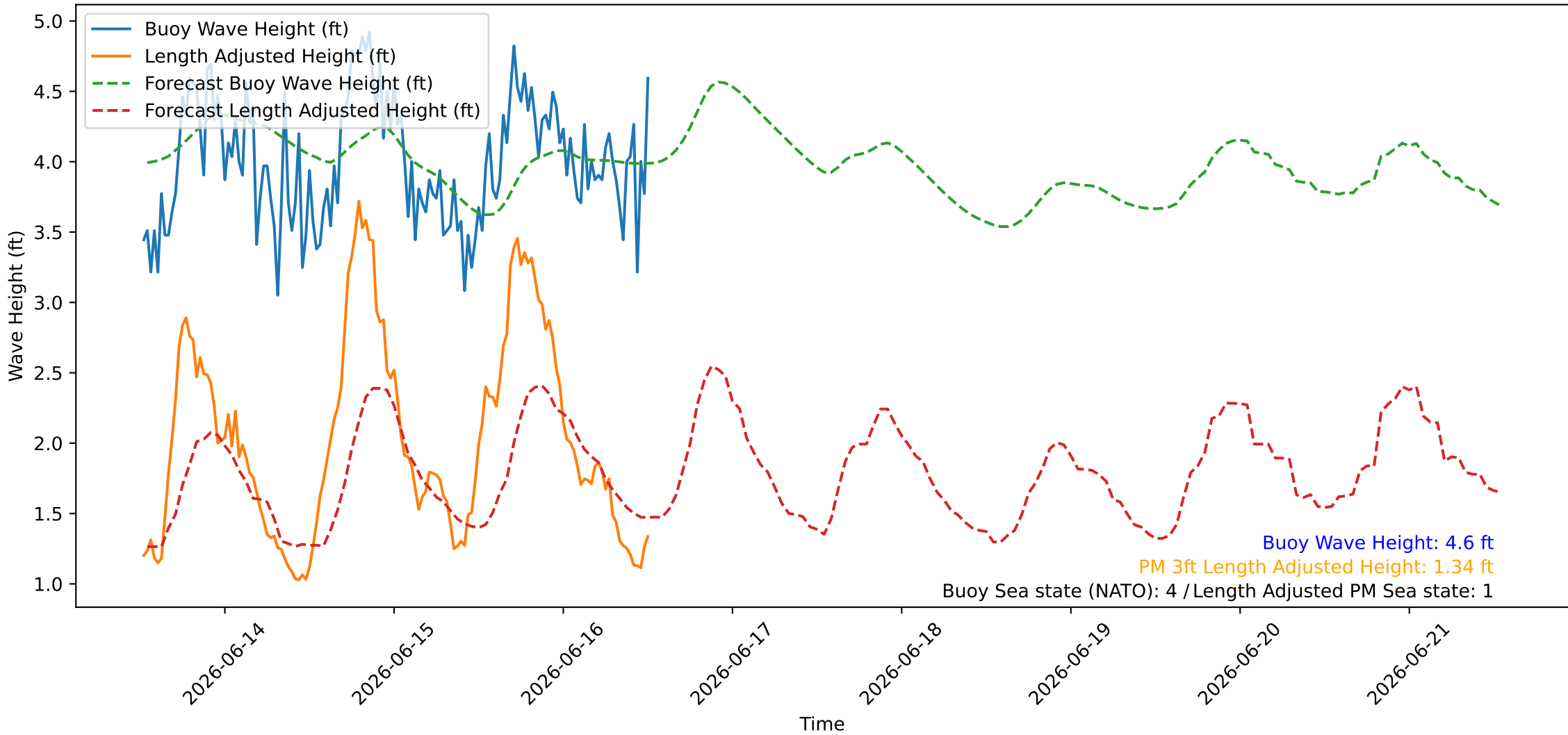
Wave Heights over Time for Green Beach at 2026-06-16 12:41:08
