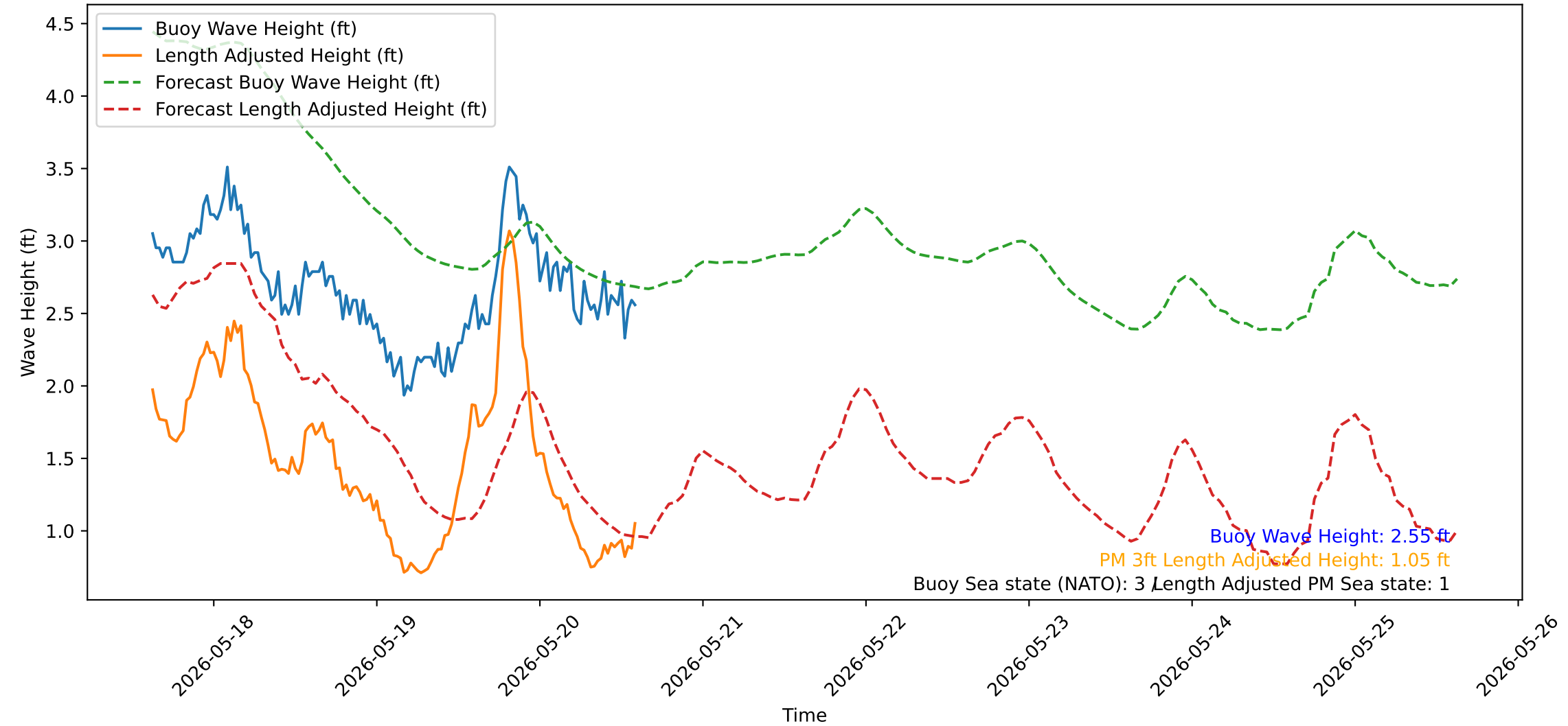
Wave Heights over Time for Red Beach at 2026-05-20 14:40:51
