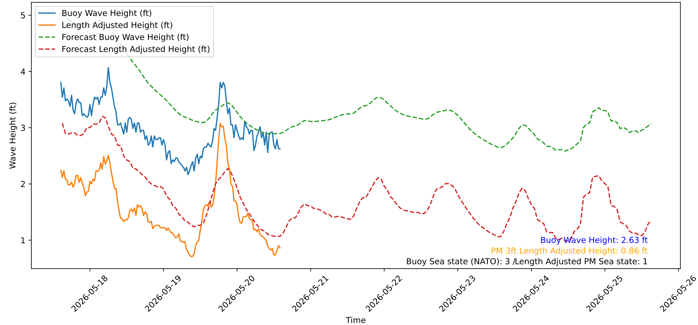
Wave Heights over Time for Green Beach at 2026-05-20 14:41:14
