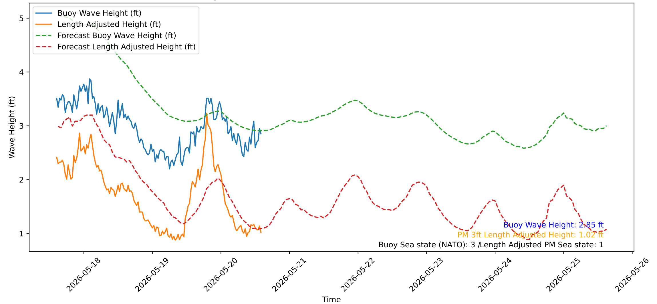
Wave Heights over Time for Oceanside Harbor at 2026-05-20 14:40:31
