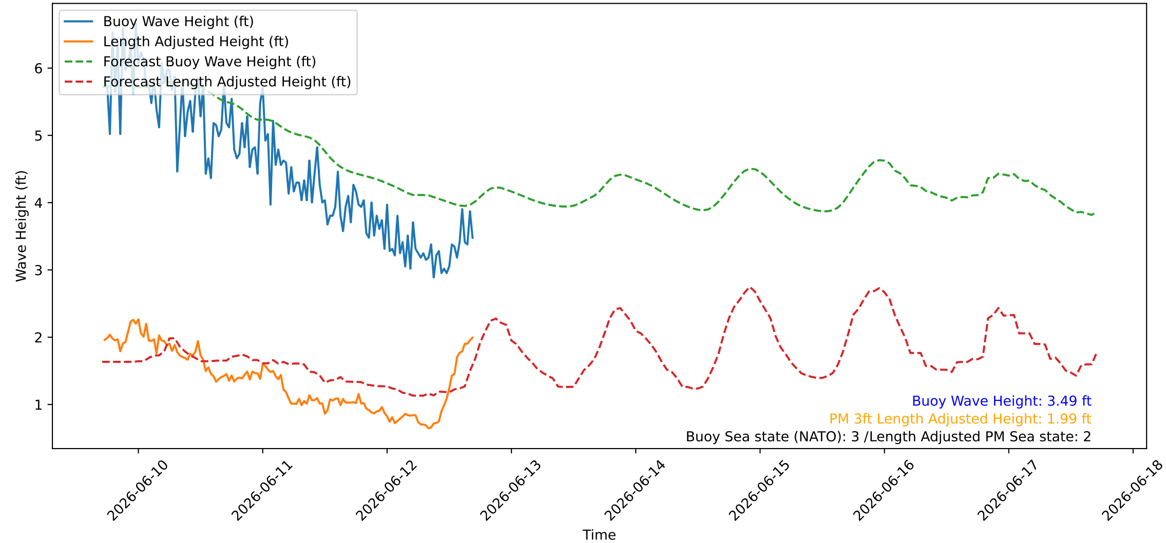
Wave Heights over Time for Green Beach at 2026-06-12 17:21:09
