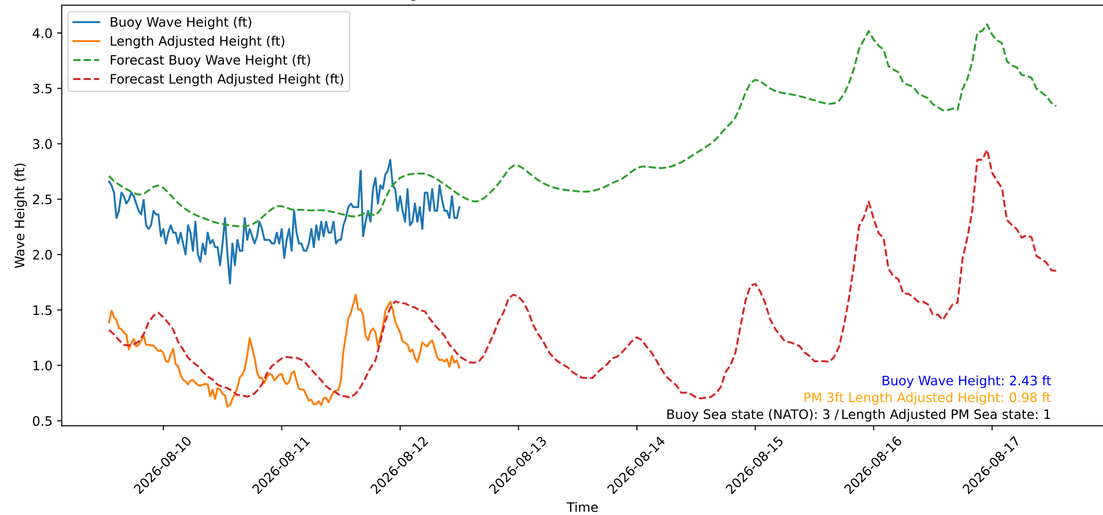
Wave Heights over Time for Red Beach at 2026-08-12 12:40:46
