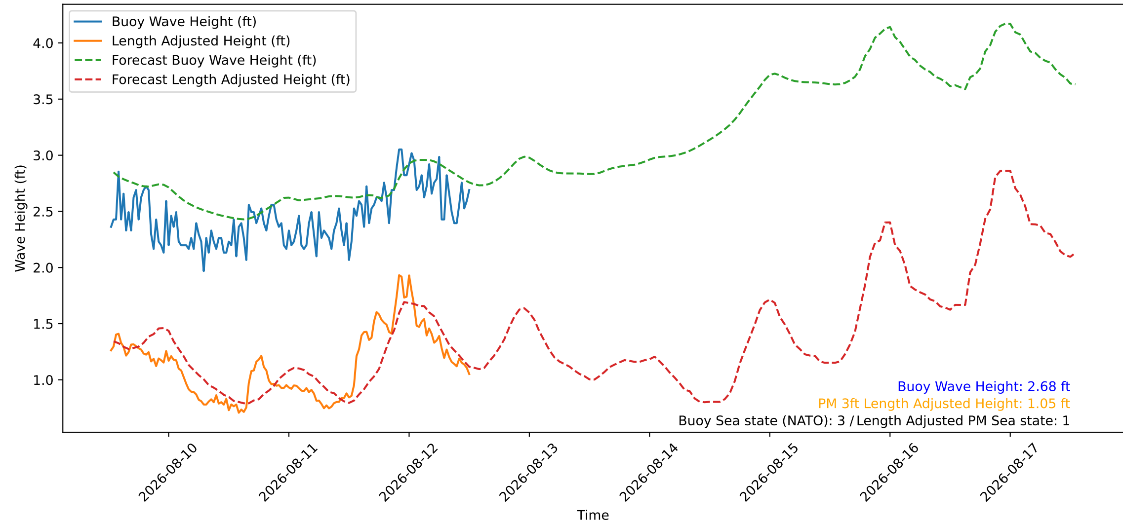
Wave Heights over Time for Oceanside Harbor at 2026-08-12 12:40:26
